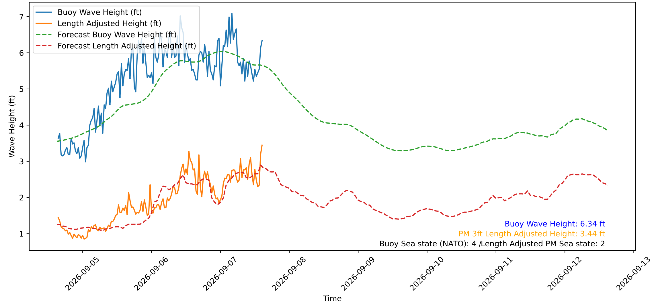
Wave Heights over Time for Oceanside Harbor at 2026-09-07 15:20:30
