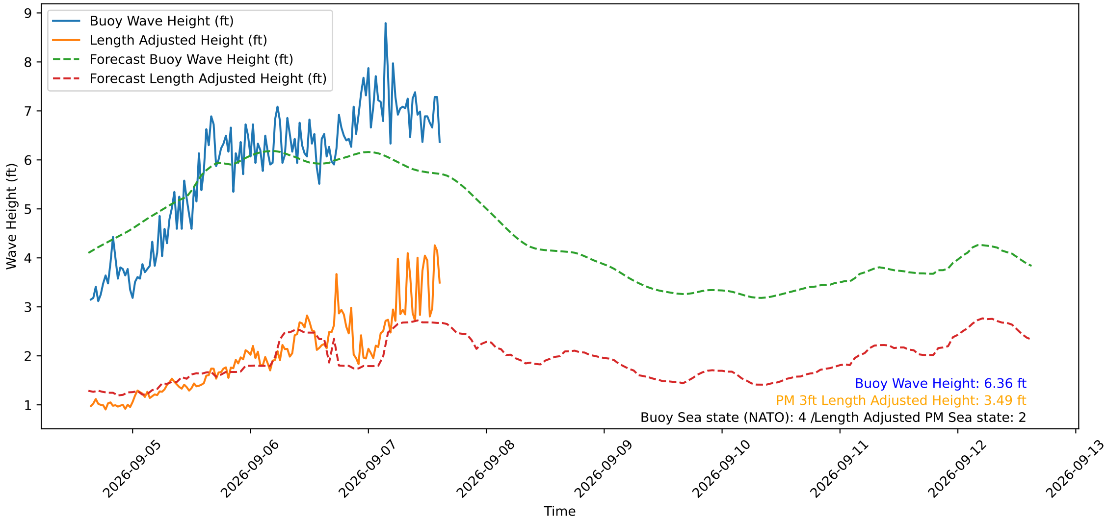
Wave Heights over Time for Green Beach at 2026-09-07 15:21:15
