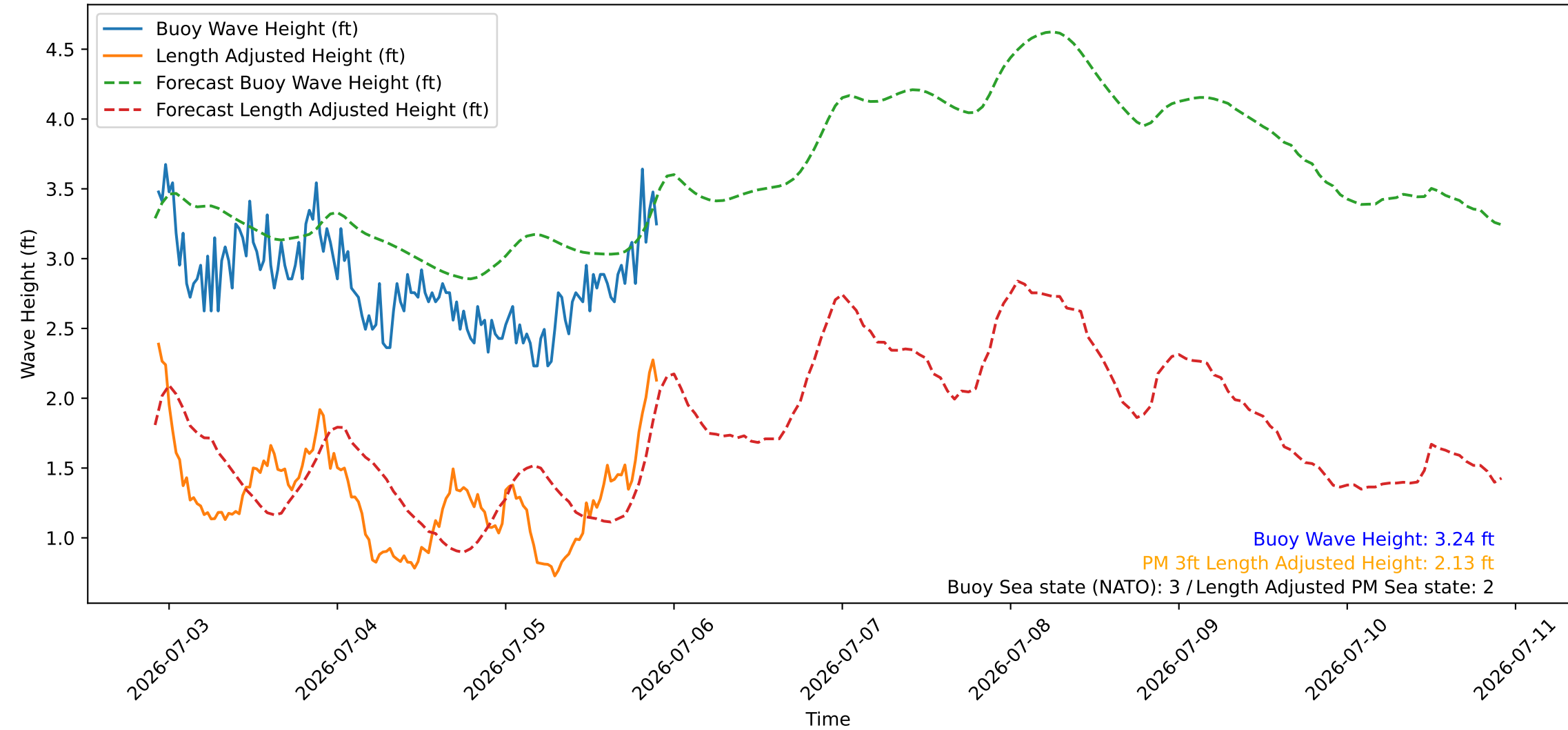
Wave Heights over Time for Red Beach at 2026-07-05 22:20:47
