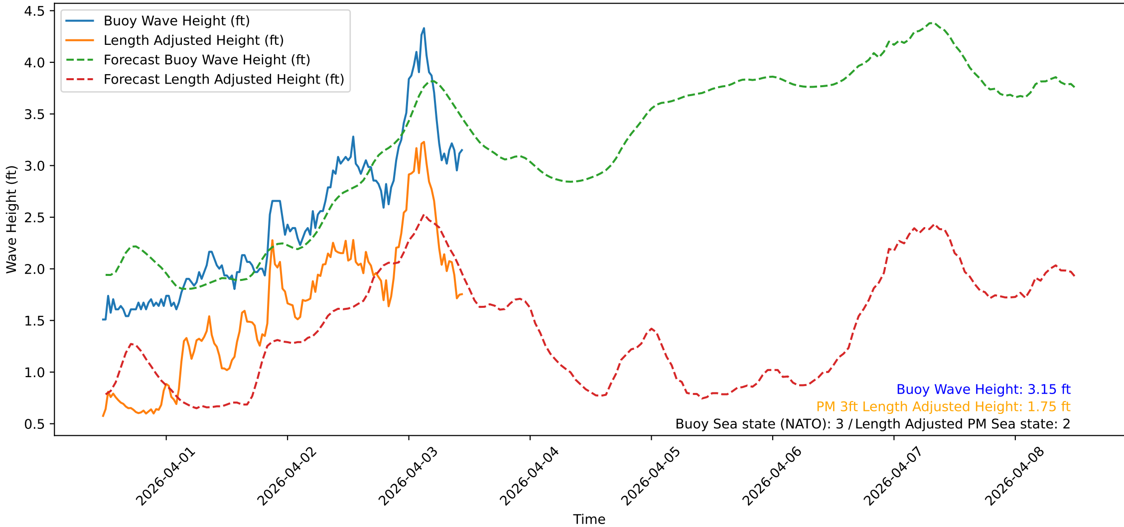
Wave Heights over Time for Green Beach at 2026-04-03 11:31:09
