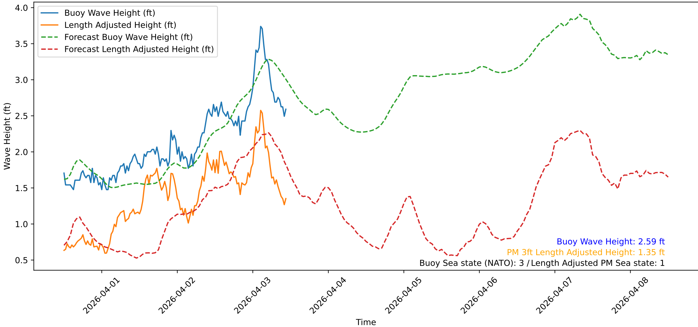
Wave Heights over Time for Red Beach at 2026-04-03 11:30:47
