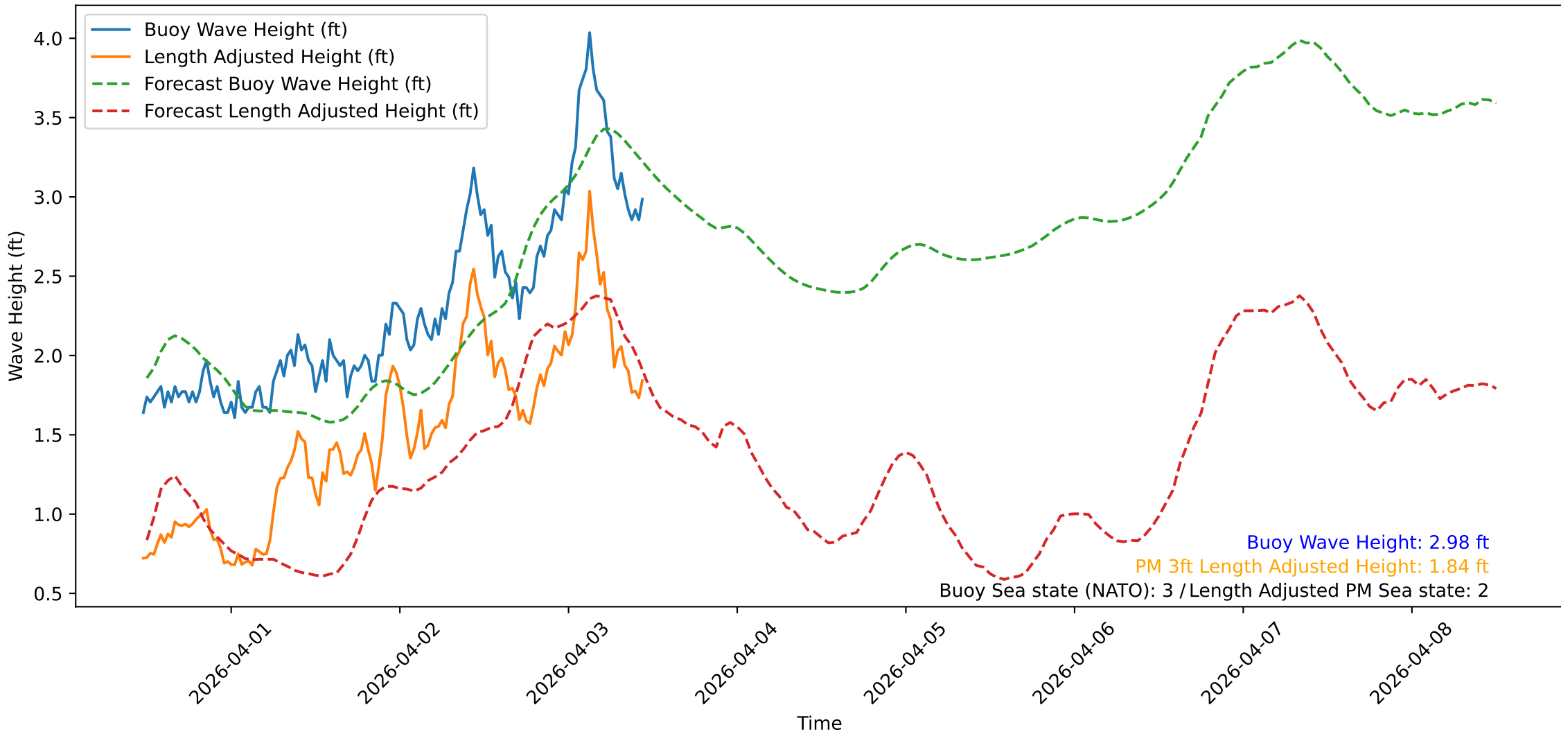
Wave Heights over Time for Oceanside Harbor at 2026-04-03 11:30:31
