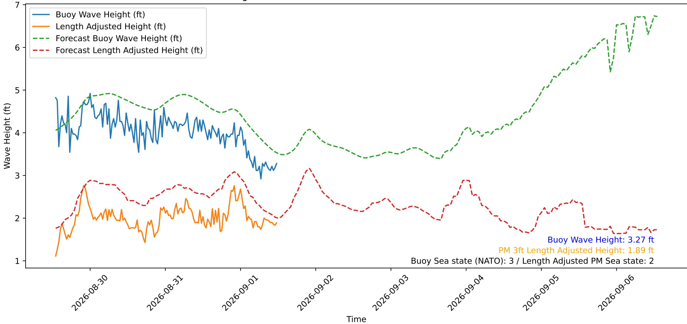
Wave Heights over Time for Green Beach at 2026-09-01 12:31:12
