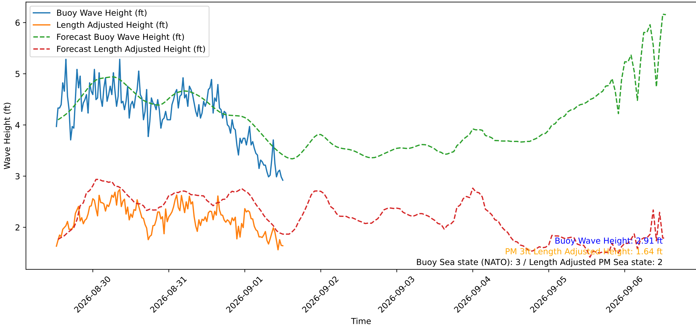
Wave Heights over Time for Oceanside Harbor at 2026-09-01 12:30:30
