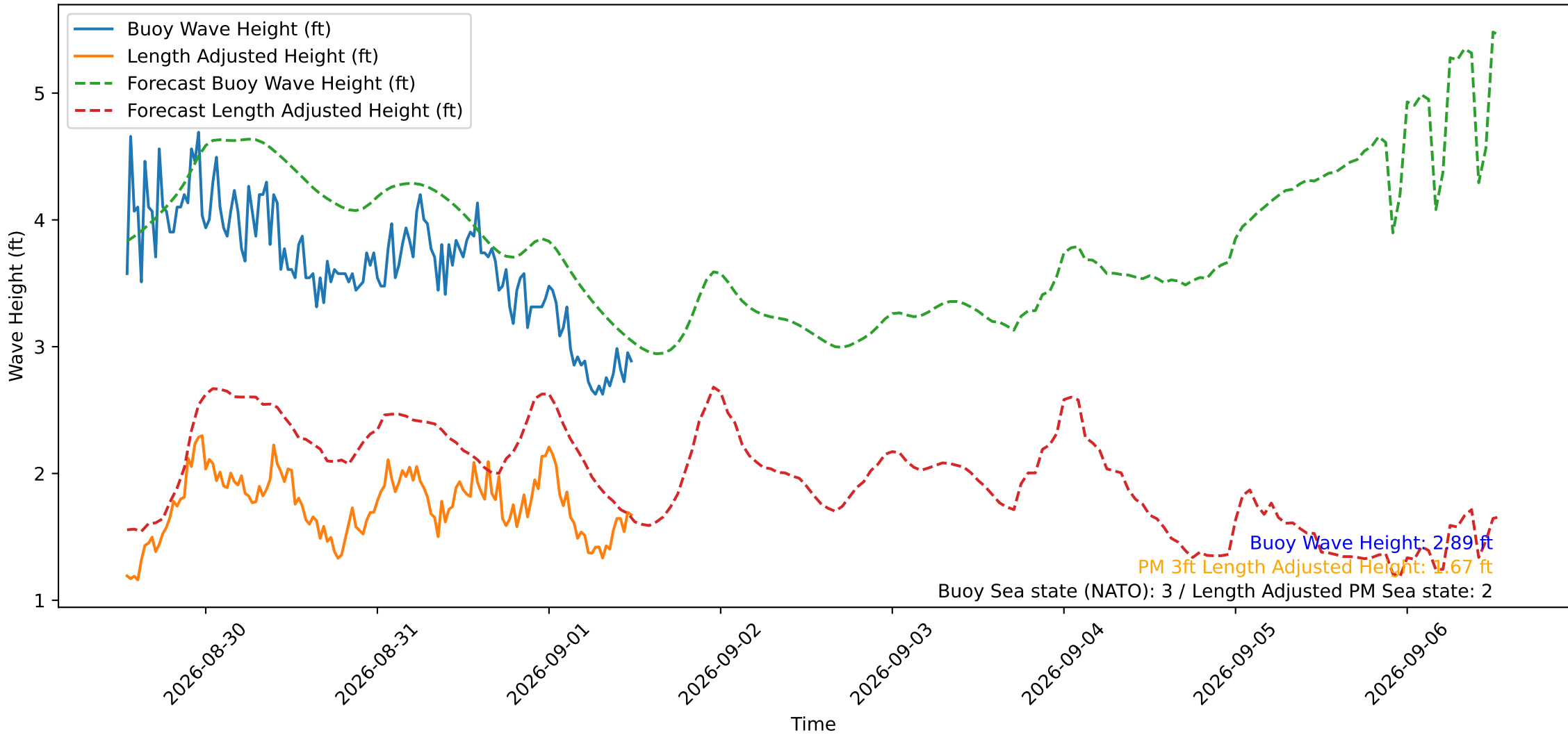
Wave Heights over Time for Red Beach at 2026-09-01 12:30:49
