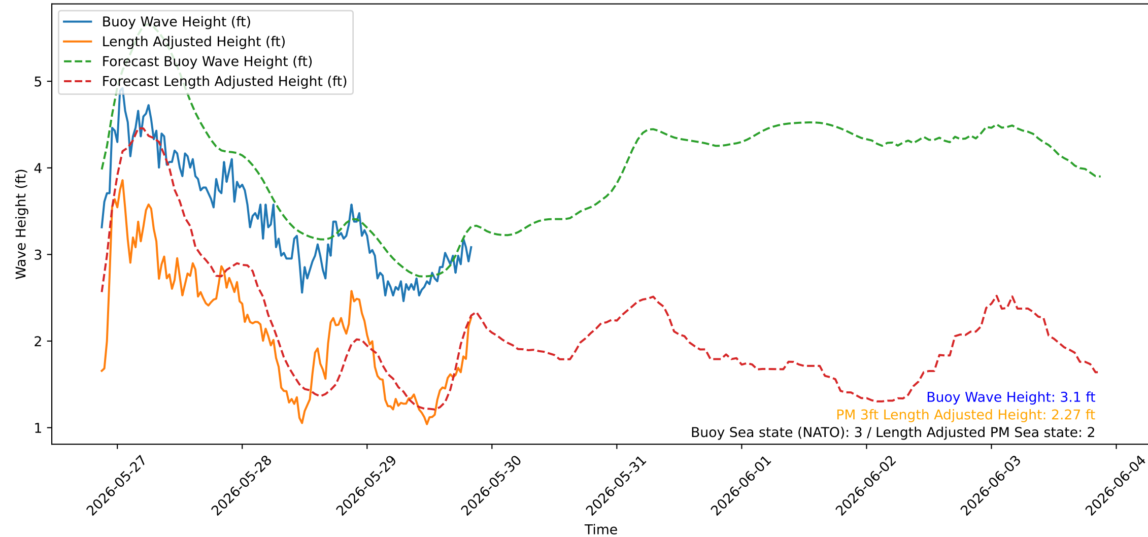
Wave Heights over Time for Green Beach at 2026-05-29 20:51:06
