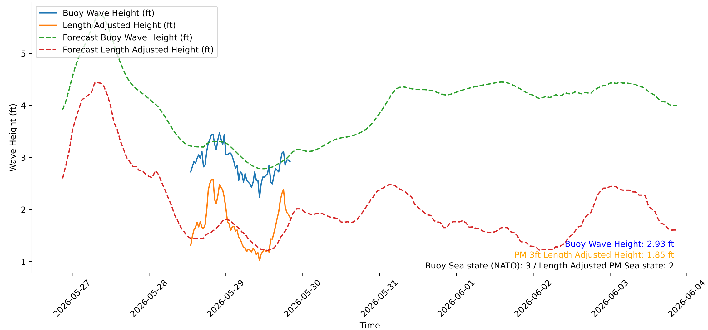
Wave Heights over Time for Oceanside Harbor at 2026-05-29 20:50:23
