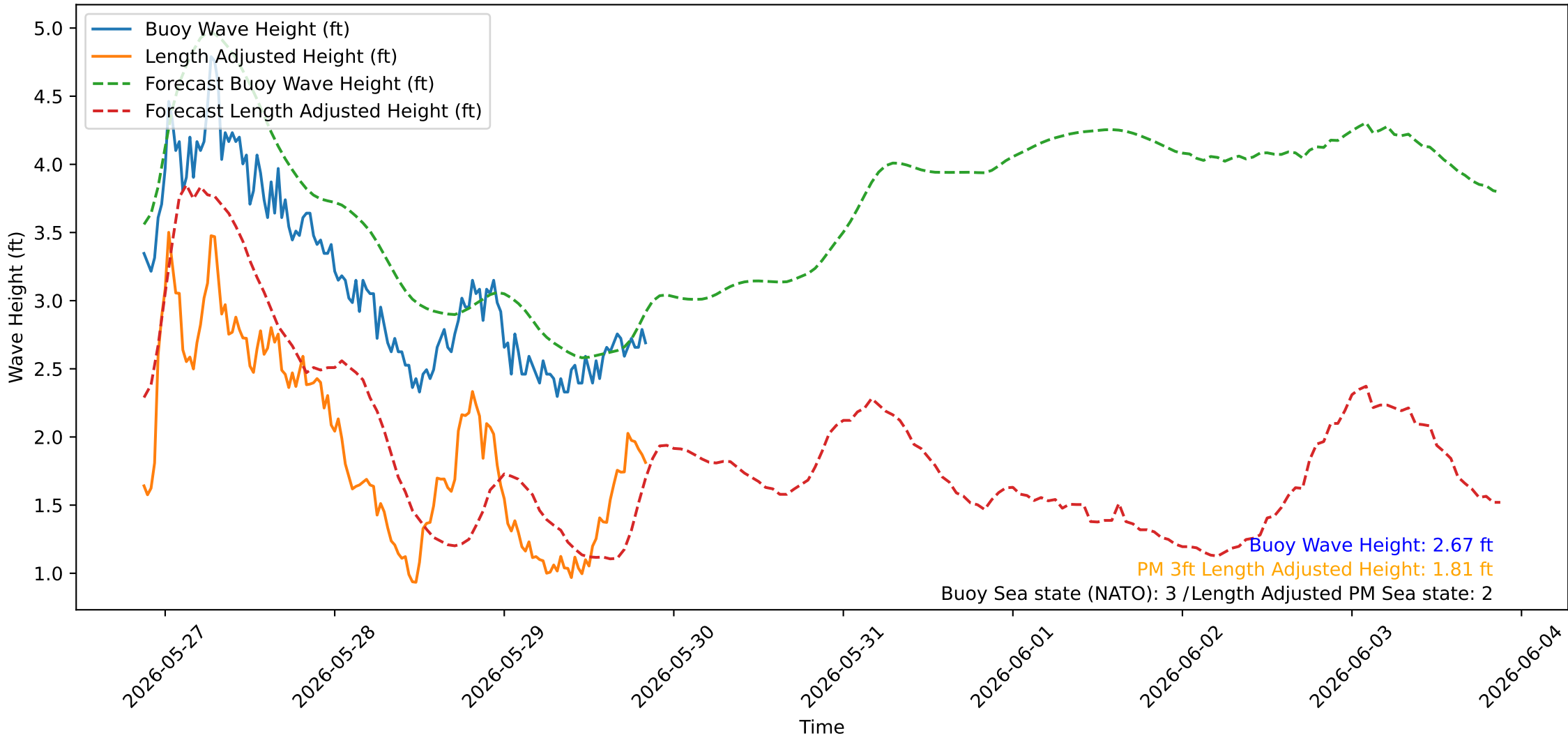
Wave Heights over Time for Red Beach at 2026-05-29 20:50:43
