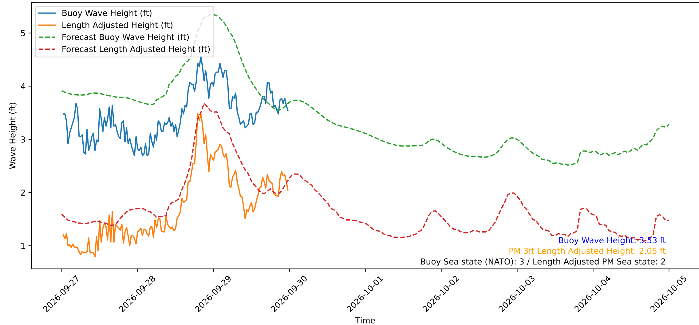
Wave Heights over Time for Green Beach at 2026-09-30 00:11:14
