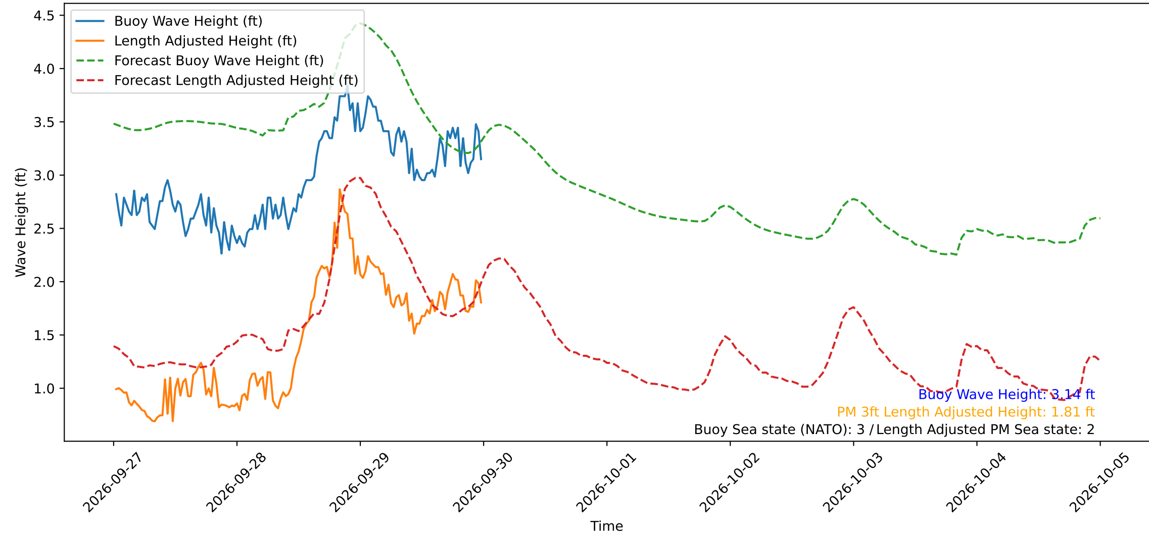
Wave Heights over Time for Red Beach at 2026-09-30 00:10:51
