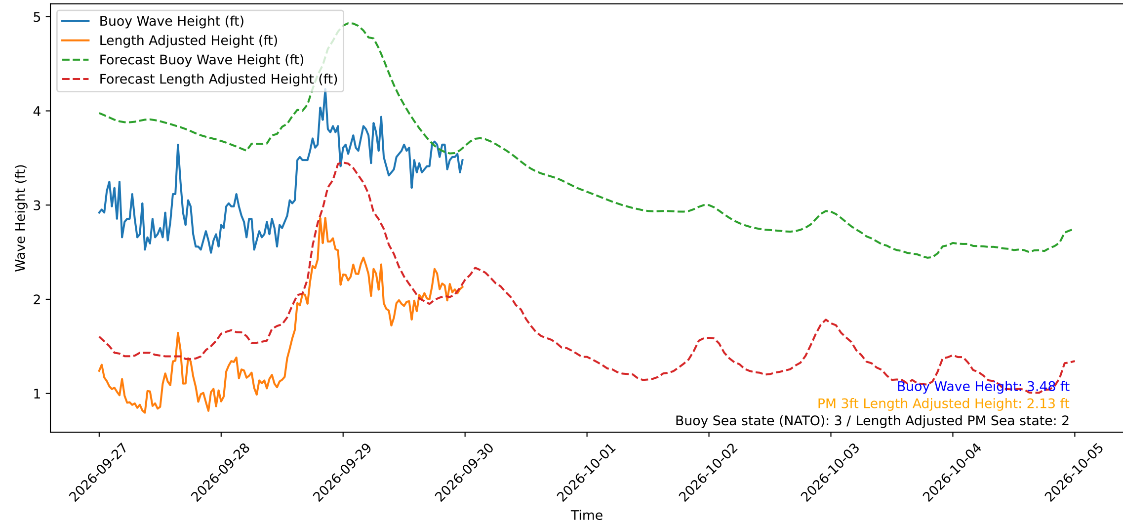
Wave Heights over Time for Oceanside Harbor at 2026-09-30 00:10:31
