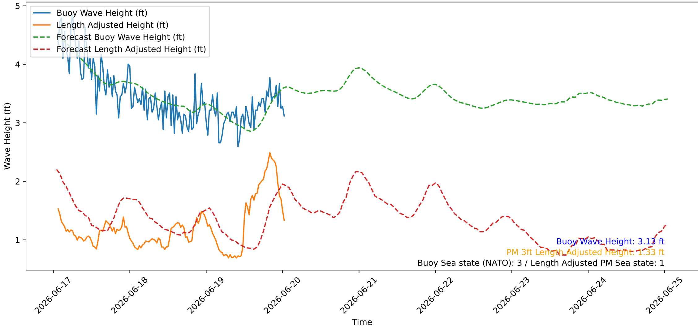
Wave Heights over Time for Red Beach at 2026-06-20 01:10:45
