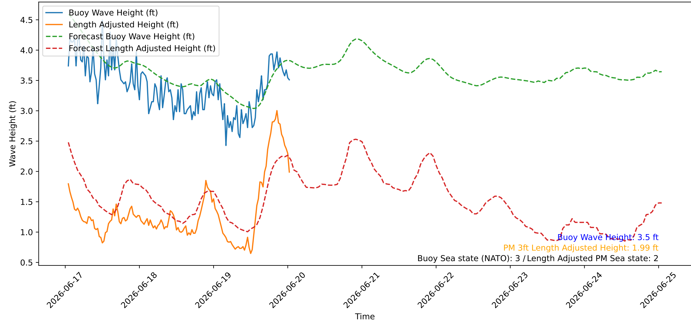
Wave Heights over Time for Green Beach at 2026-06-20 01:11:07
