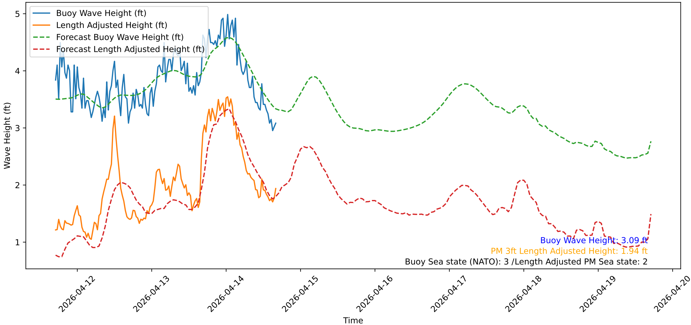
Wave Heights over Time for Green Beach at 2026-04-14 16:51:15
