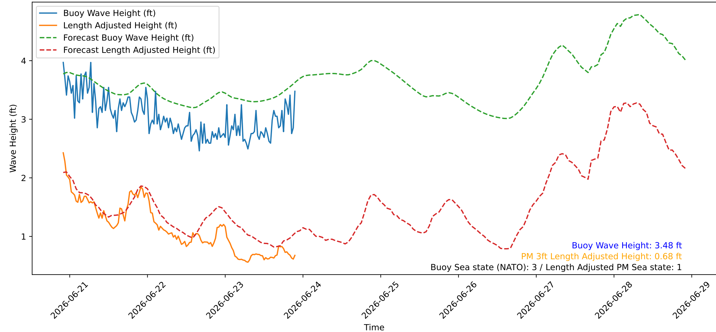
Wave Heights over Time for Green Beach at 2026-06-23 22:11:08
