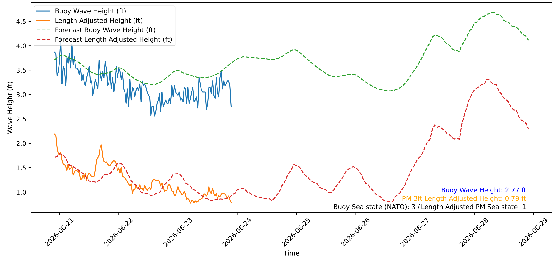
Wave Heights over Time for Oceanside Harbor at 2026-06-23 22:10:26
