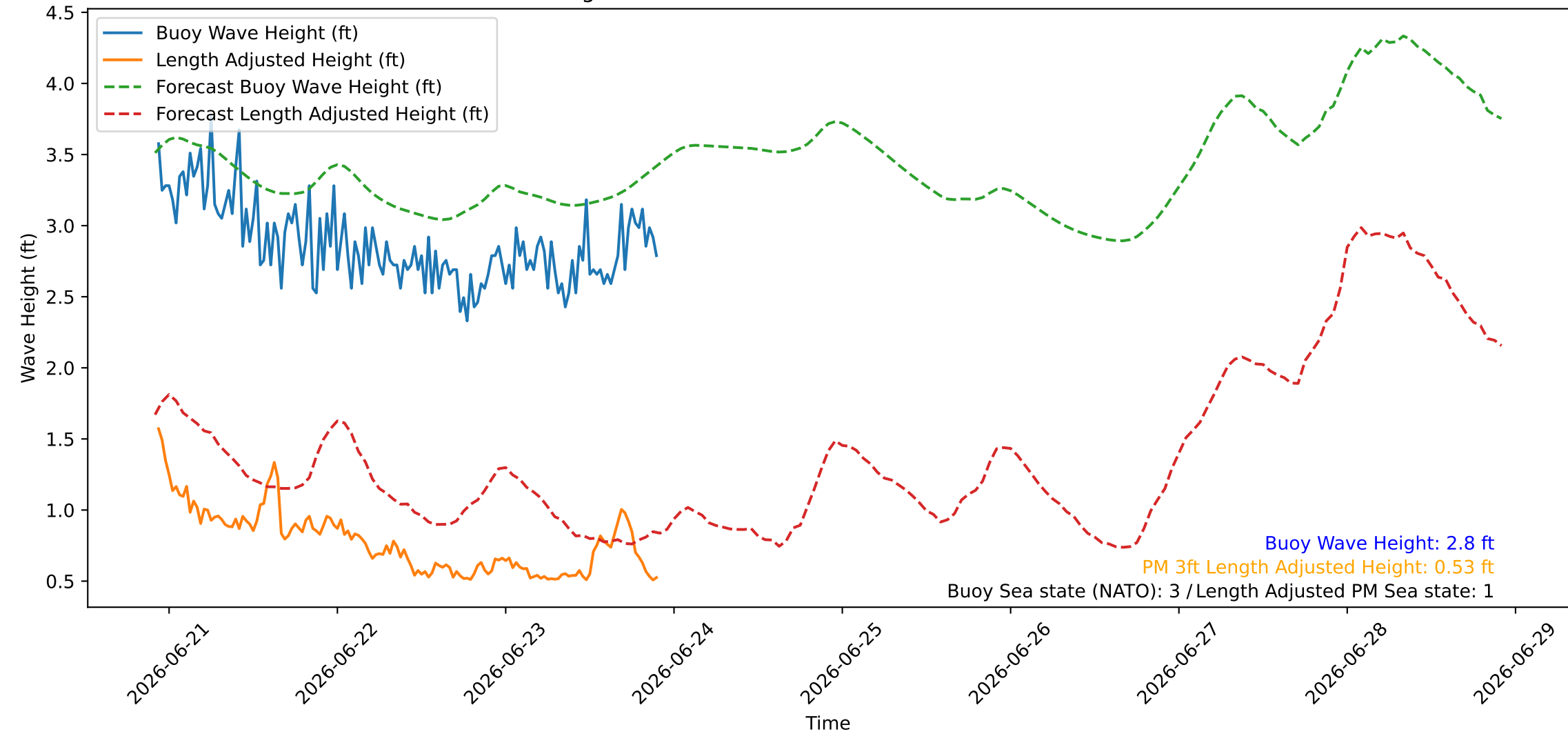
Wave Heights over Time for Red Beach at 2026-06-23 22:10:45
