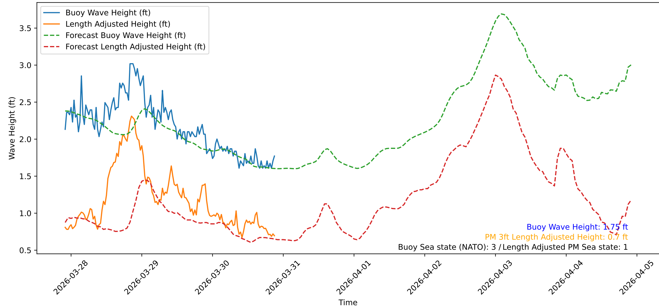
Wave Heights over Time for Red Beach at 2026-03-30 21:40:47
