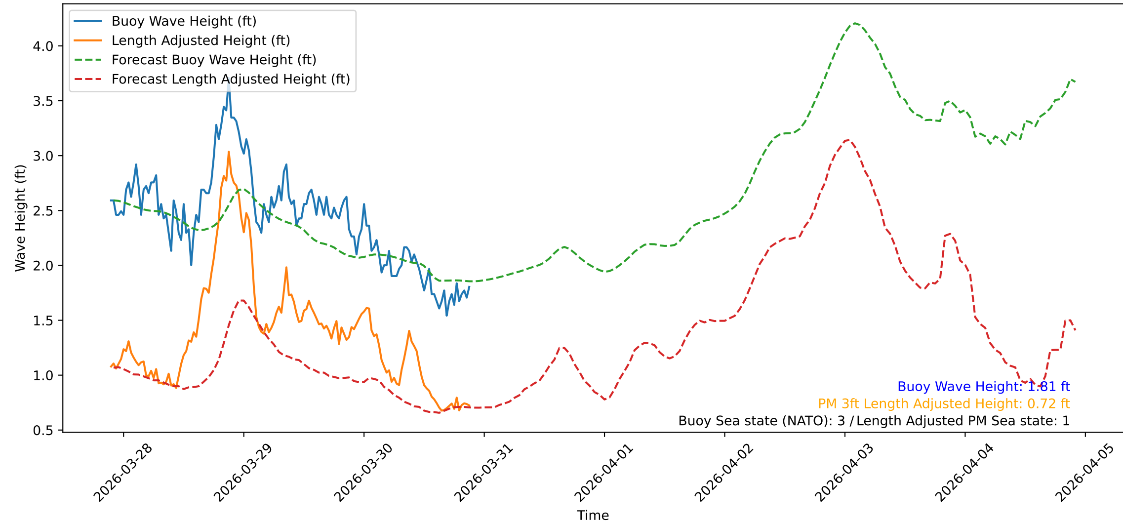
Wave Heights over Time for Green Beach at 2026-03-30 21:41:09
