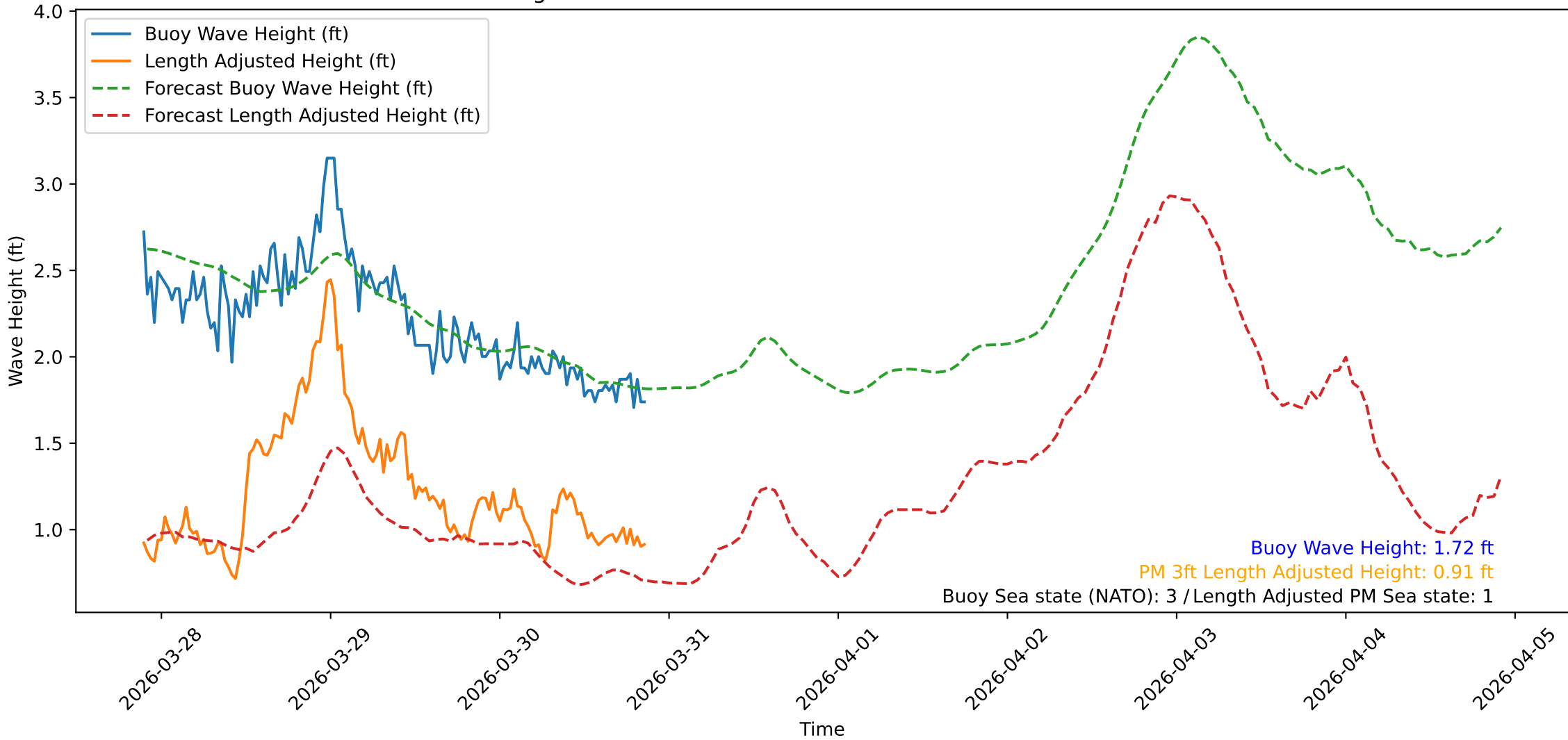
Wave Heights over Time for Oceanside Harbor at 2026-03-30 21:40:31
