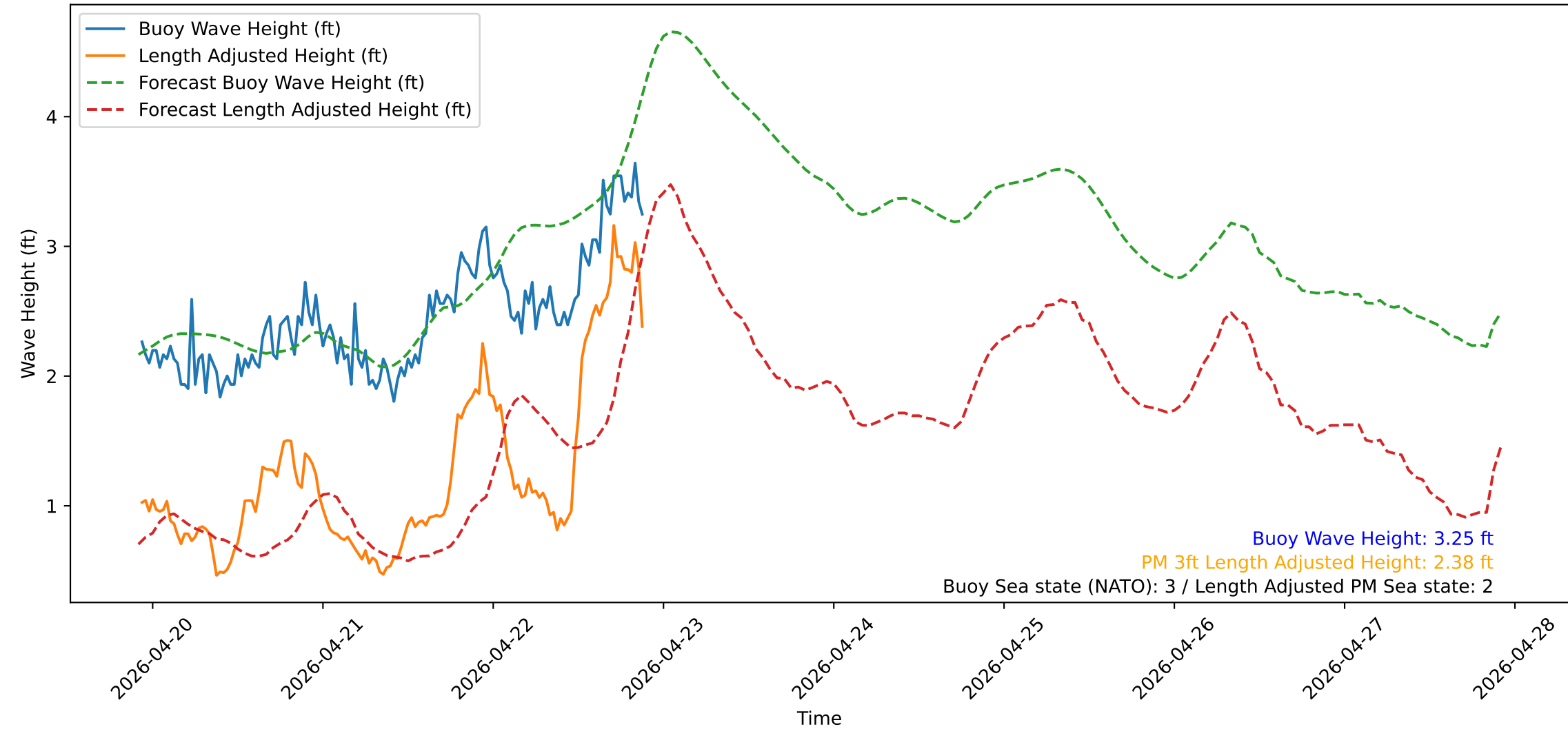
Wave Heights over Time for Red Beach at 2026-04-22 22:00:50
