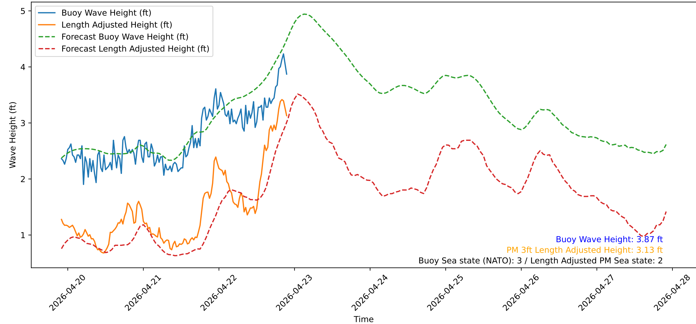
Wave Heights over Time for Oceanside Harbor at 2026-04-22 22:00:31
