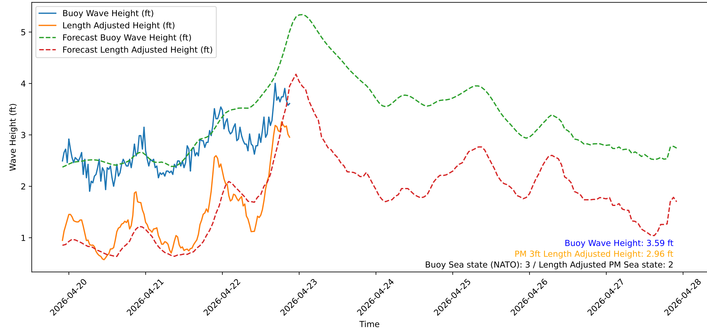
Wave Heights over Time for Green Beach at 2026-04-22 22:01:12
