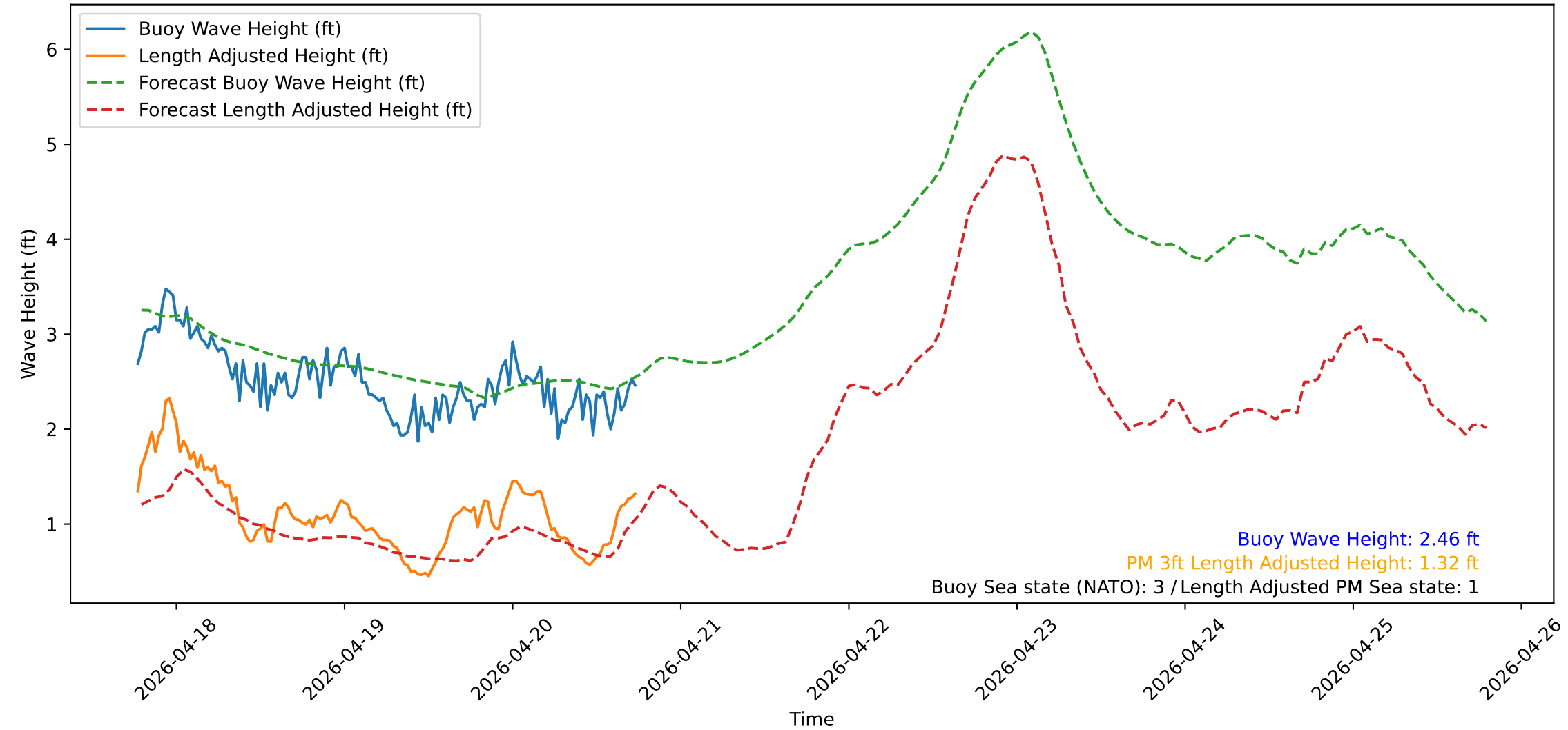
Wave Heights over Time for Green Beach at 2026-04-20 18:31:13
