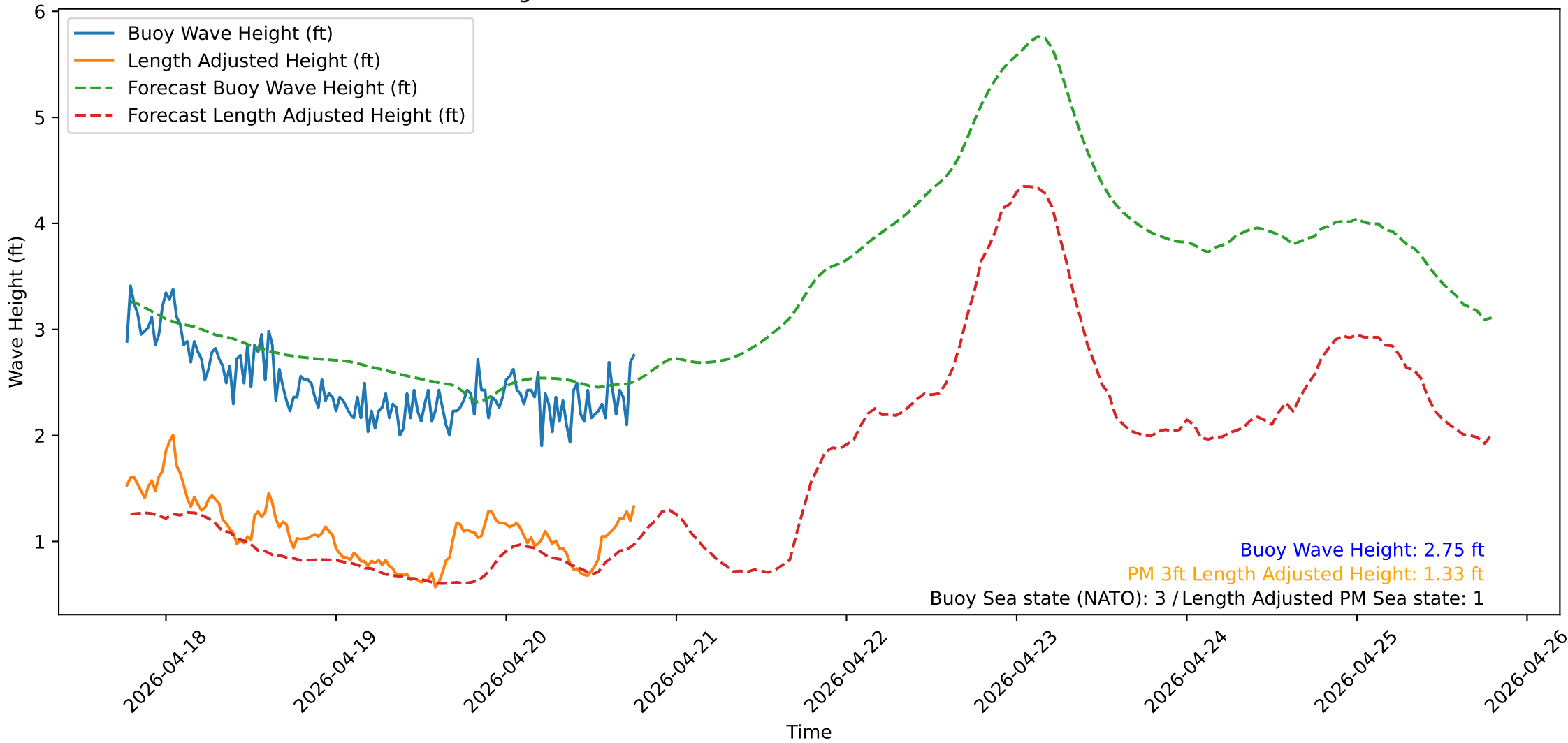
Wave Heights over Time for Oceanside Harbor at 2026-04-20 18:30:32
