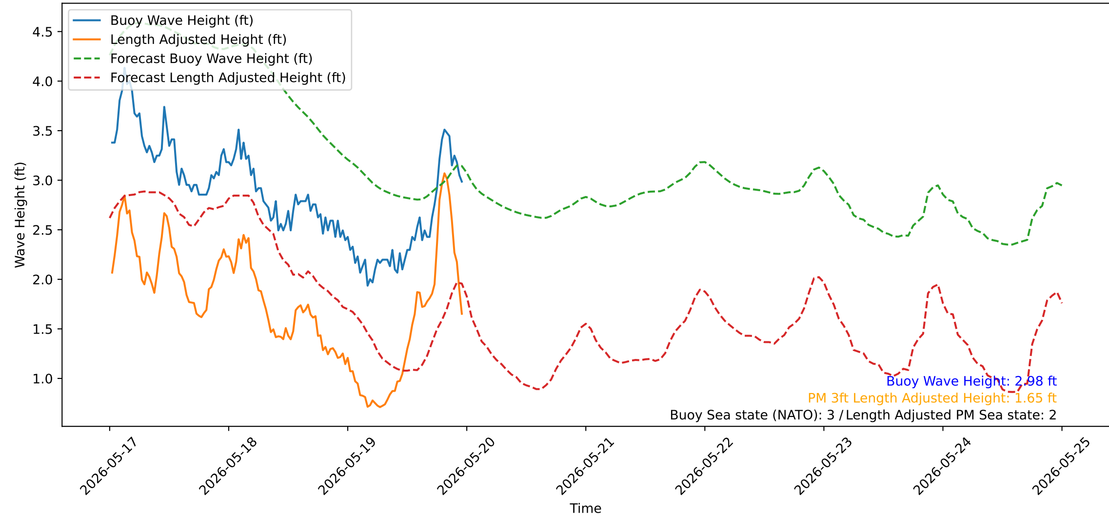
Wave Heights over Time for Red Beach at 2026-05-20 00:00:51
