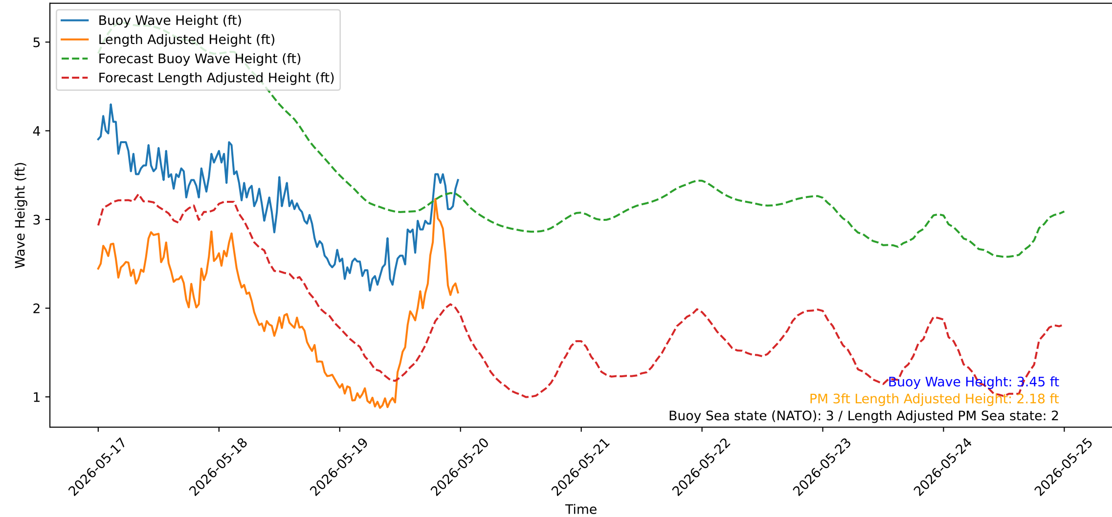
Wave Heights over Time for Oceanside Harbor at 2026-05-20 00:00:32
