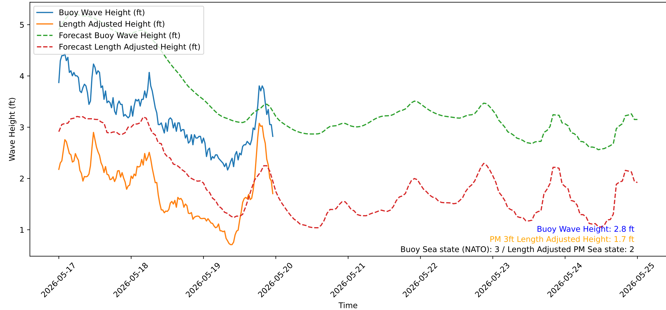
Wave Heights over Time for Green Beach at 2026-05-20 00:01:13
