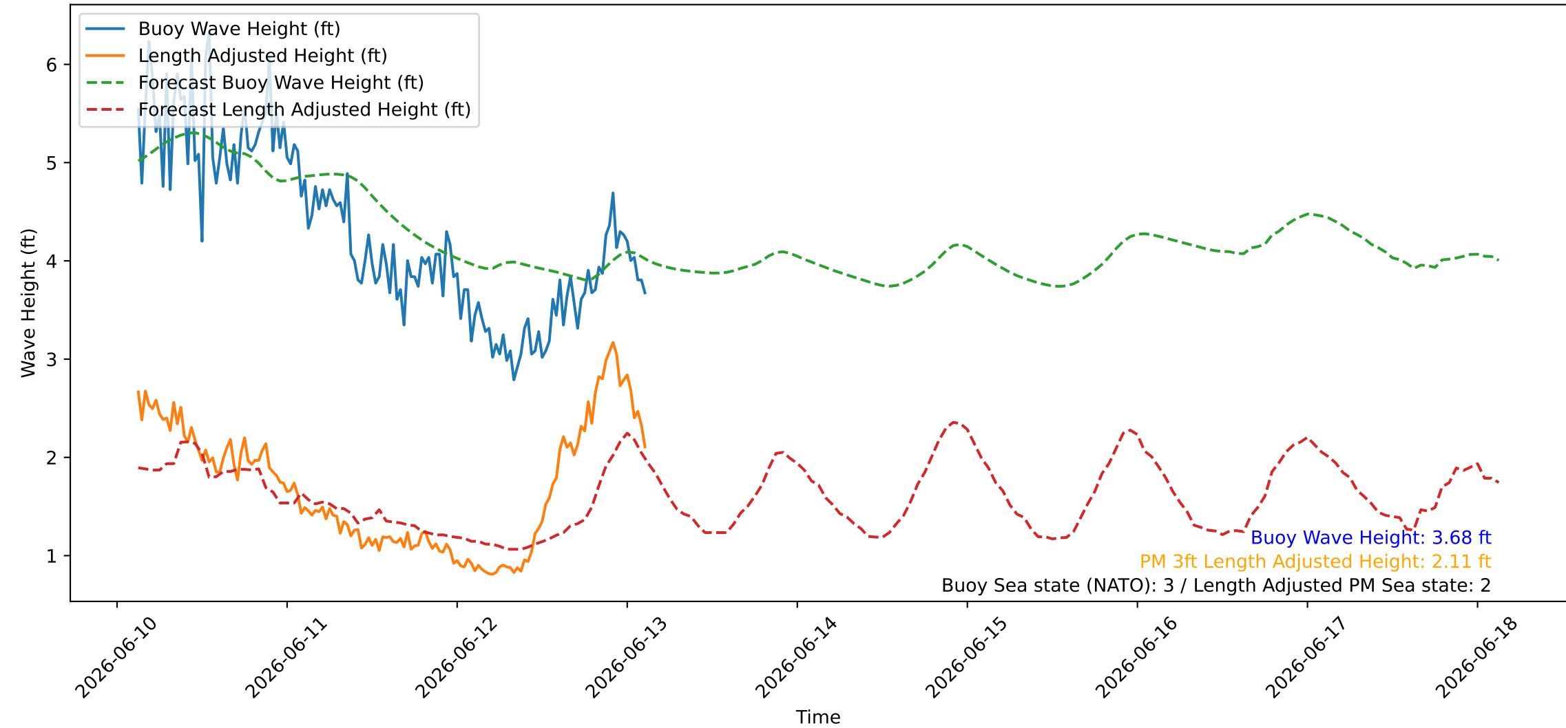
Wave Heights over Time for Oceanside Harbor at 2026-06-13 03:10:26
