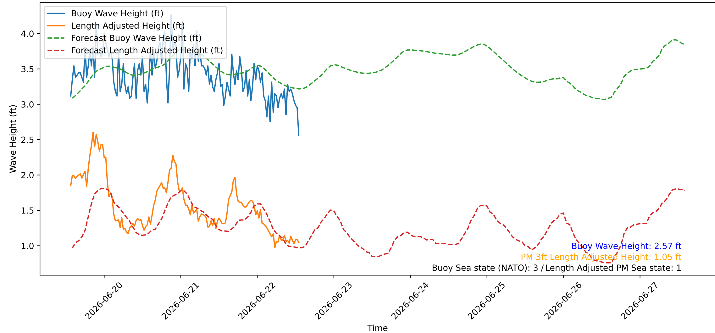
Wave Heights over Time for Oceanside Harbor at 2026-06-22 13:40:26
