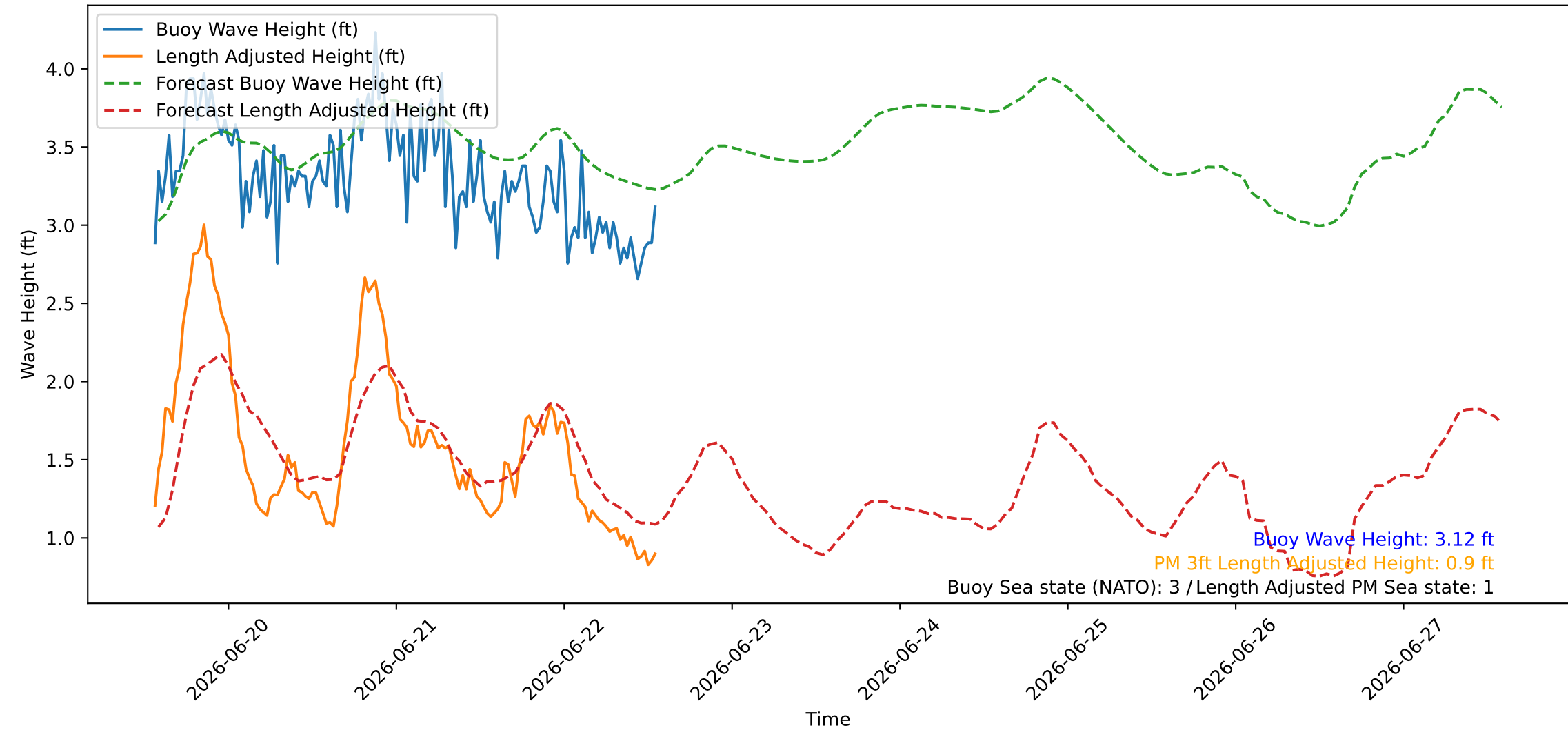
Wave Heights over Time for Green Beach at 2026-06-22 13:41:08
