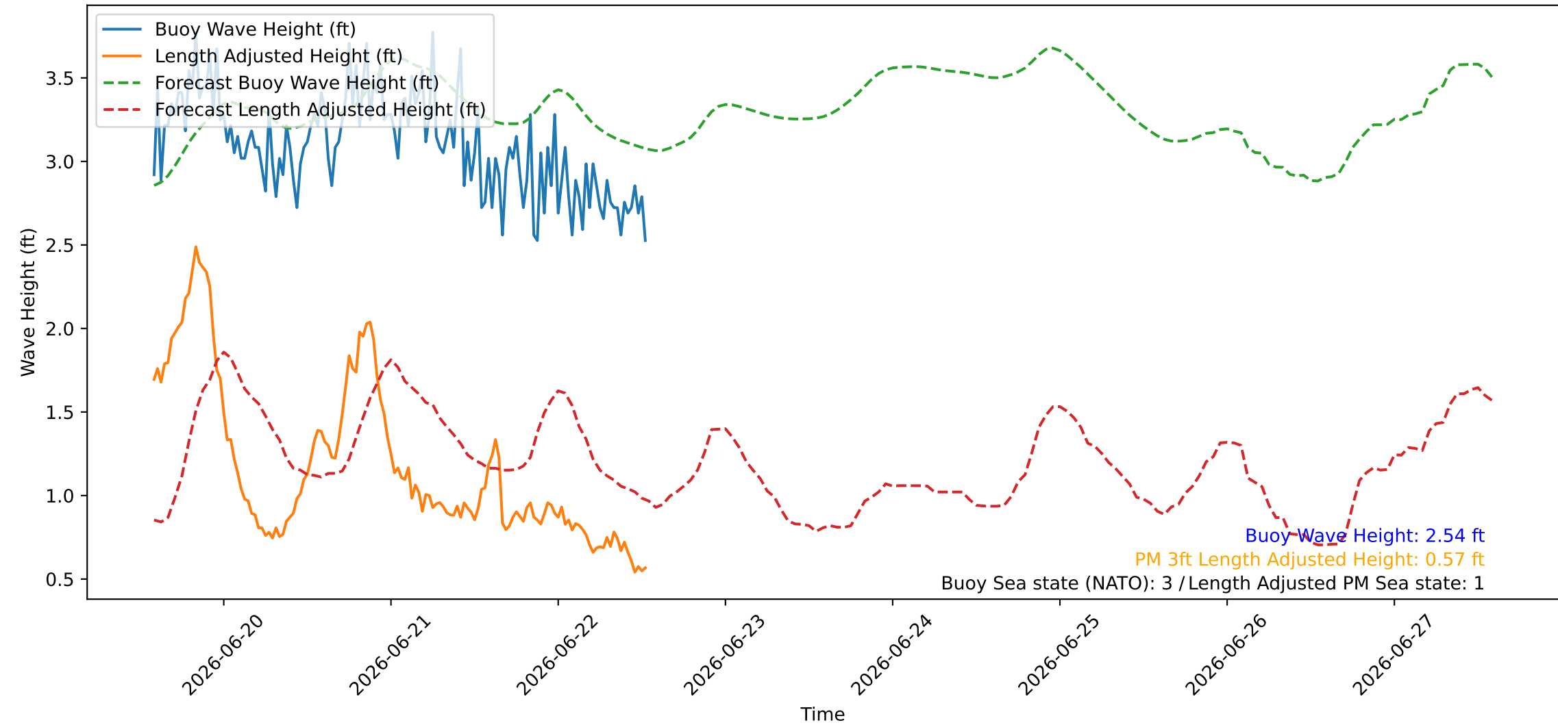
Wave Heights over Time for Red Beach at 2026-06-22 13:40:45
