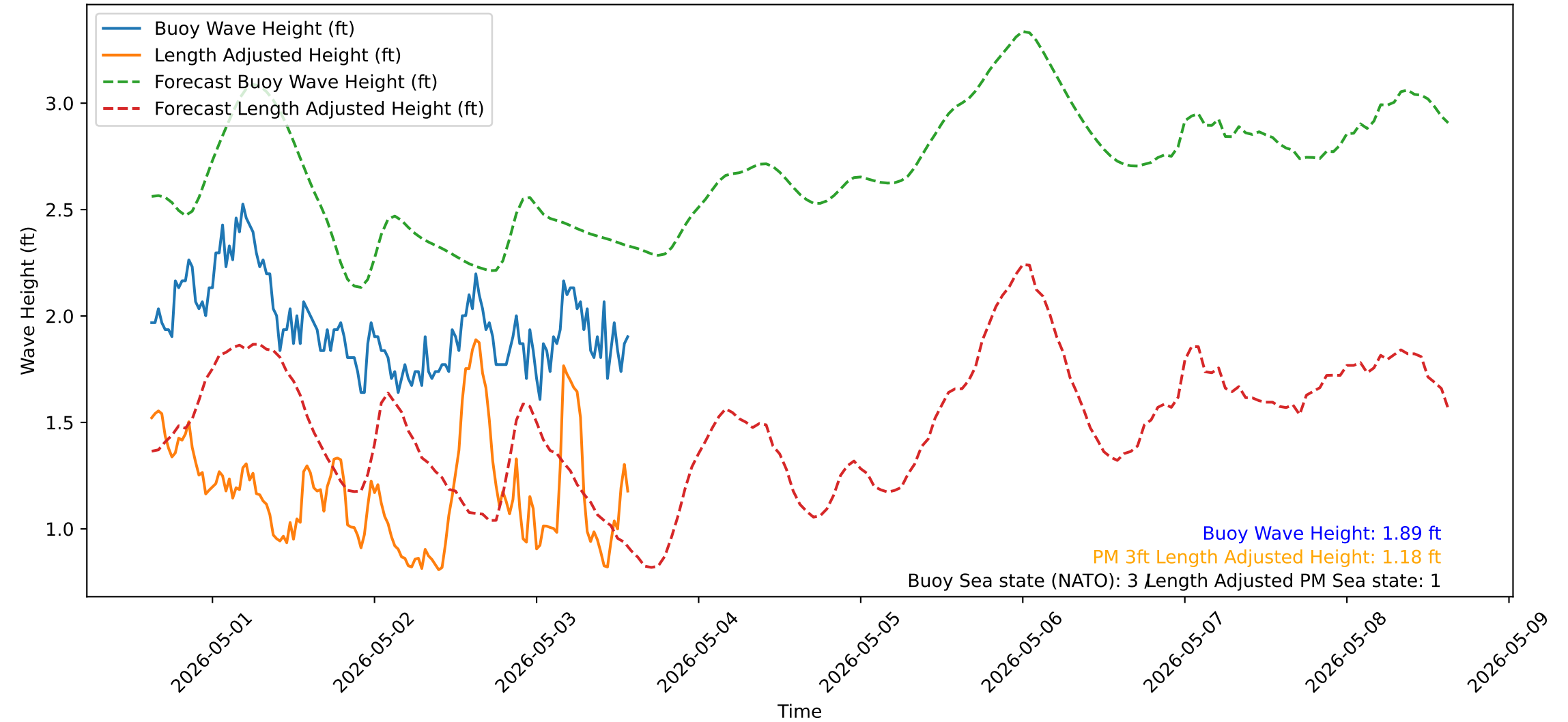
Wave Heights over Time for Red Beach at 2026-05-03 14:30:51
