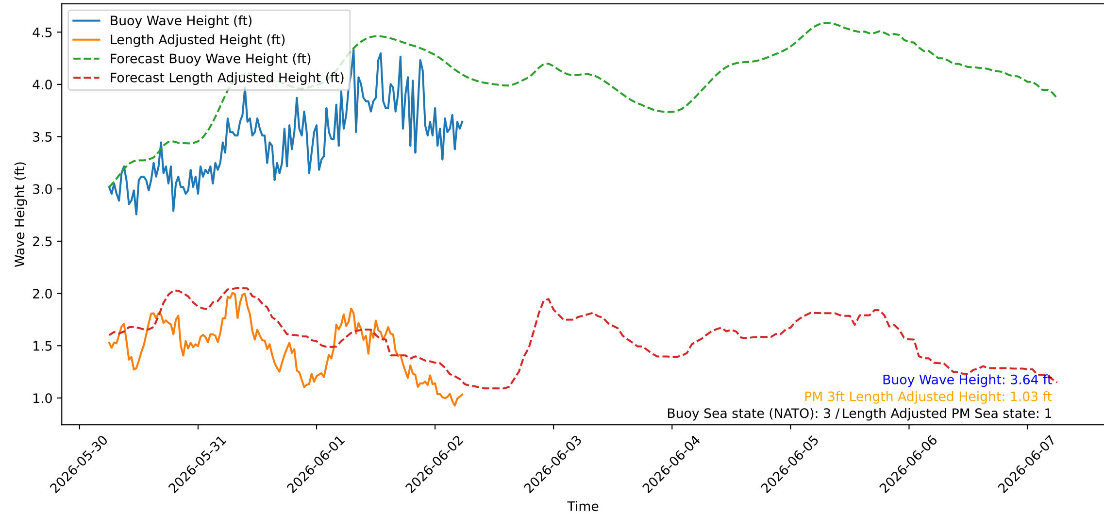
Wave Heights over Time for Green Beach at 2026-06-02 06:11:07
