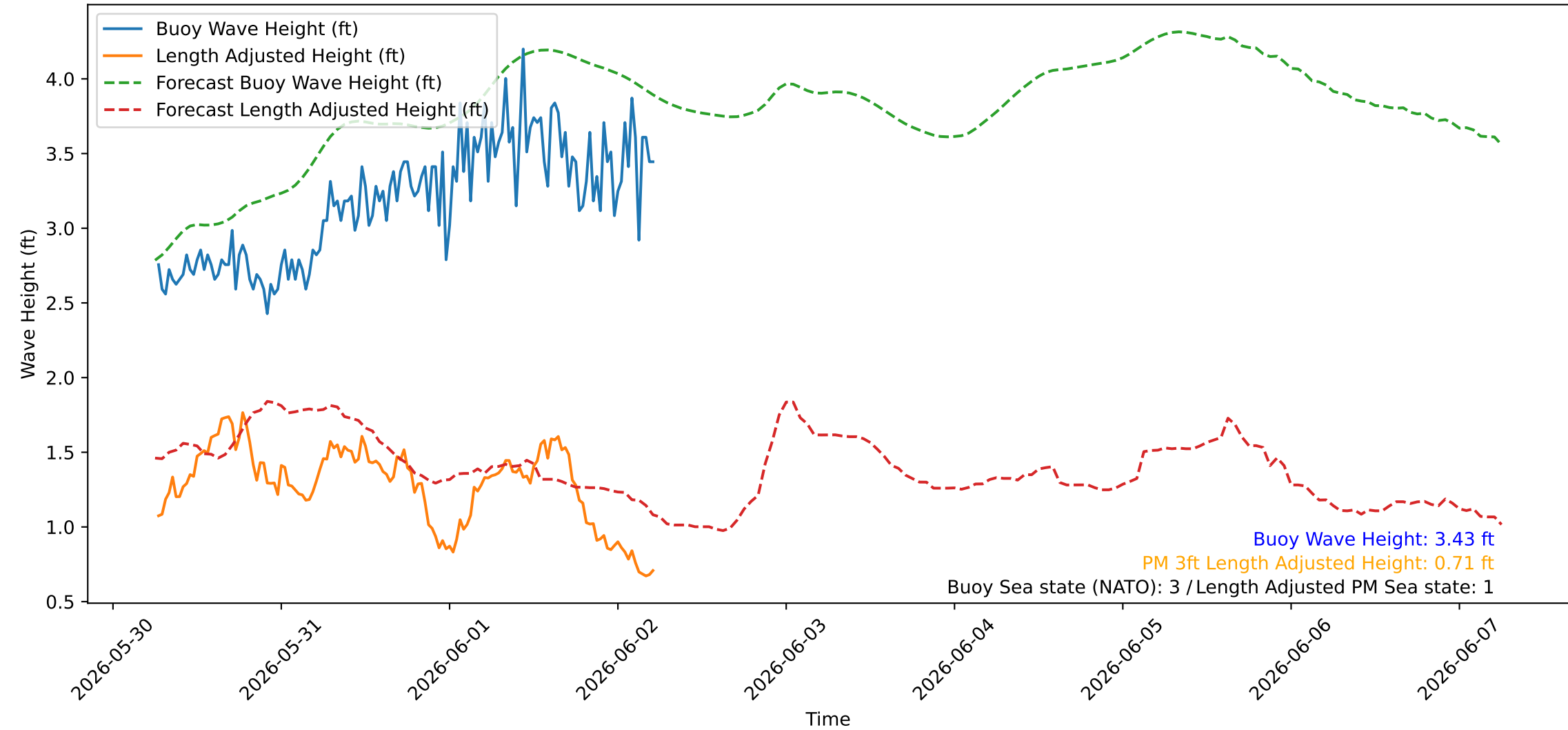
Wave Heights over Time for Red Beach at 2026-06-02 06:10:45
