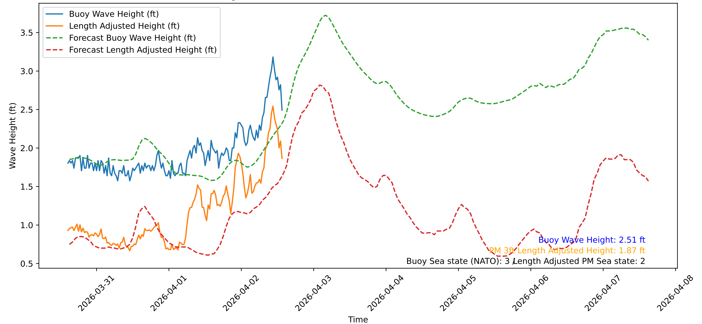
Wave Heights over Time for Oceanside Harbor at 2026-04-02 14:30:31
