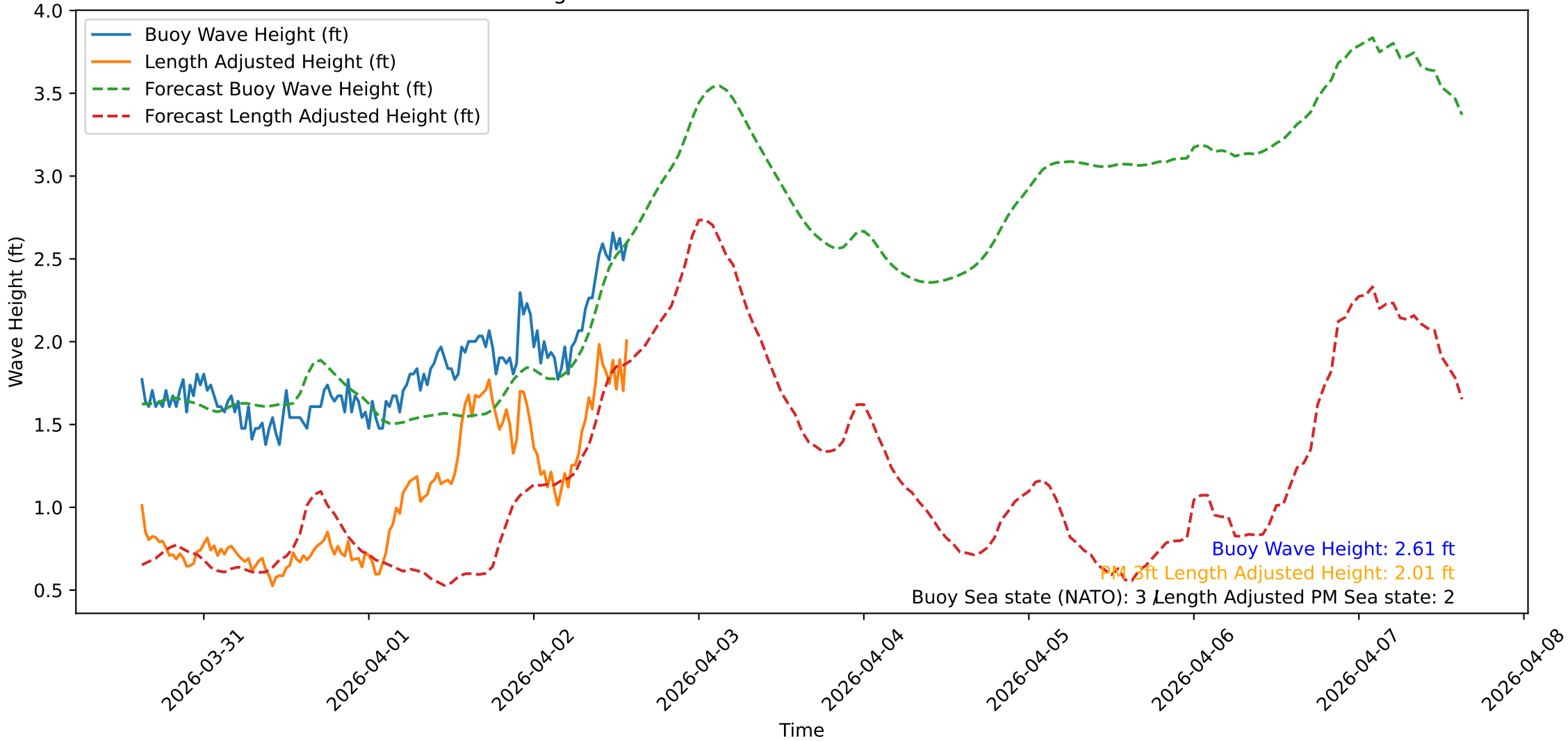
Wave Heights over Time for Red Beach at 2026-04-02 14:30:48
