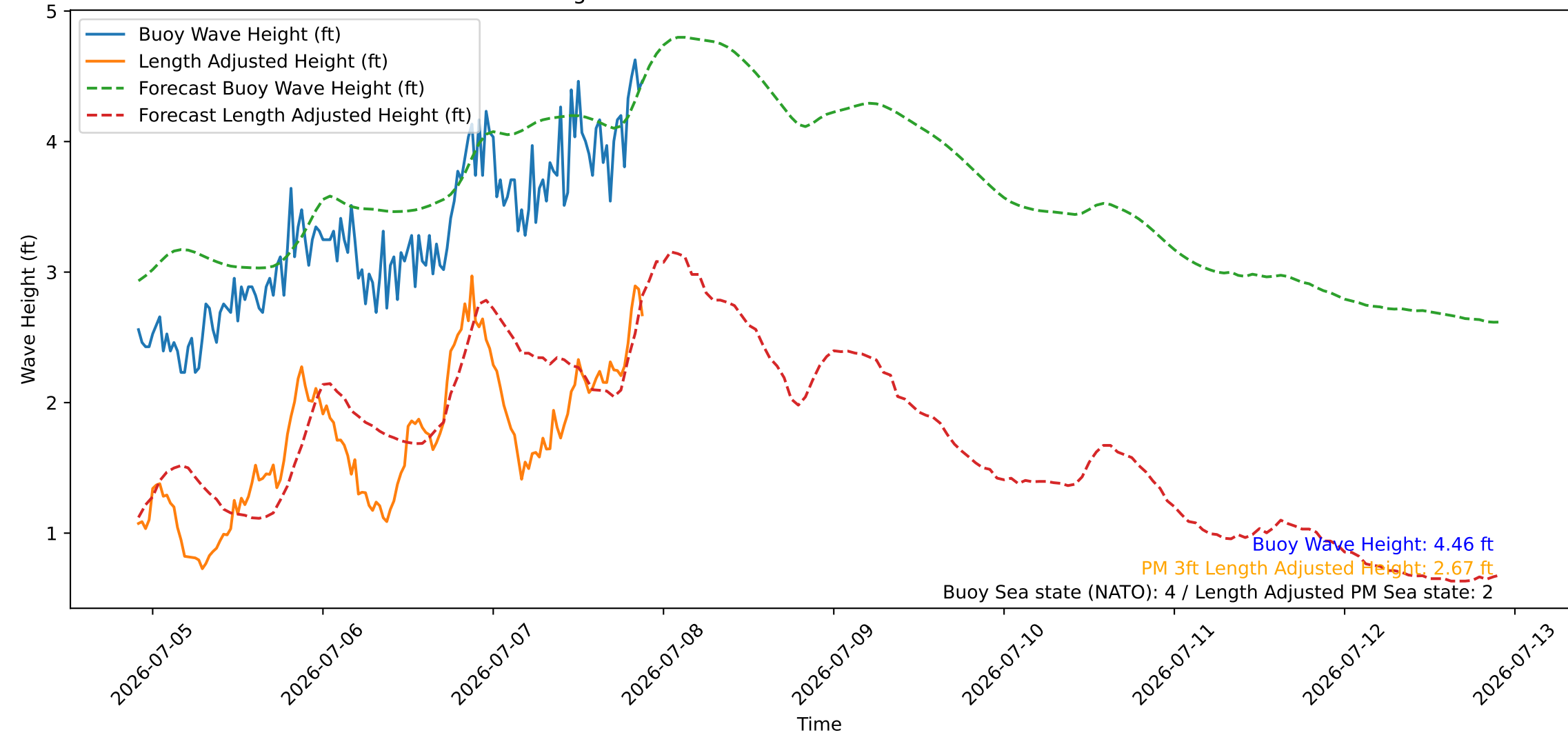
Wave Heights over Time for Red Beach at 2026-07-07 21:40:46
