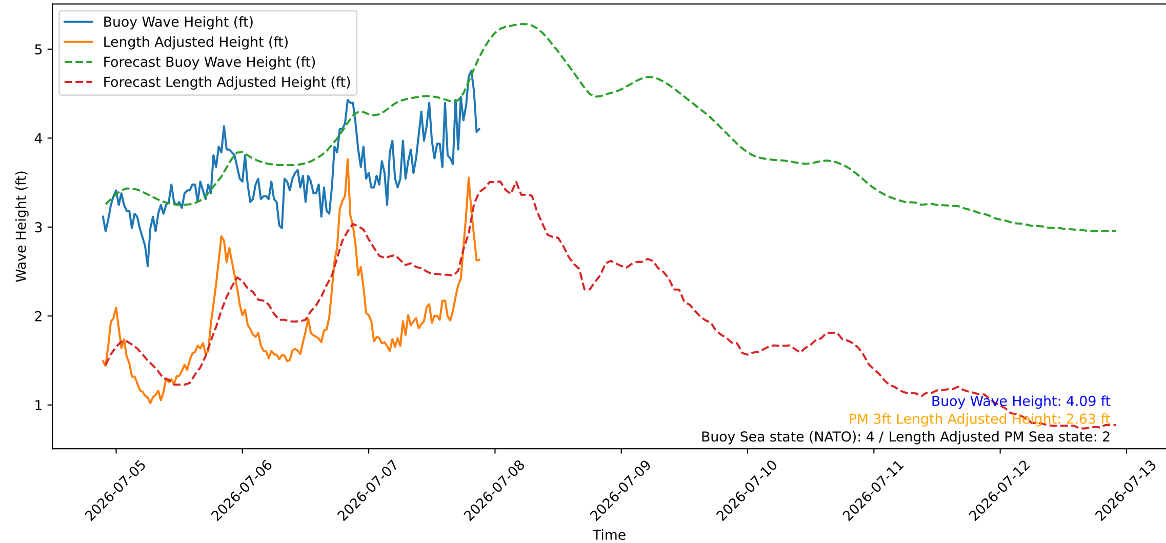
Wave Heights over Time for Green Beach at 2026-07-07 21:41:09
