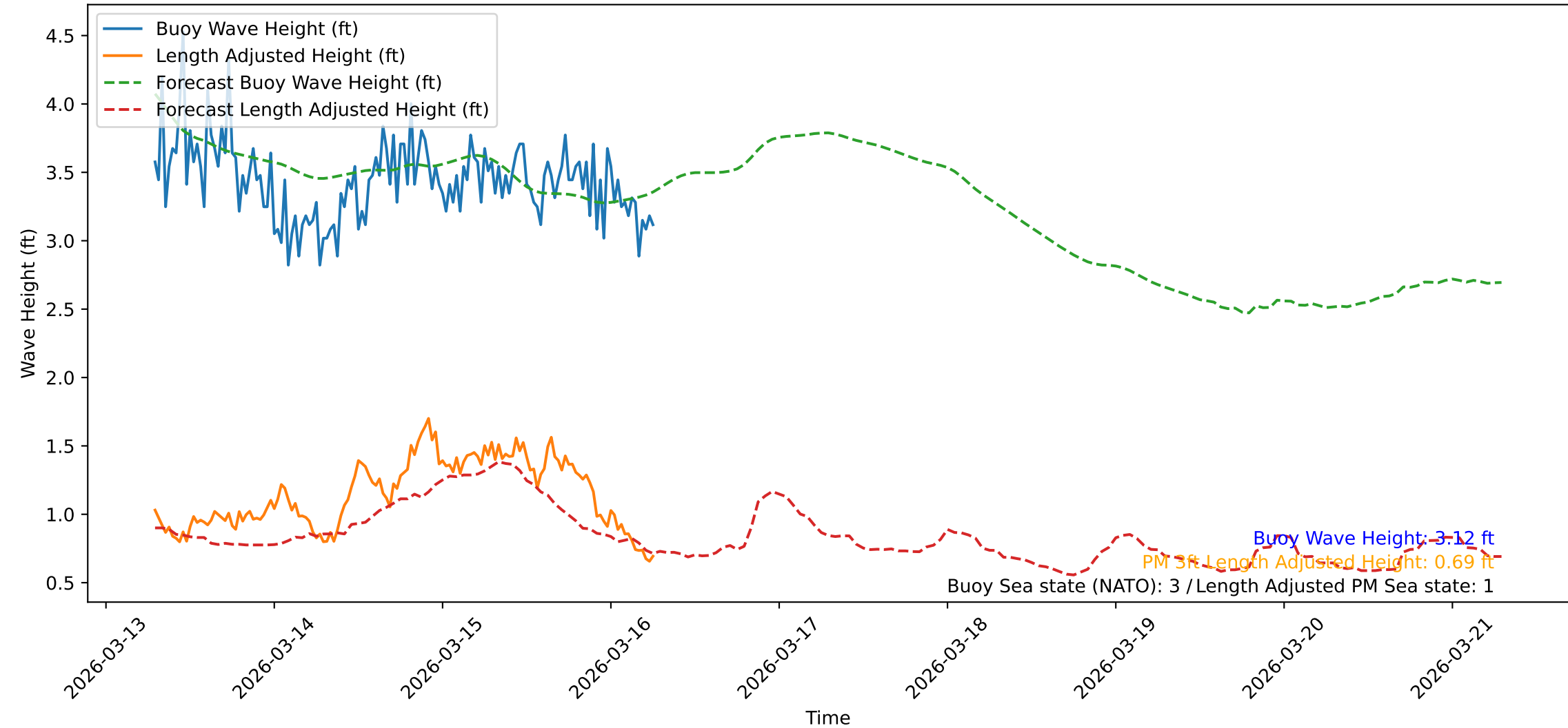
Wave Heights over Time for Green Beach at 2026-03-16 06:51:37
