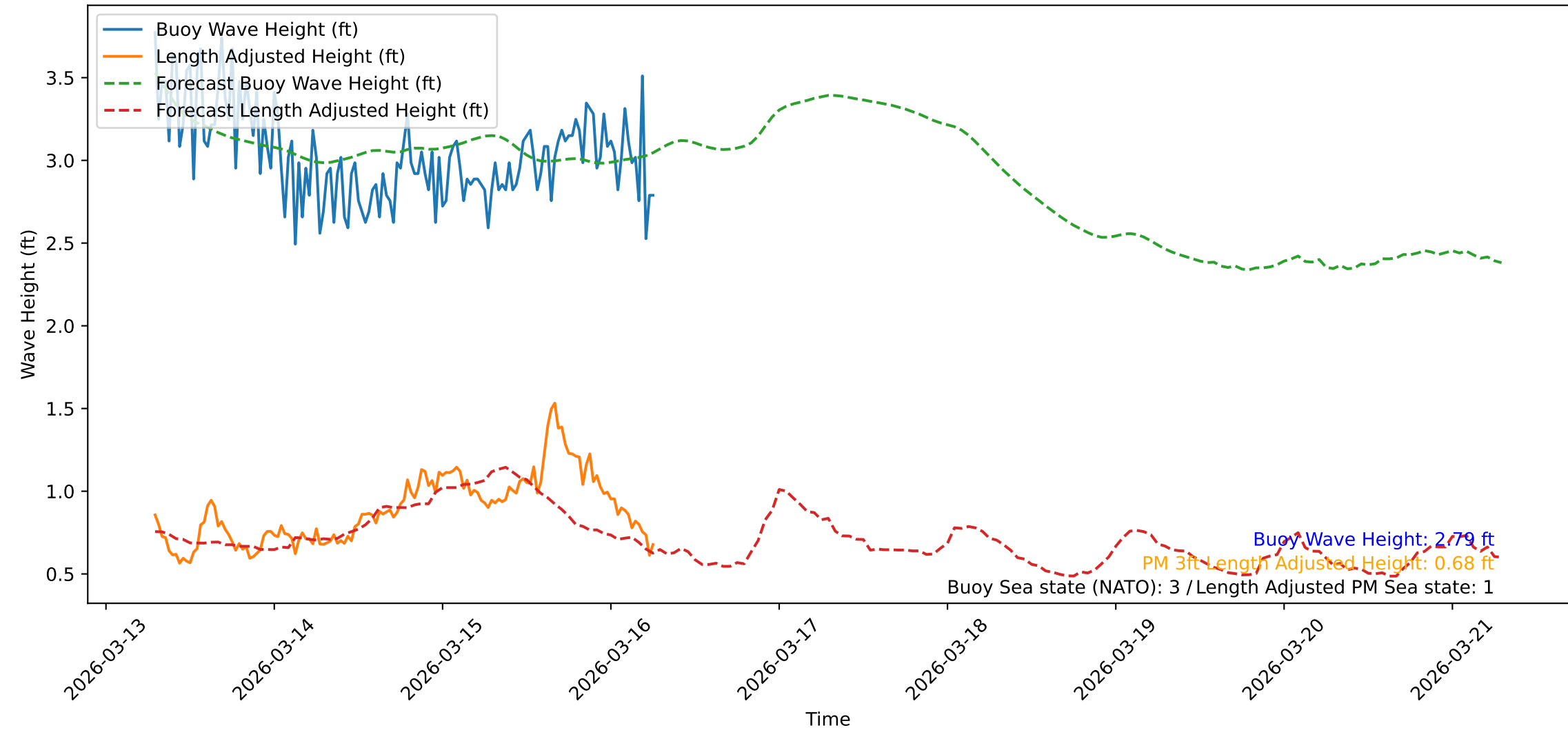
Wave Heights over Time for Red Beach at 2026-03-16 06:51:04
