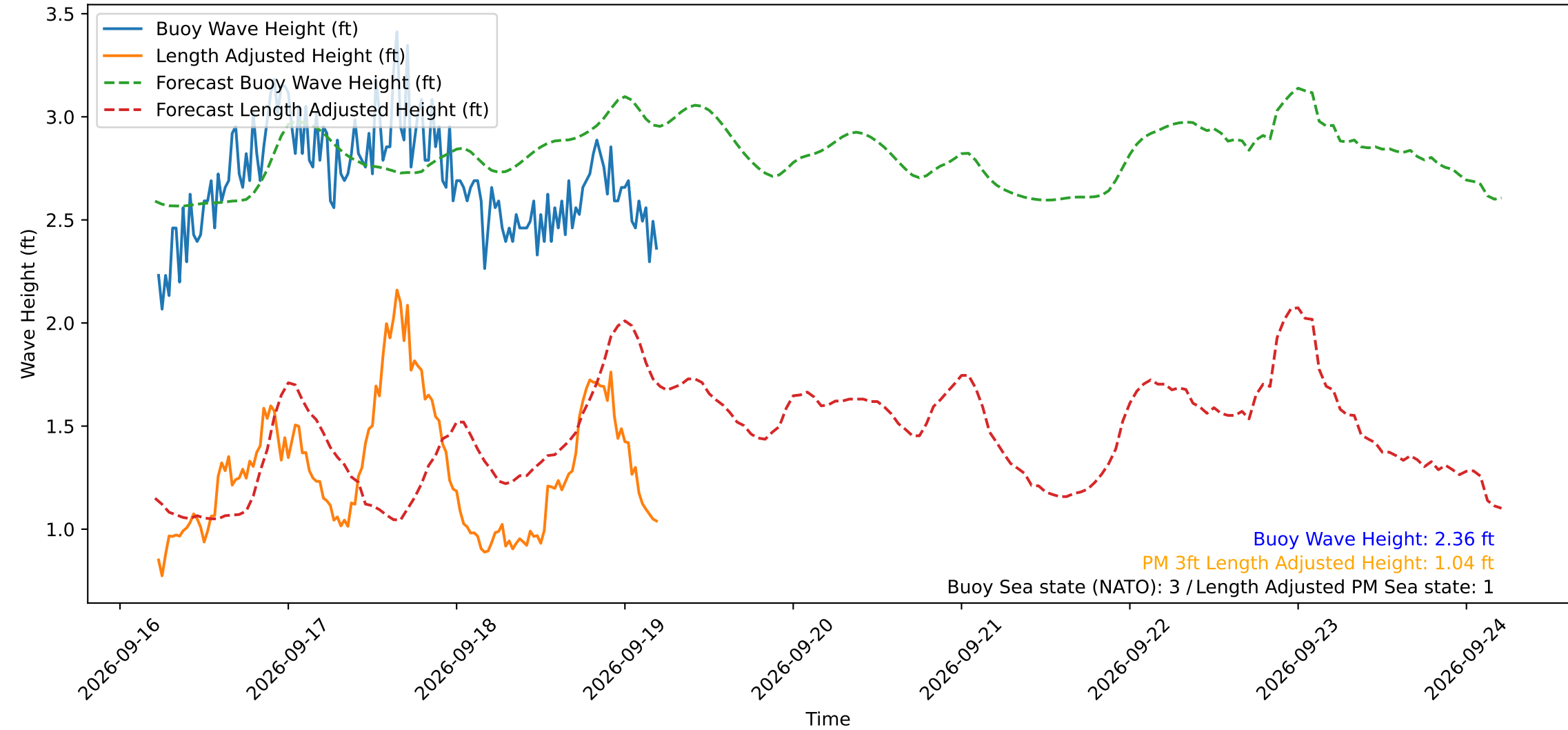
Wave Heights over Time for Red Beach at 2026-09-19 05:20:50
