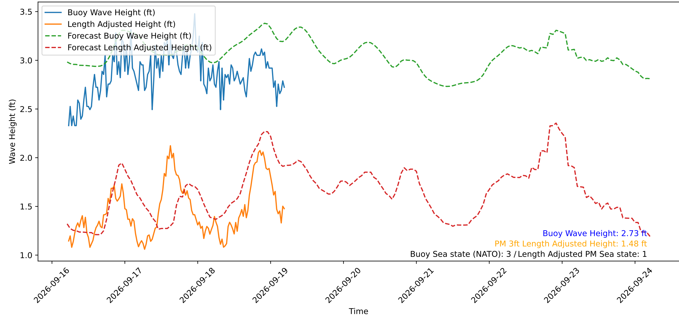
Wave Heights over Time for Green Beach at 2026-09-19 05:21:15
