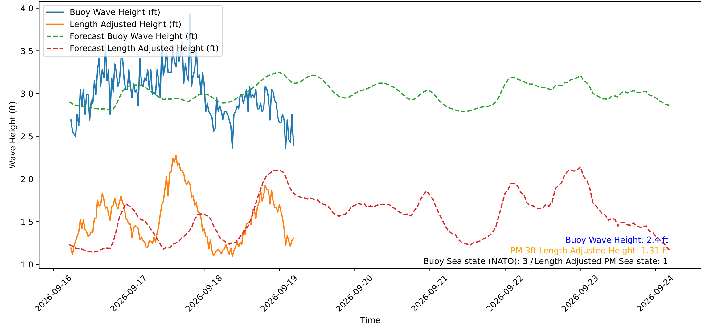
Wave Heights over Time for Oceanside Harbor at 2026-09-19 05:20:30
