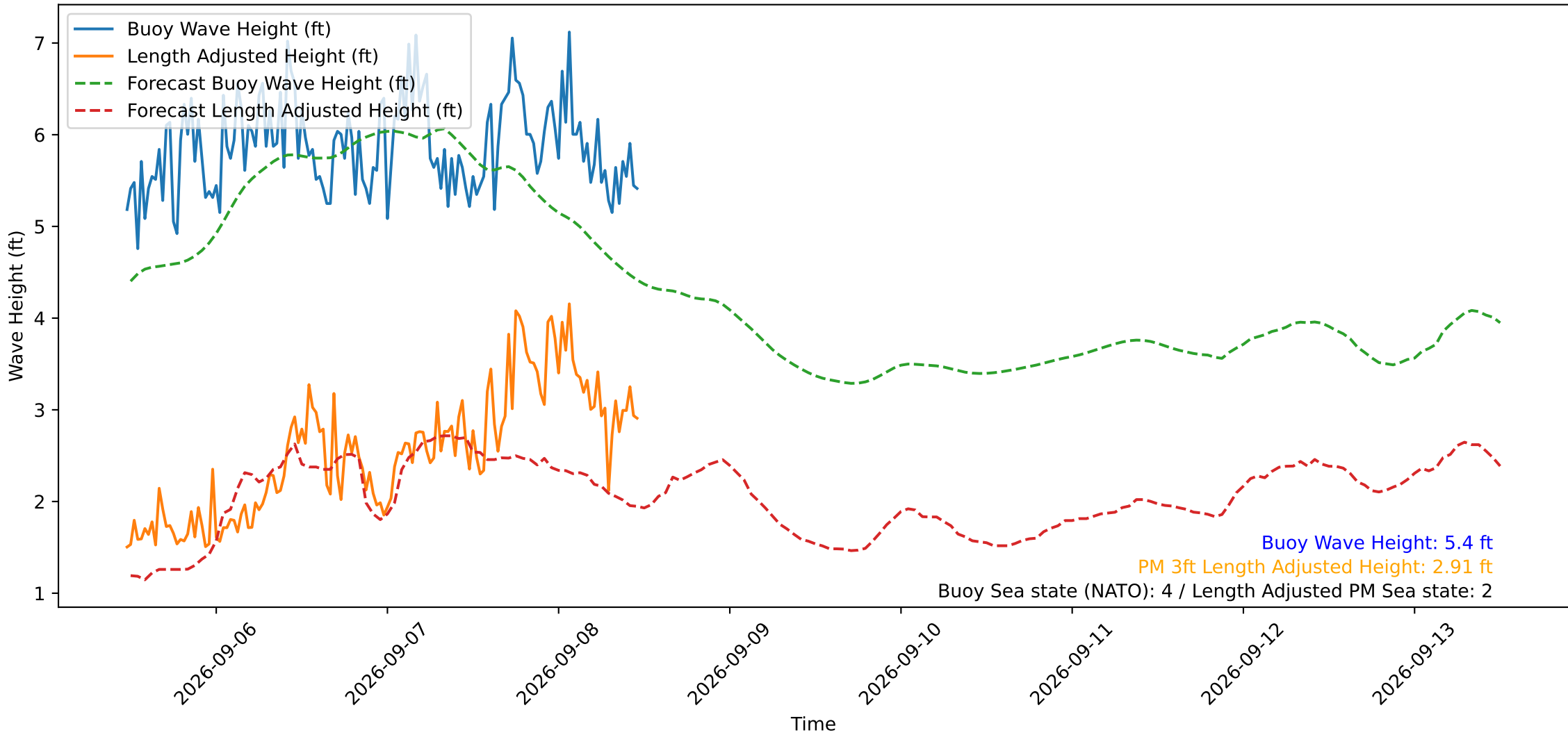
Wave Heights over Time for Oceanside Harbor at 2026-09-08 11:40:30
