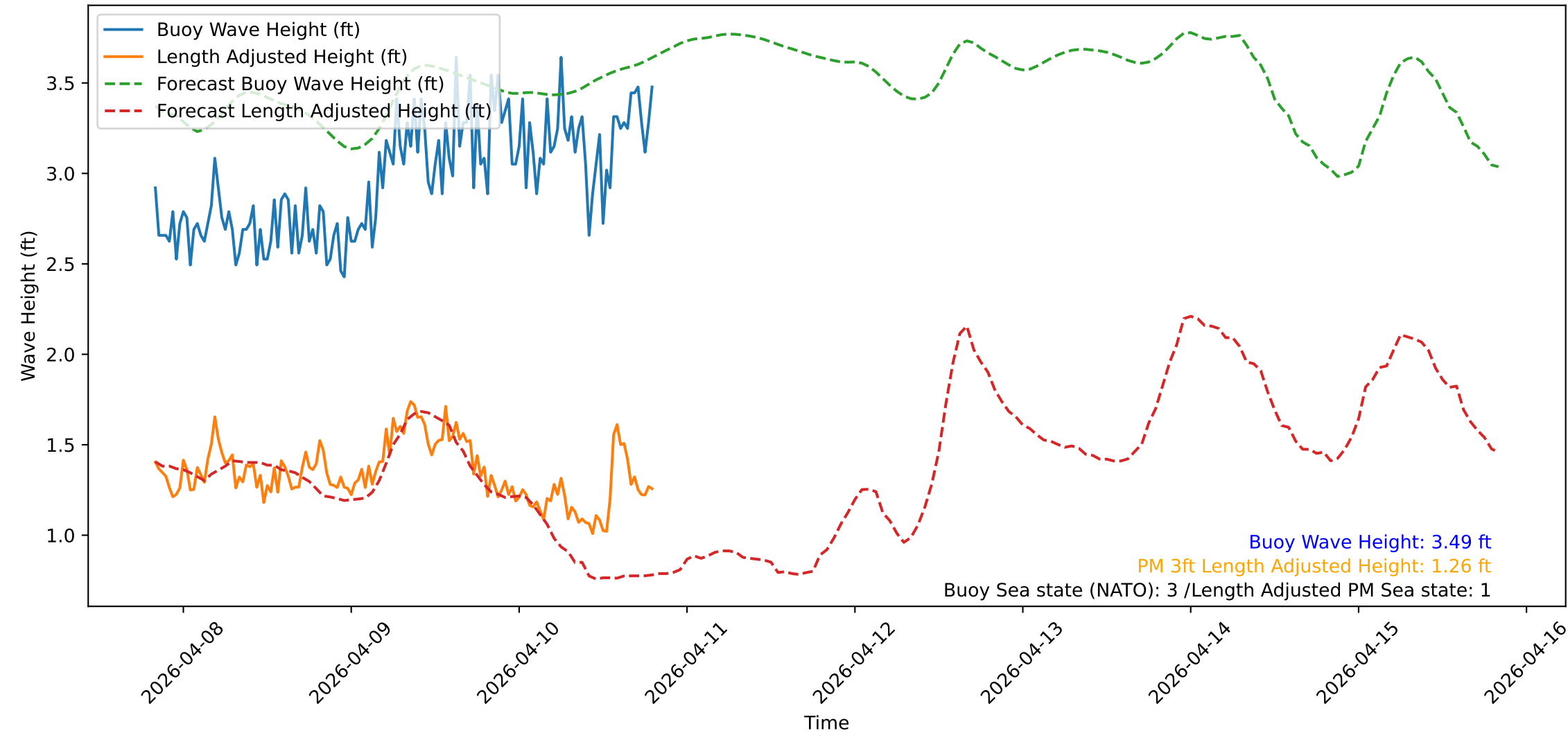
Wave Heights over Time for Oceanside Harbor at 2026-04-10 19:50:31
