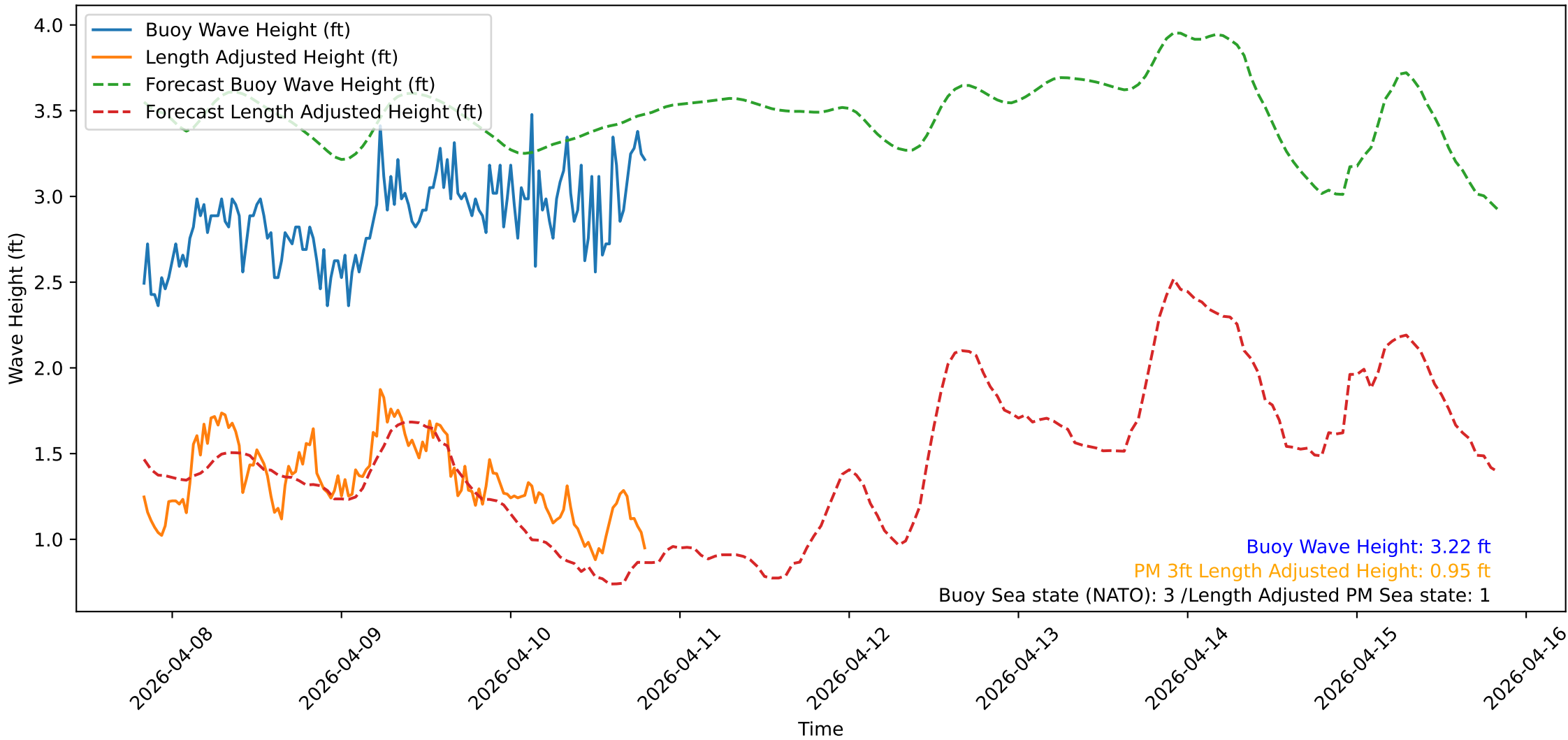
Wave Heights over Time for Green Beach at 2026-04-10 19:51:15
