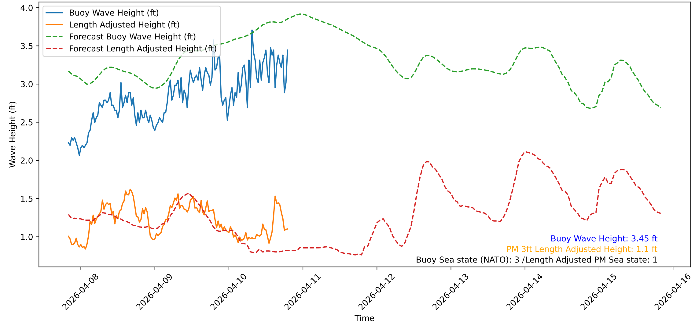
Wave Heights over Time for Red Beach at 2026-04-10 19:50:52
