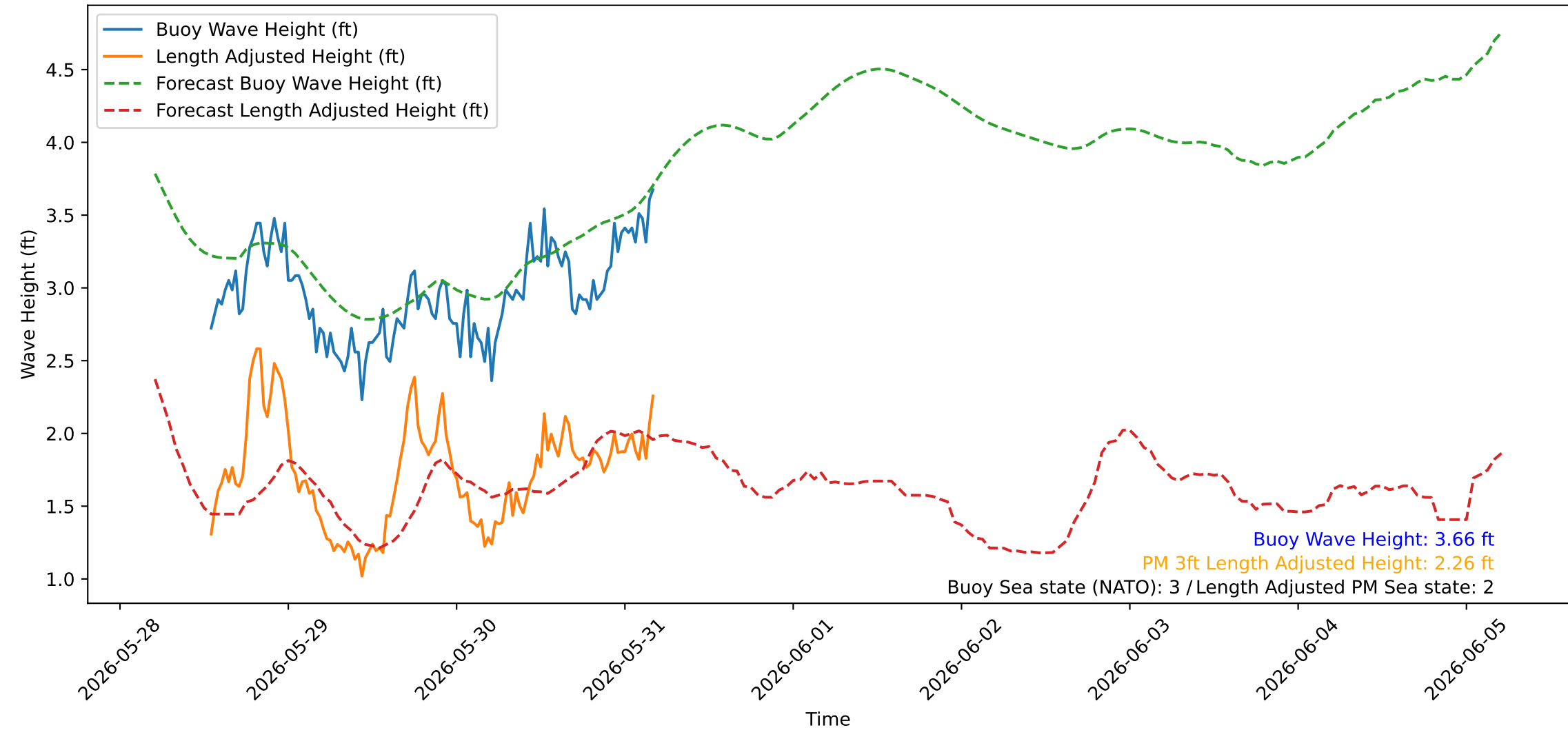
Wave Heights over Time for Oceanside Harbor at 2026-05-31 04:30:25
