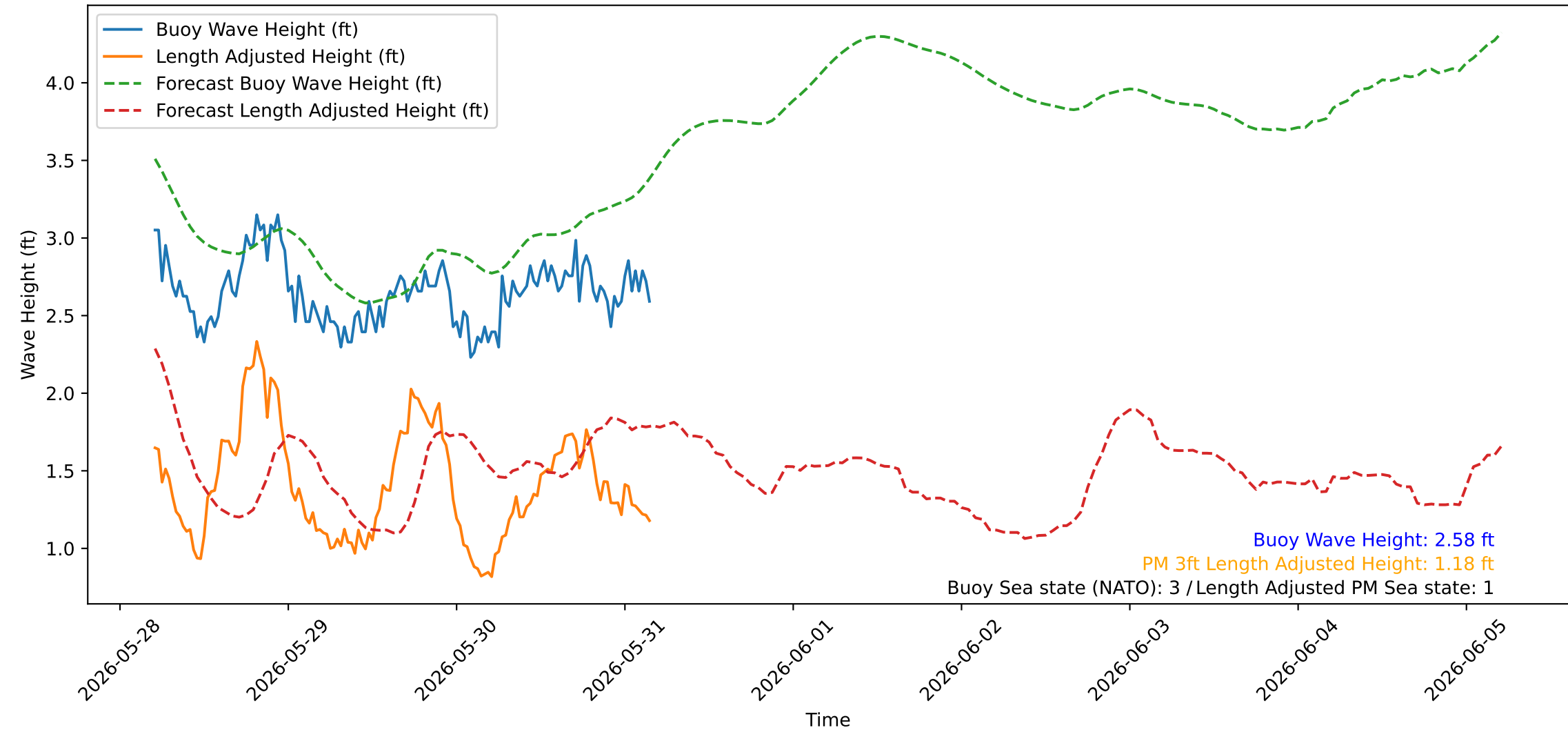
Wave Heights over Time for Red Beach at 2026-05-31 04:30:44
