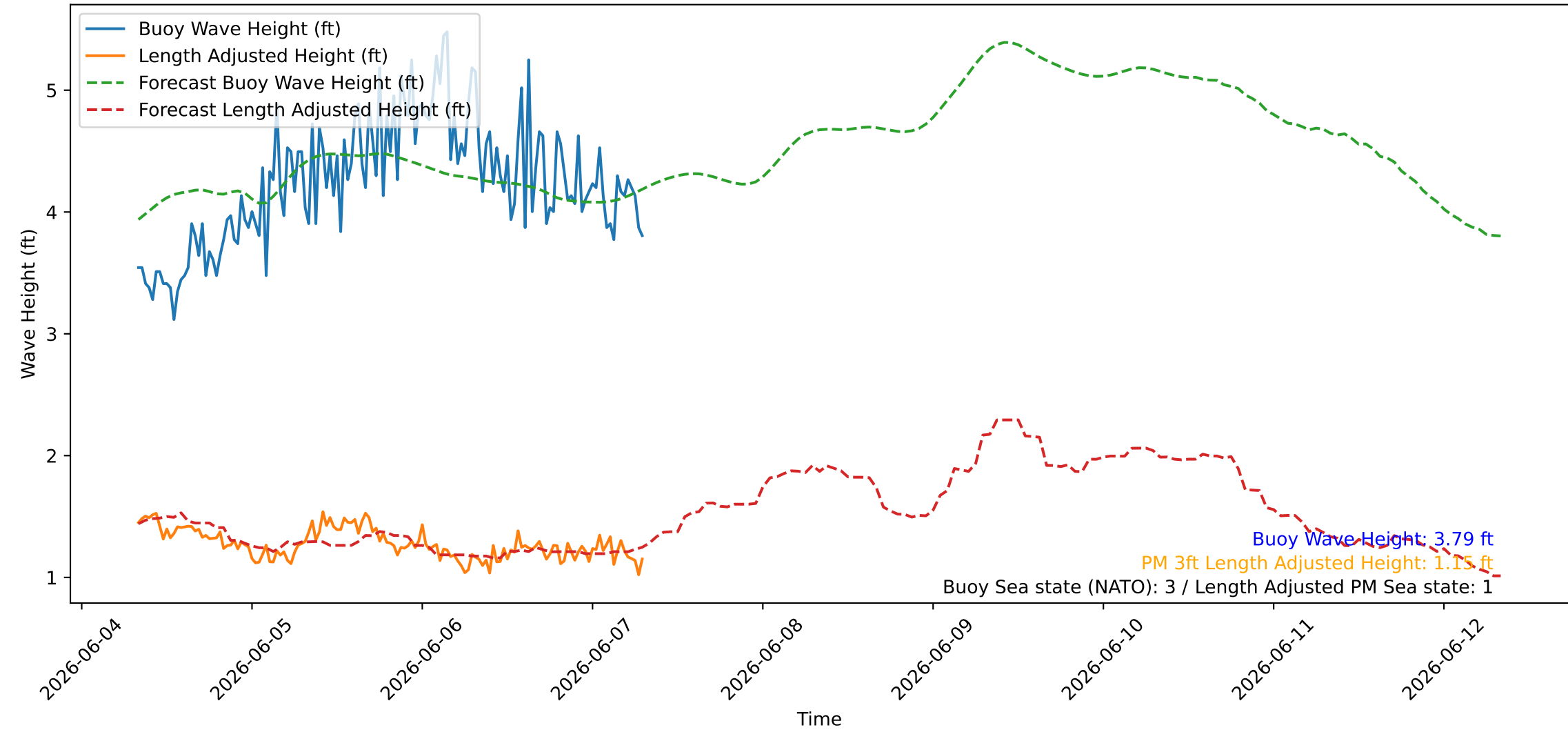
Wave Heights over Time for Oceanside Harbor at 2026-06-07 08:00:26
