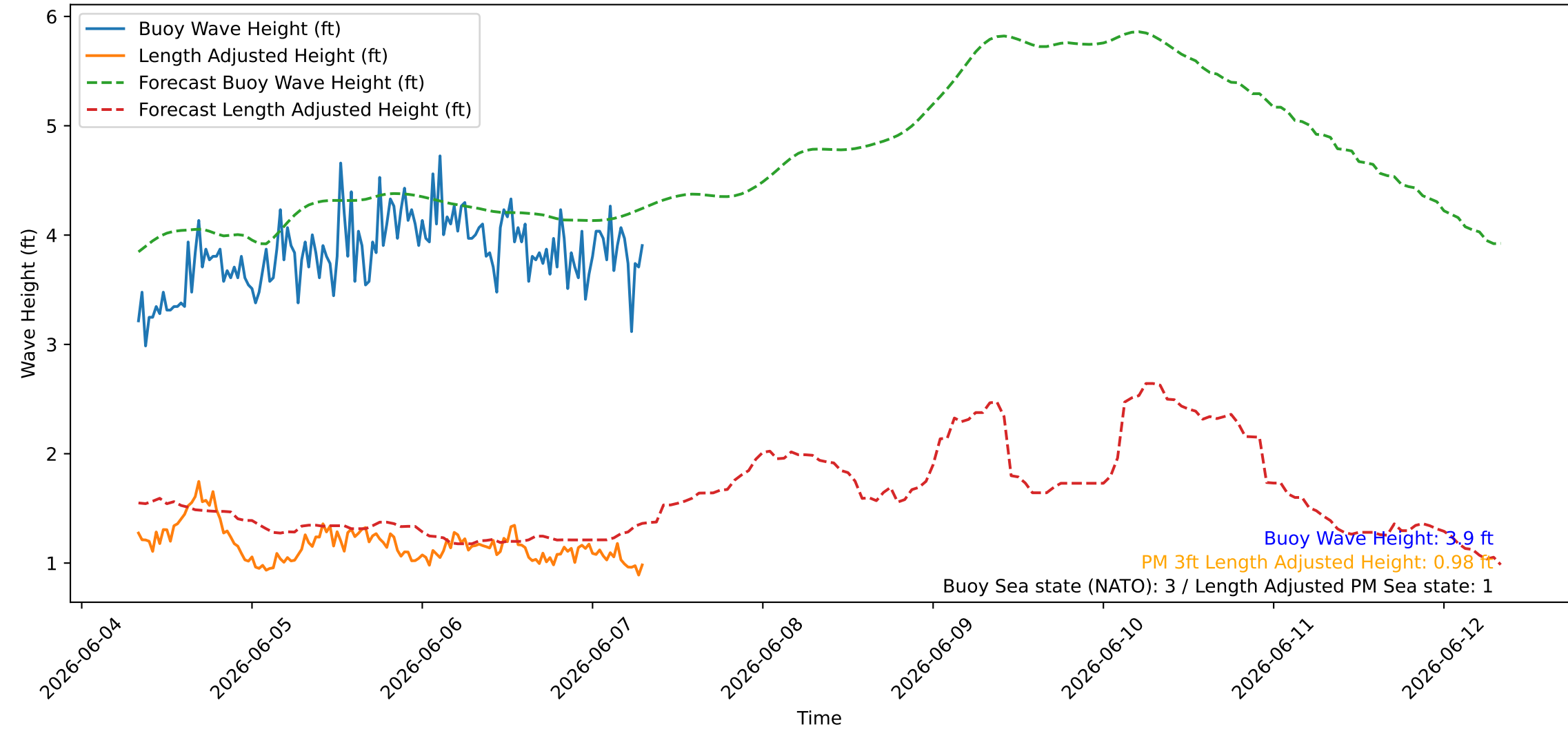
Wave Heights over Time for Green Beach at 2026-06-07 08:01:08
