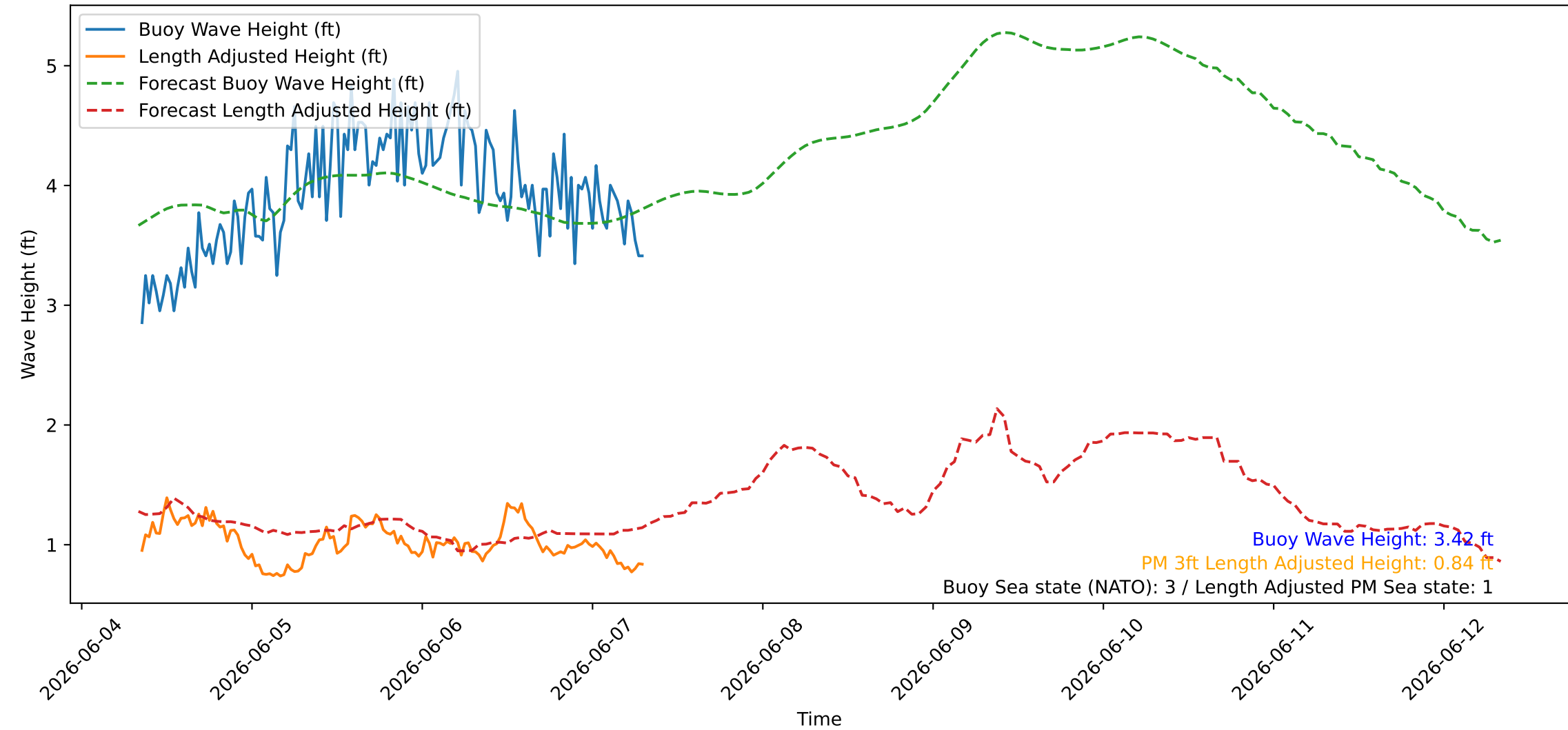
Wave Heights over Time for Red Beach at 2026-06-07 08:00:46
