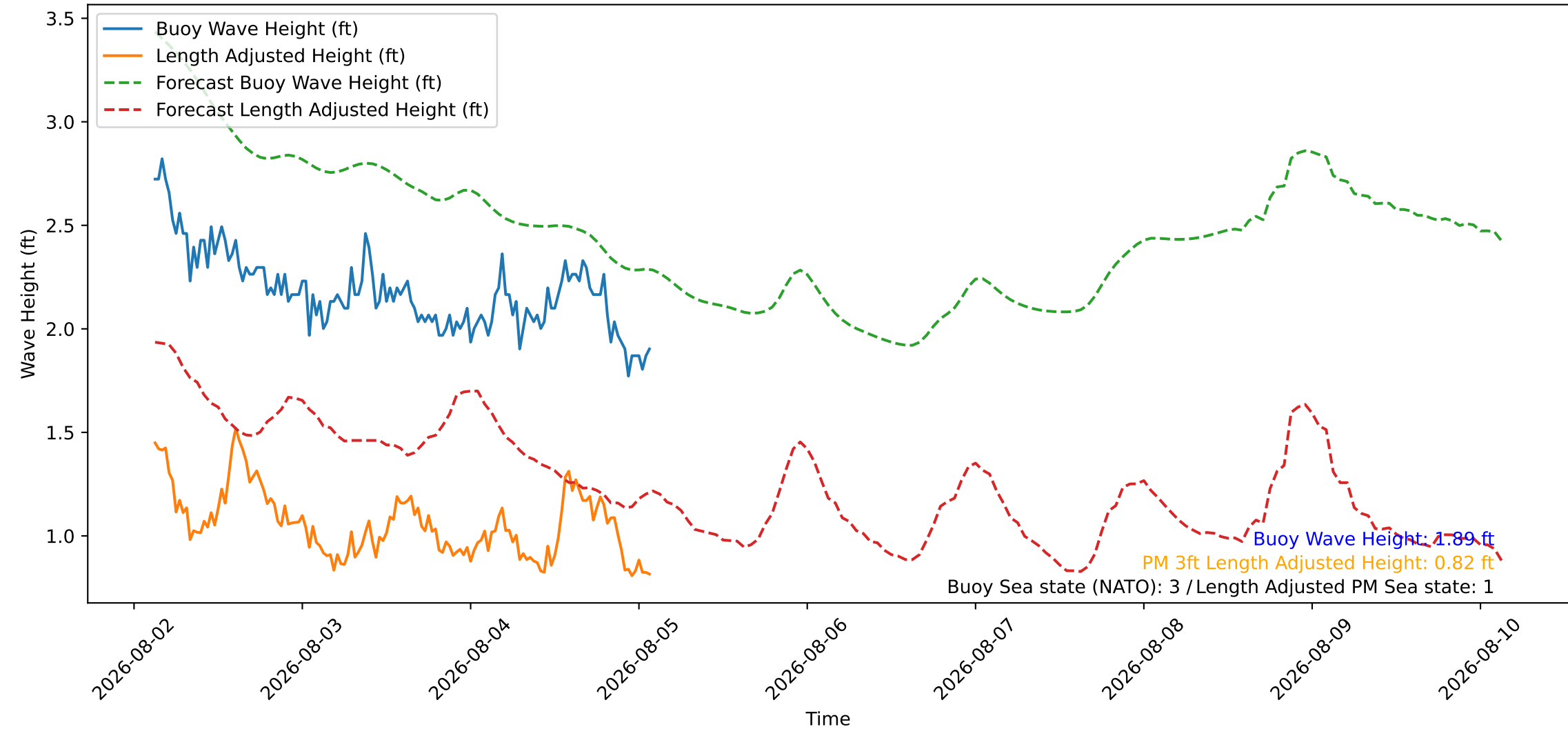
Wave Heights over Time for Red Beach at 2026-08-05 02:40:46
