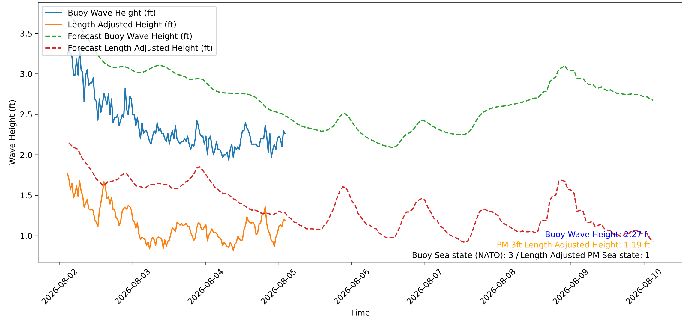
Wave Heights over Time for Green Beach at 2026-08-05 02:41:09
