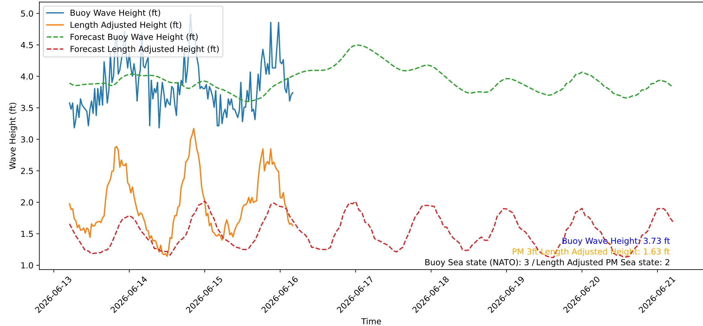
Wave Heights over Time for Oceanside Harbor at 2026-06-16 04:50:26
