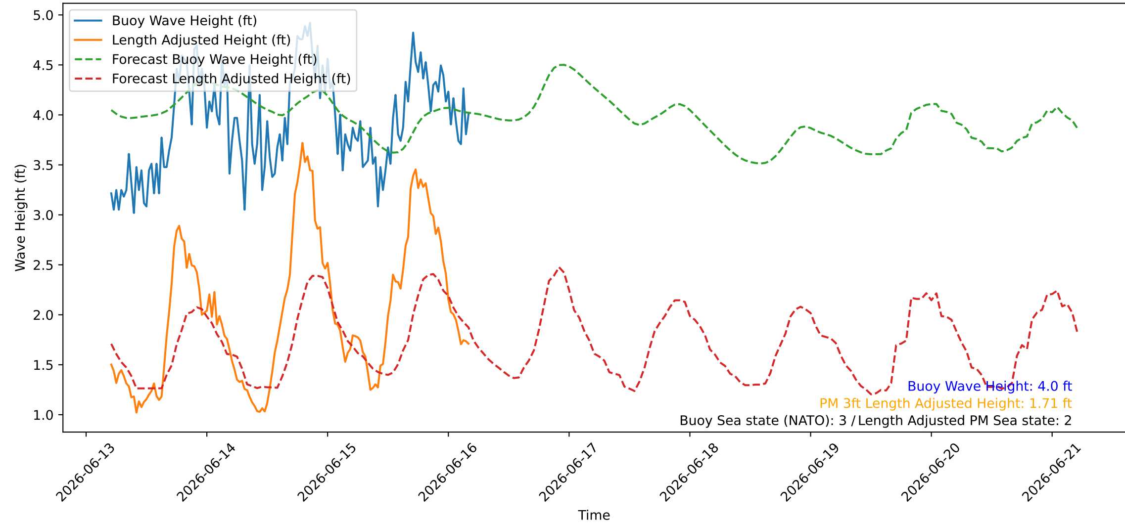
Wave Heights over Time for Green Beach at 2026-06-16 04:51:09
