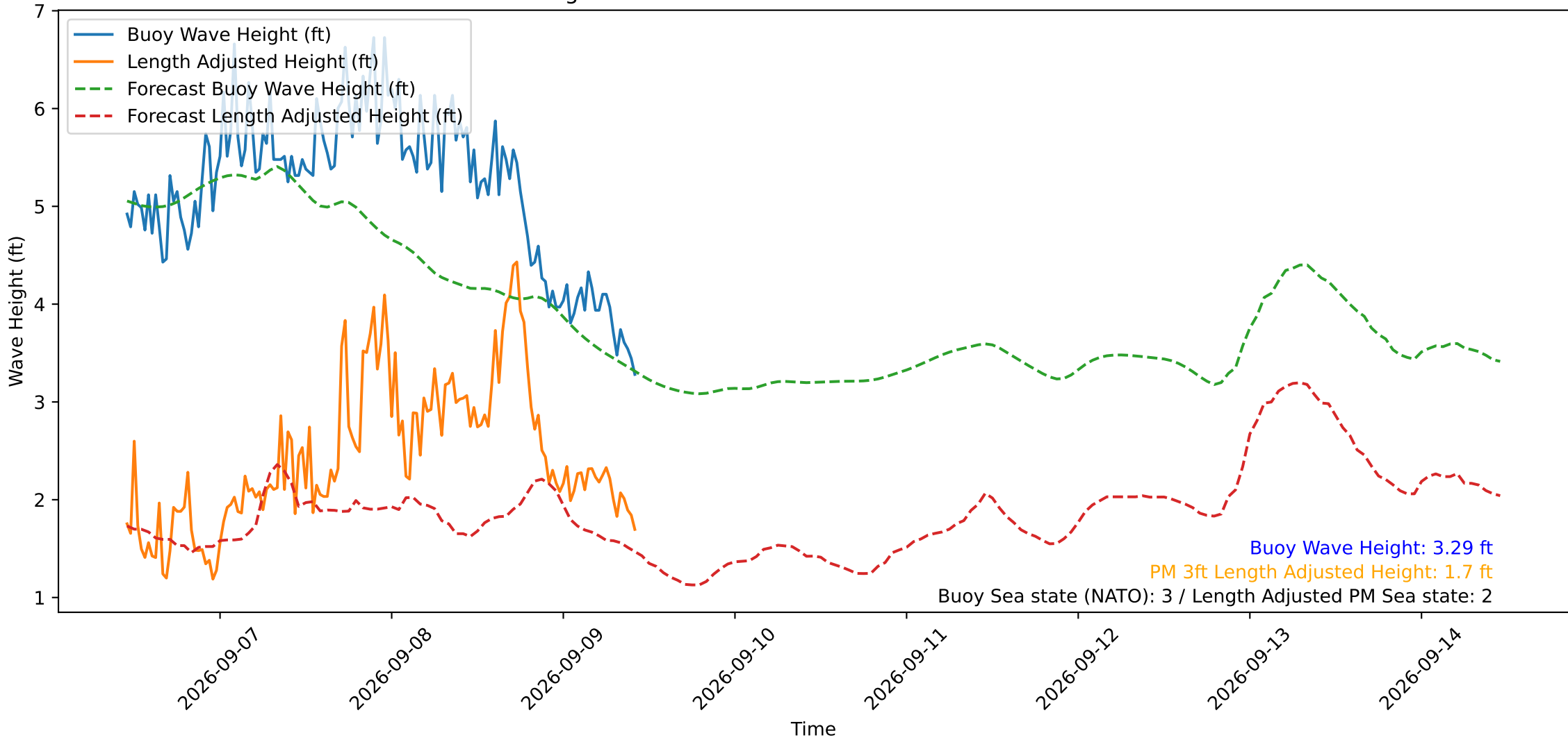
Wave Heights over Time for Red Beach at 2026-09-09 10:50:51
