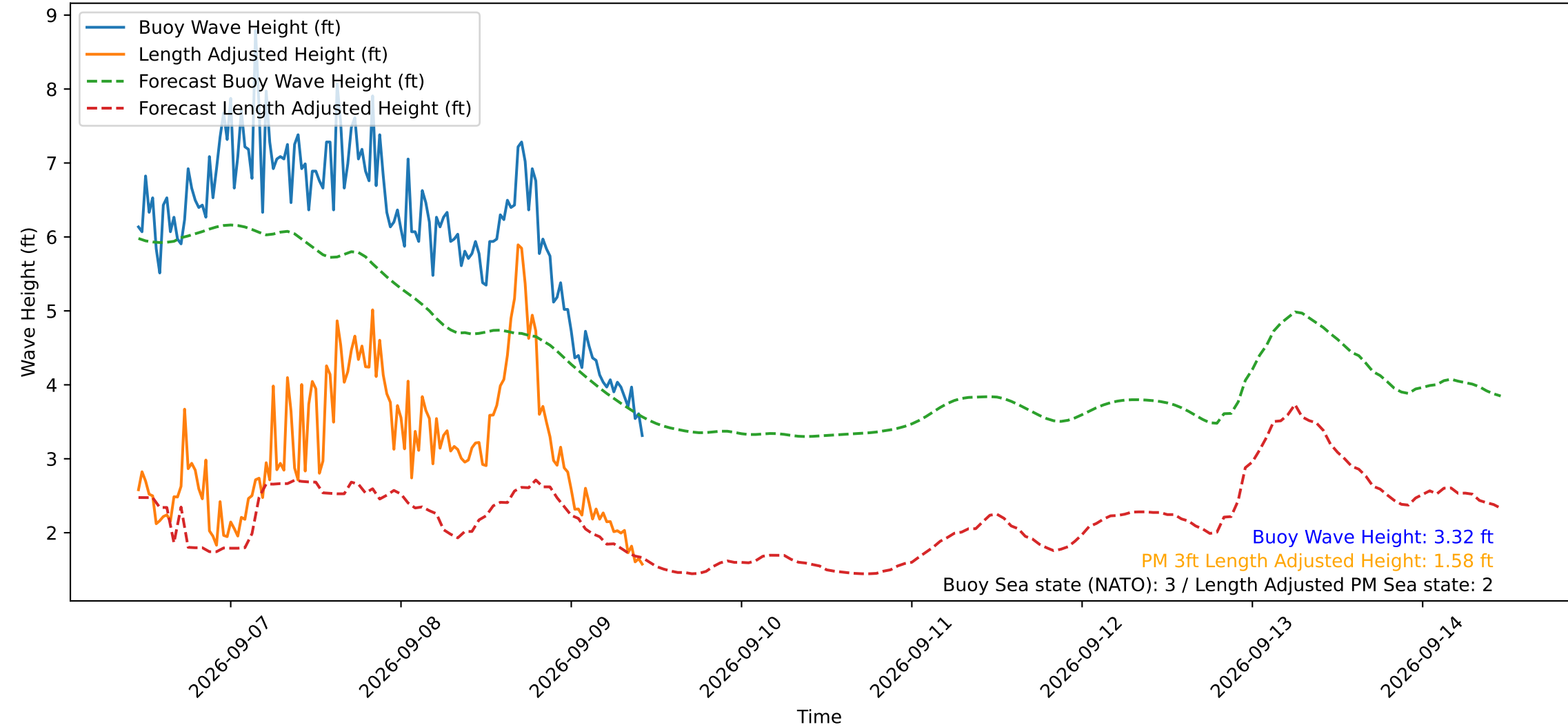
Wave Heights over Time for Green Beach at 2026-09-09 10:51:14
