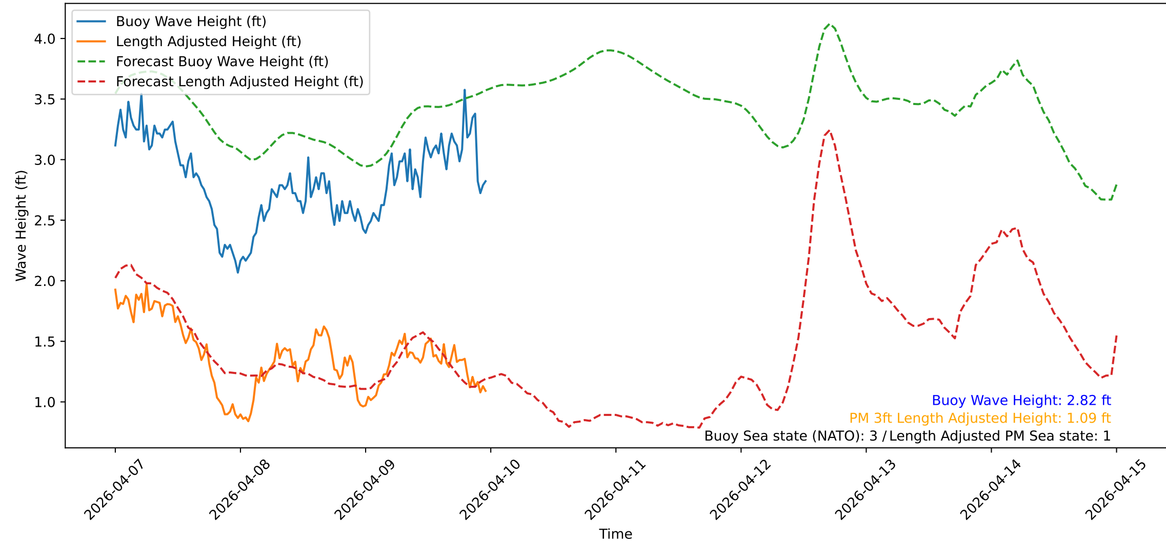
Wave Heights over Time for Red Beach at 2026-04-09 23:40:47
