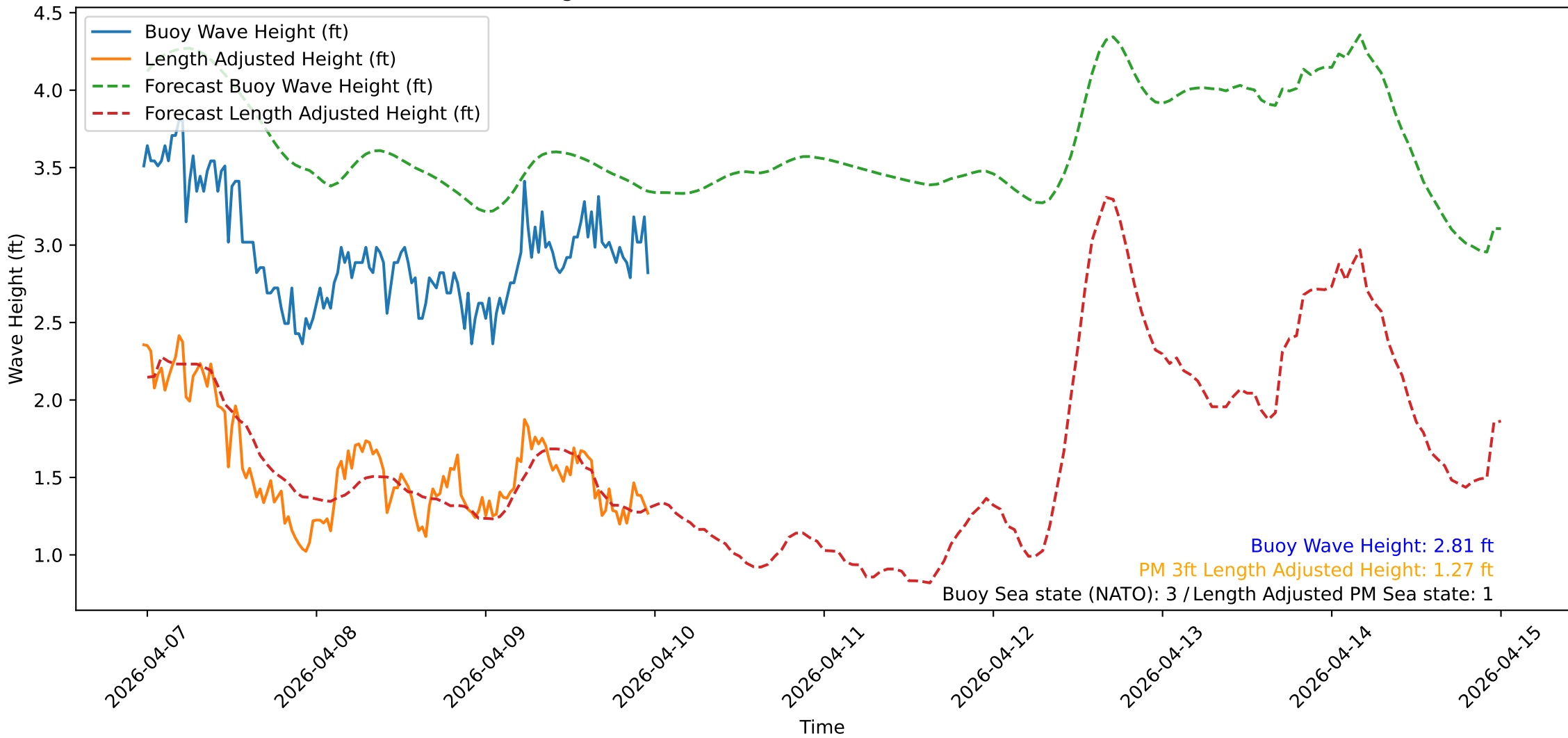
Wave Heights over Time for Green Beach at 2026-04-09 23:41:09
