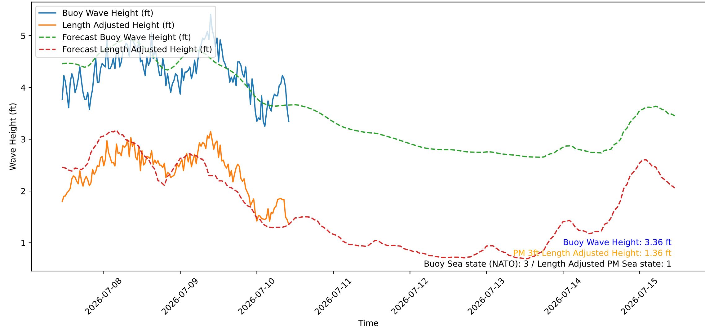
Wave Heights over Time for Oceanside Harbor at 2026-07-10 10:50:27
