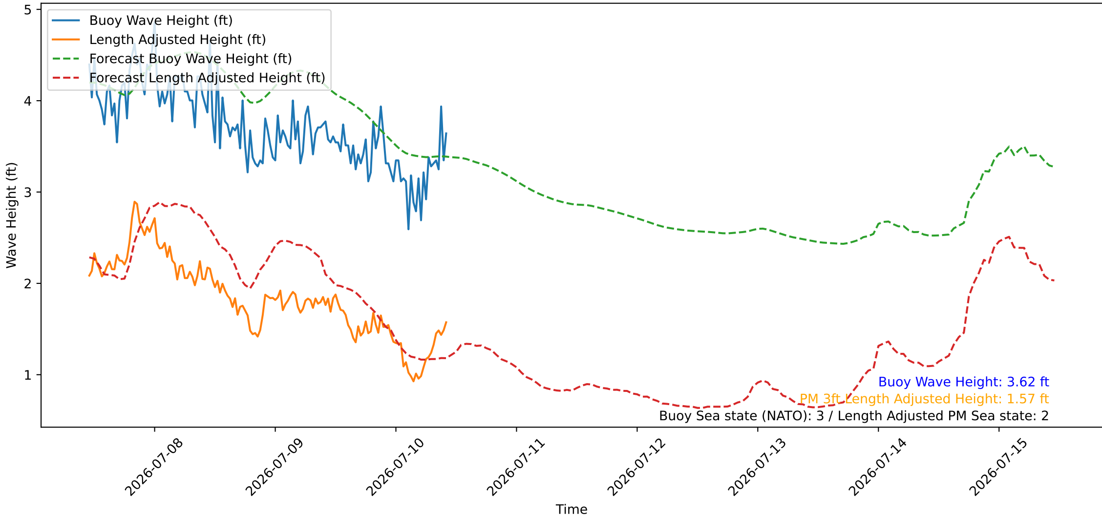
Wave Heights over Time for Red Beach at 2026-07-10 10:50:47
