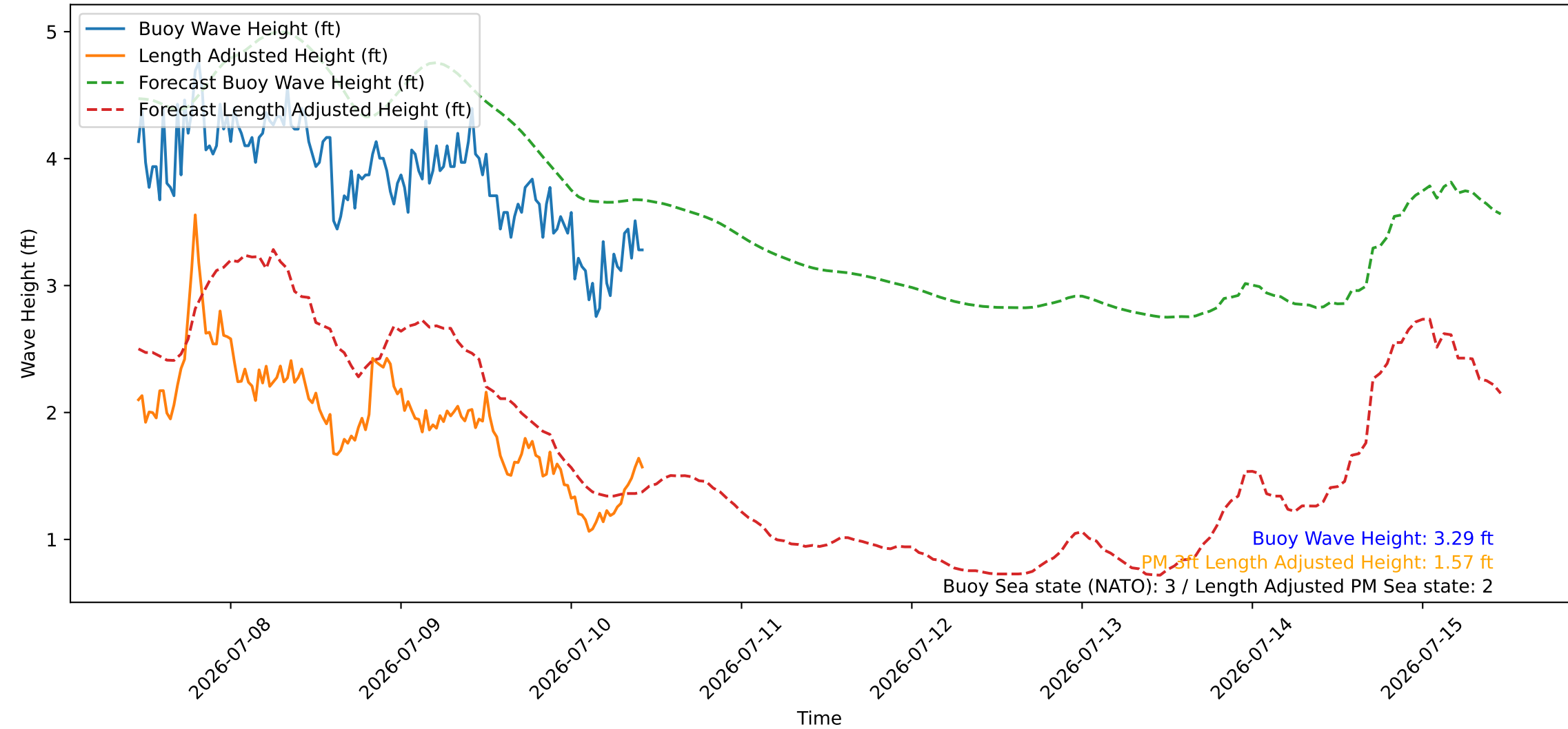
Wave Heights over Time for Green Beach at 2026-07-10 10:51:09
