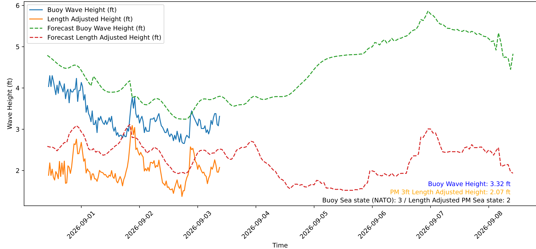
Wave Heights over Time for Green Beach at 2026-09-03 10:01:12
