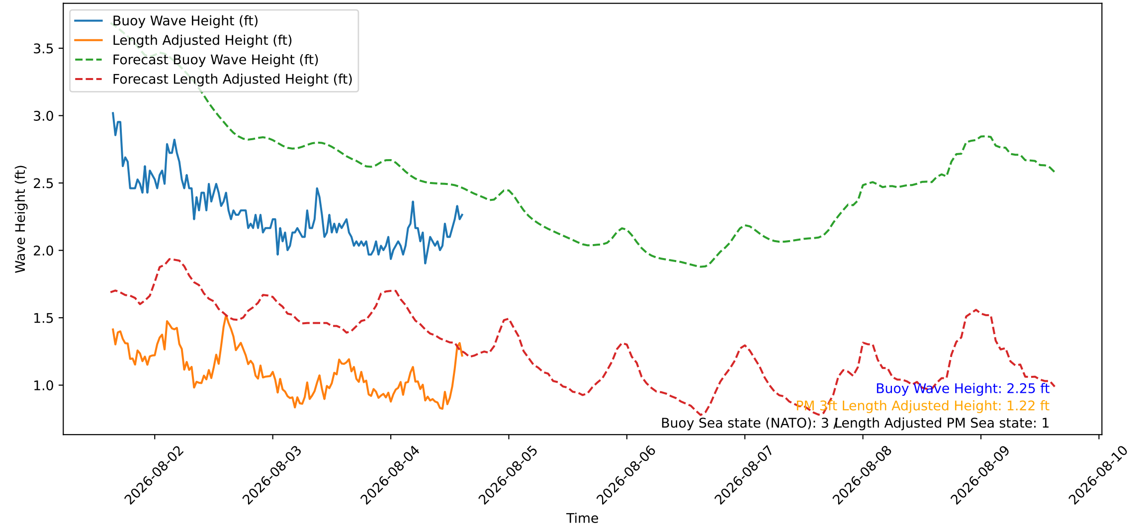
Wave Heights over Time for Red Beach at 2026-08-04 15:20:47
