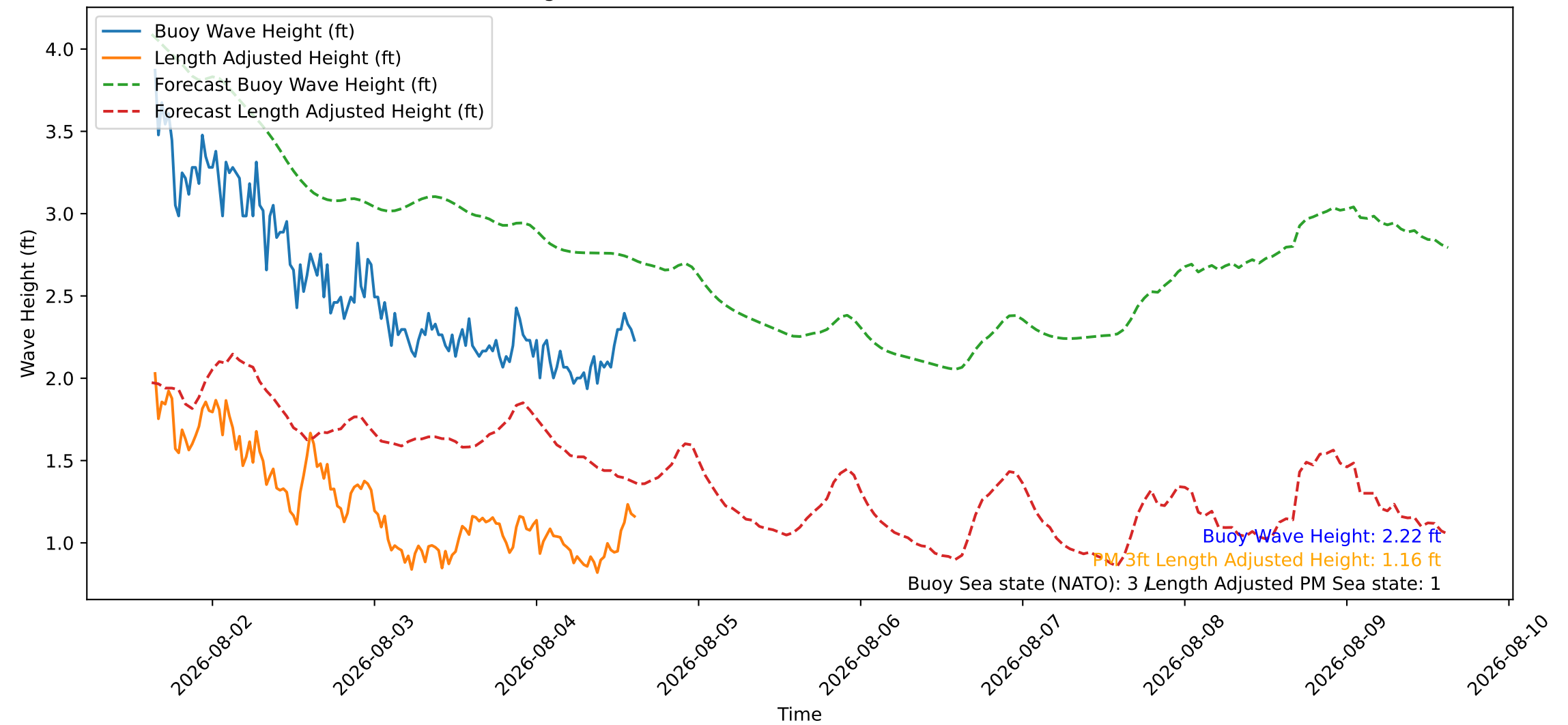
Wave Heights over Time for Green Beach at 2026-08-04 15:21:09
