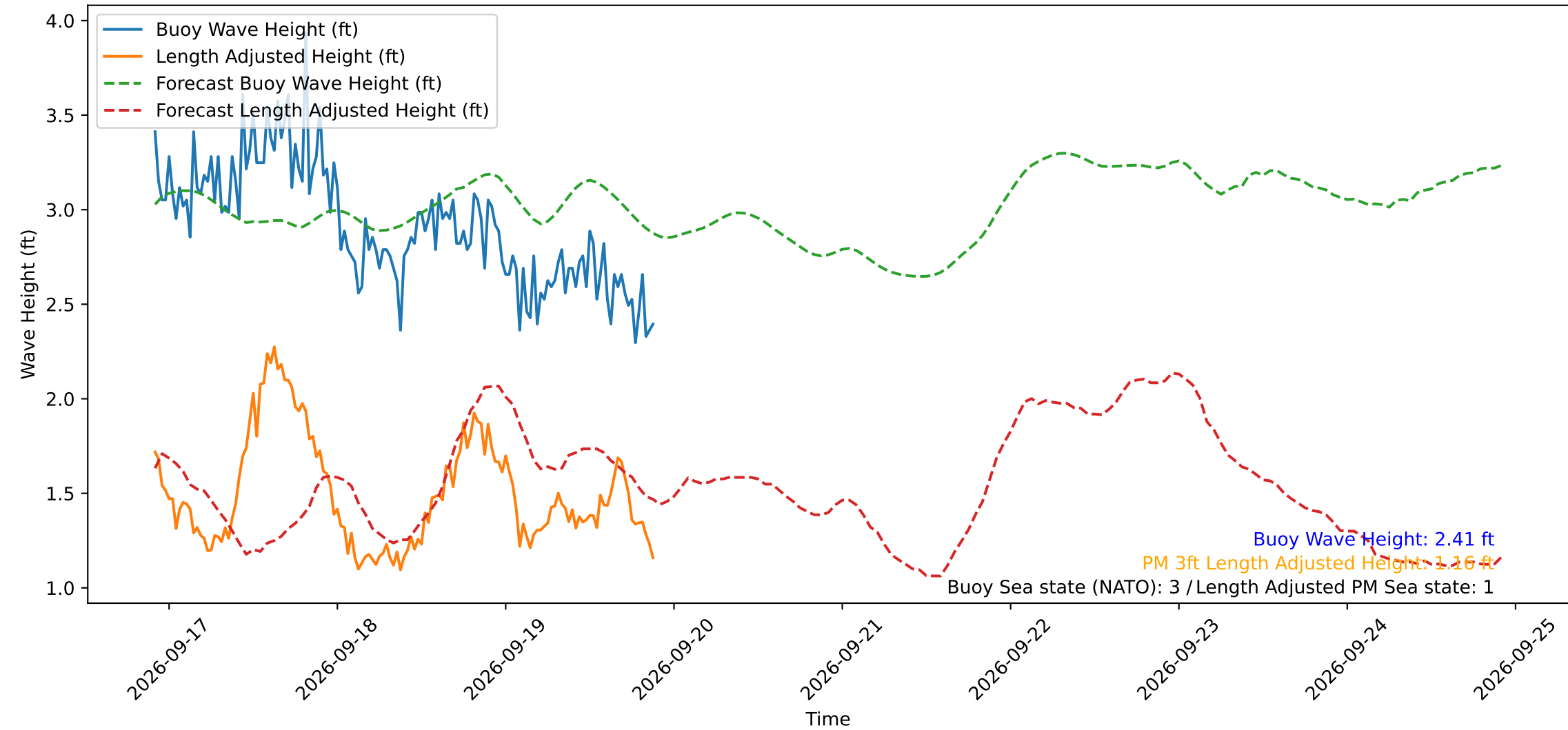
Wave Heights over Time for Oceanside Harbor at 2026-09-19 22:00:29
