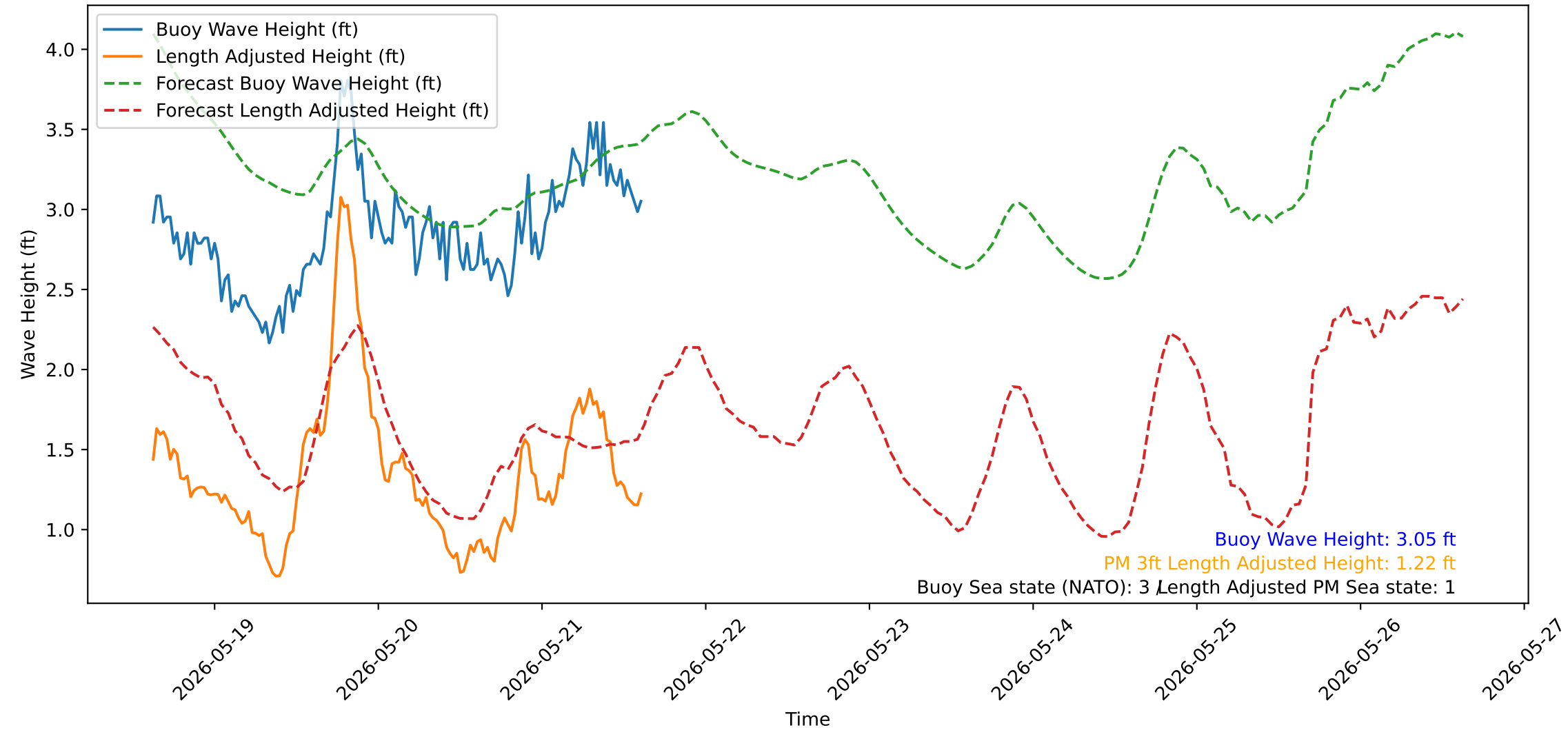
Wave Heights over Time for Green Beach at 2026-05-21 15:11:13
