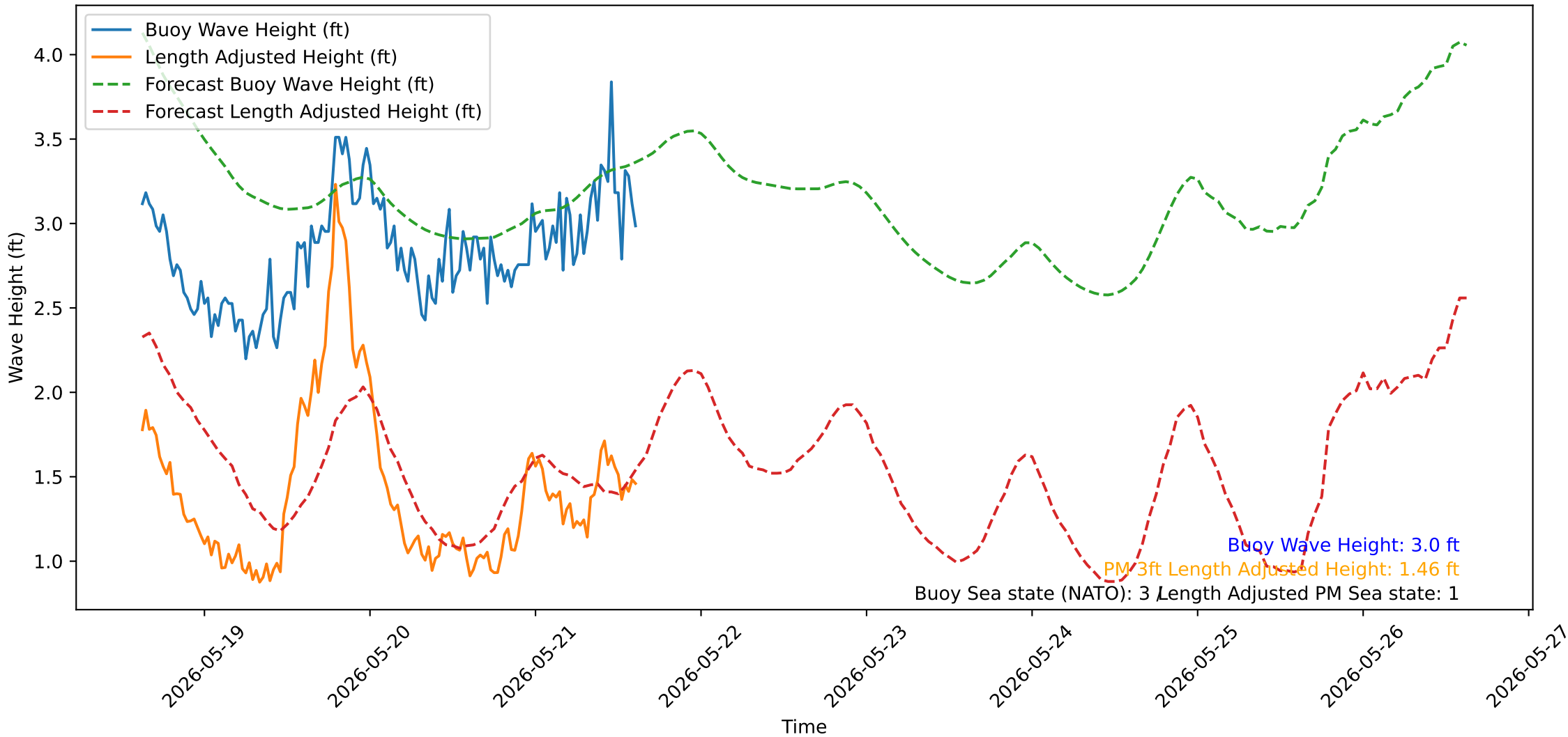
Wave Heights over Time for Oceanside Harbor at 2026-05-21 15:10:31
