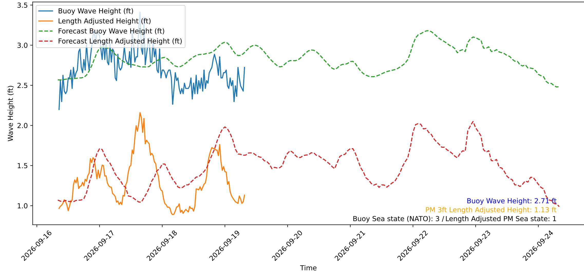
Wave Heights over Time for Red Beach at 2026-09-19 08:20:49
