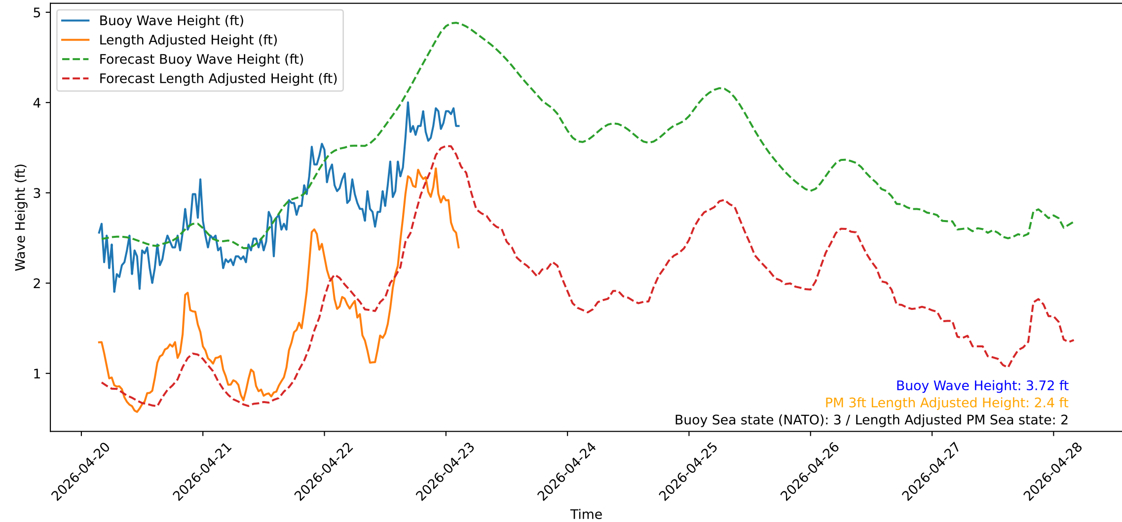
Wave Heights over Time for Green Beach at 2026-04-23 03:41:13
