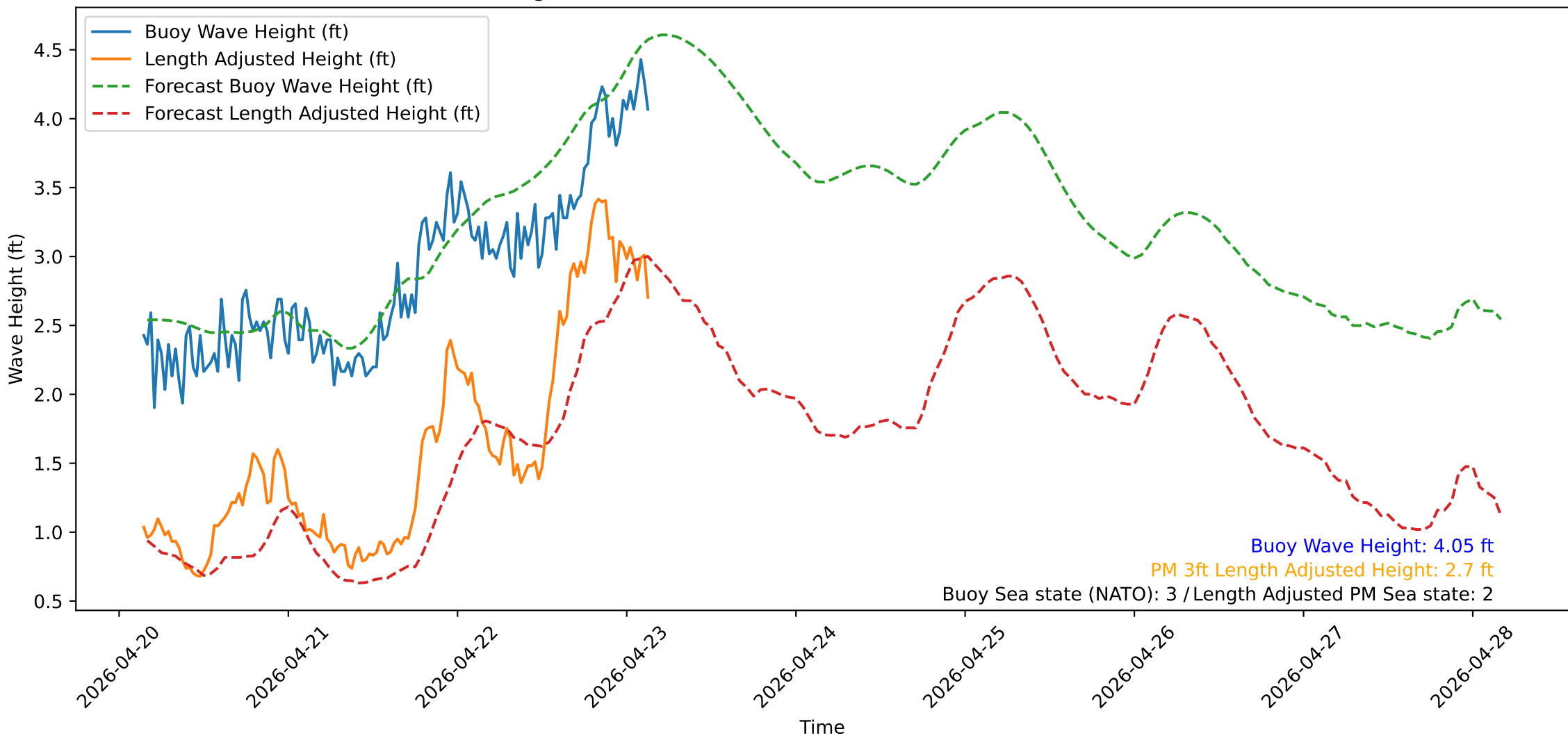
Wave Heights over Time for Oceanside Harbor at 2026-04-23 03:40:32
