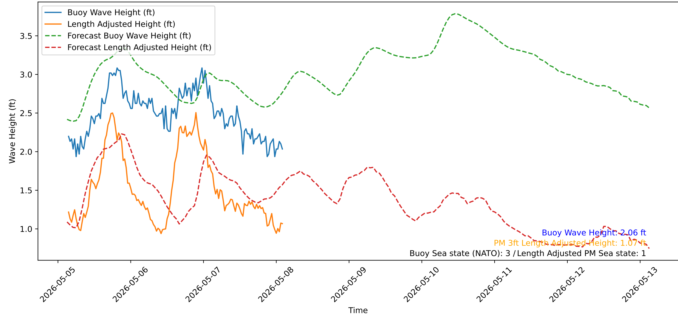
Wave Heights over Time for Red Beach at 2026-05-08 03:00:49
