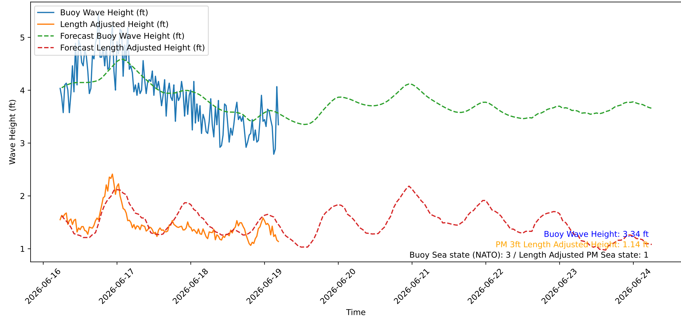
Wave Heights over Time for Oceanside Harbor at 2026-06-19 05:30:27
