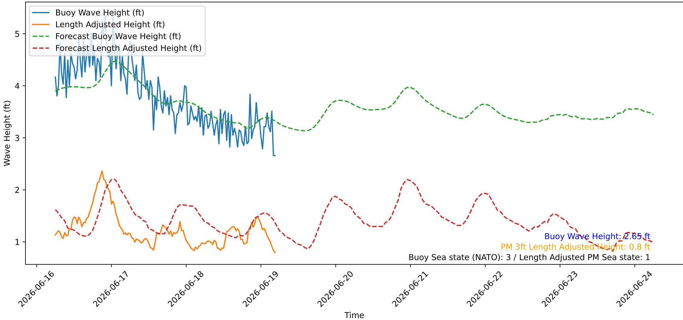
Wave Heights over Time for Red Beach at 2026-06-19 05:30:45
