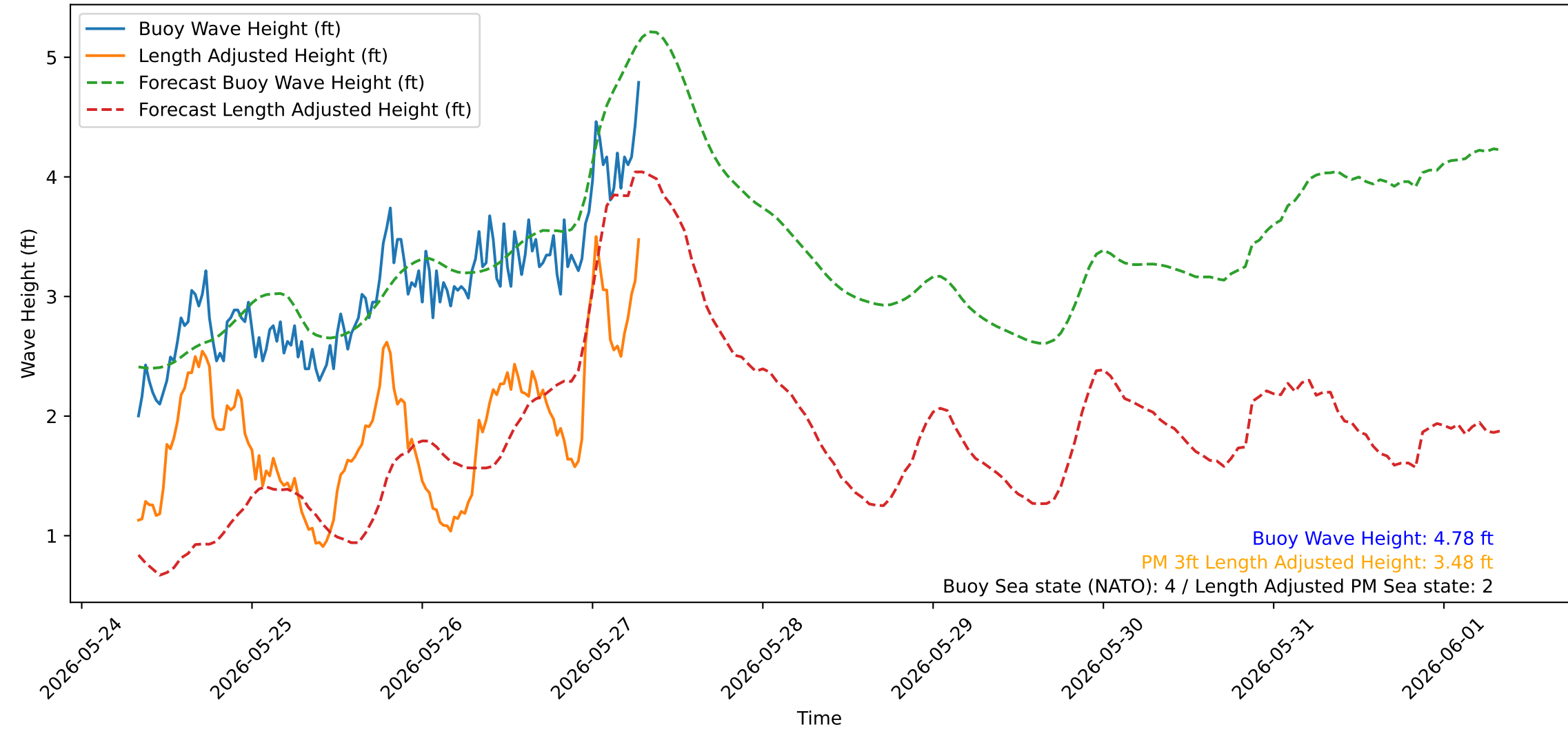
Wave Heights over Time for Red Beach at 2026-05-27 07:30:45
