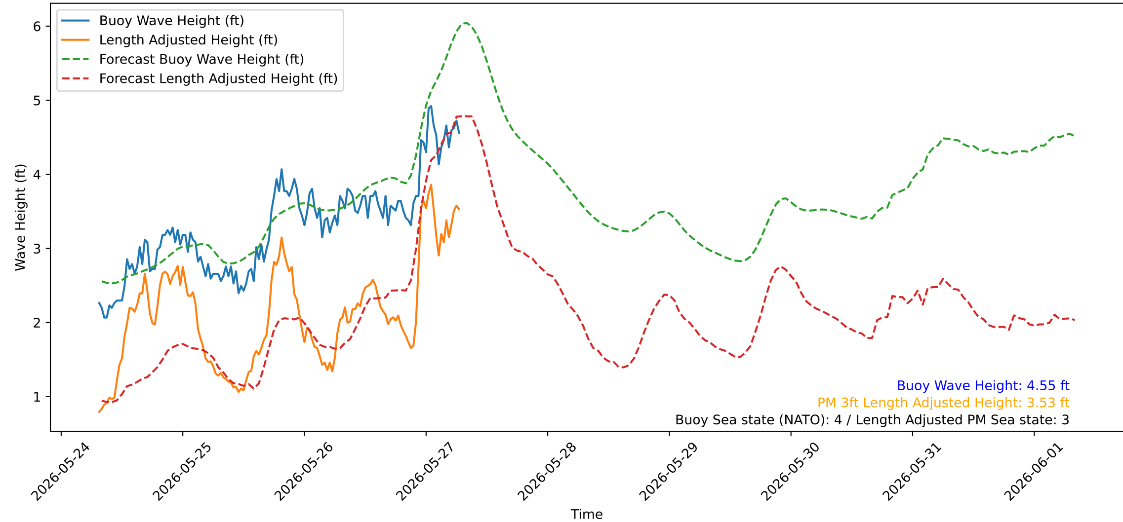
Wave Heights over Time for Green Beach at 2026-05-27 07:31:08
