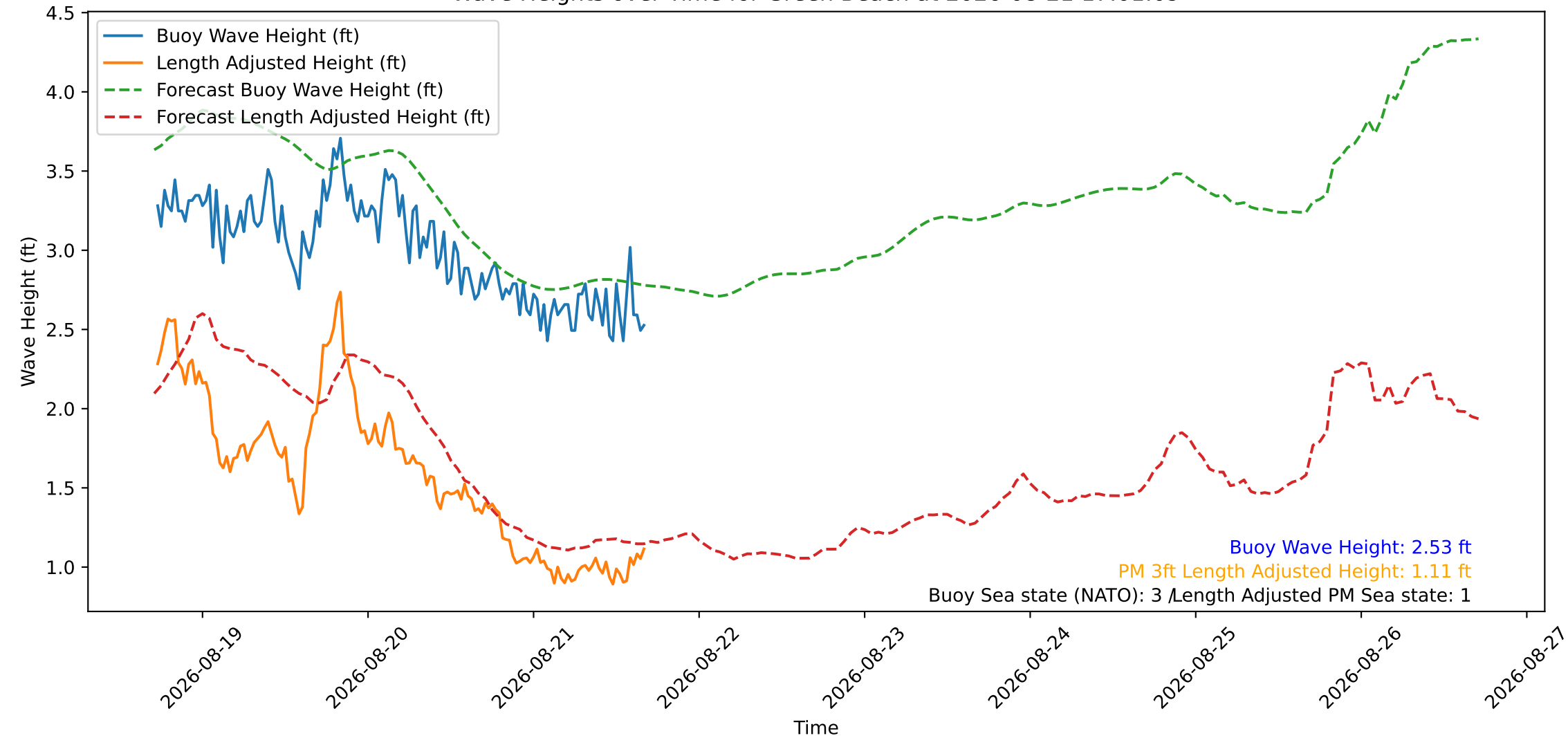
Wave Heights over Time for Green Beach at 2026-08-21 17:01:09
