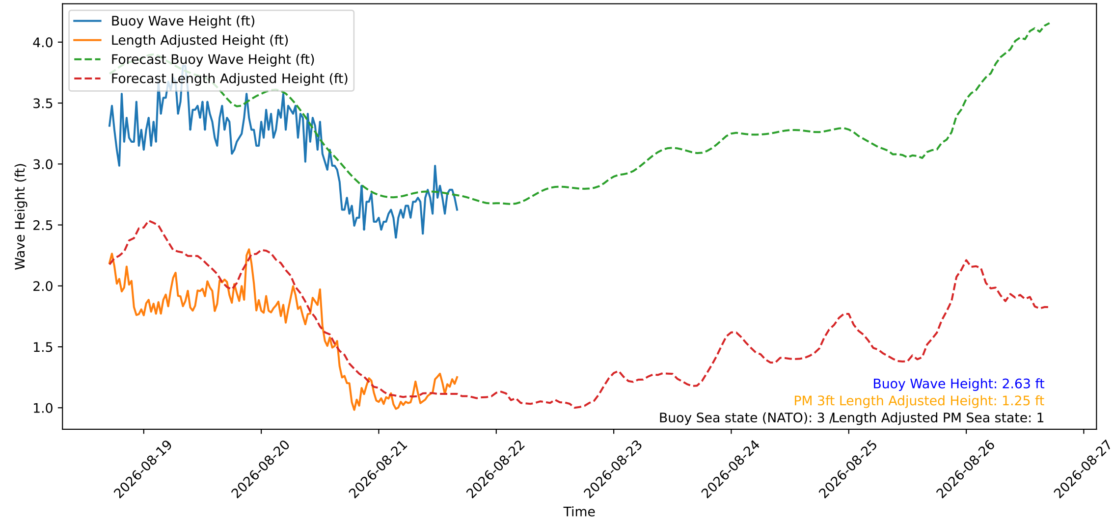
Wave Heights over Time for Oceanside Harbor at 2026-08-21 17:00:26
