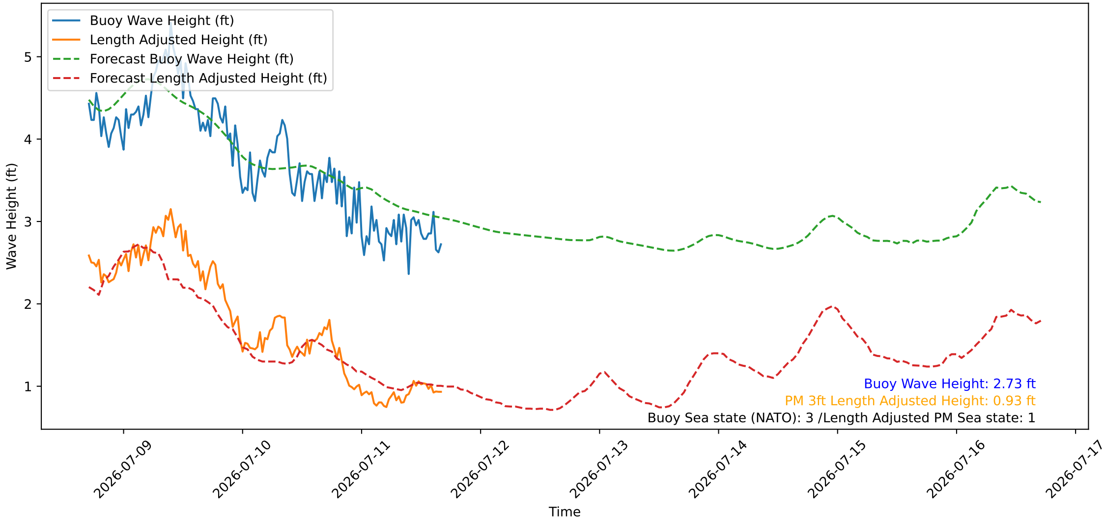
Wave Heights over Time for Oceanside Harbor at 2026-07-11 16:50:27
