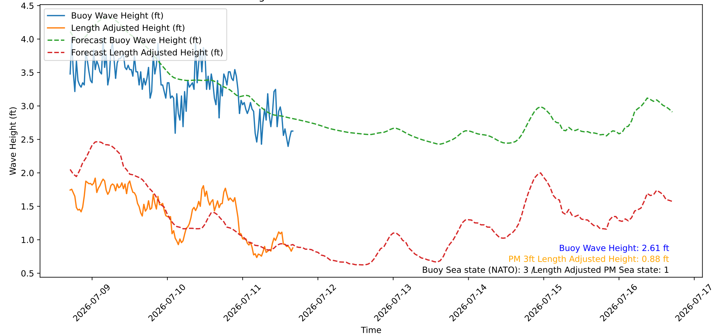
Wave Heights over Time for Red Beach at 2026-07-11 16:50:48
