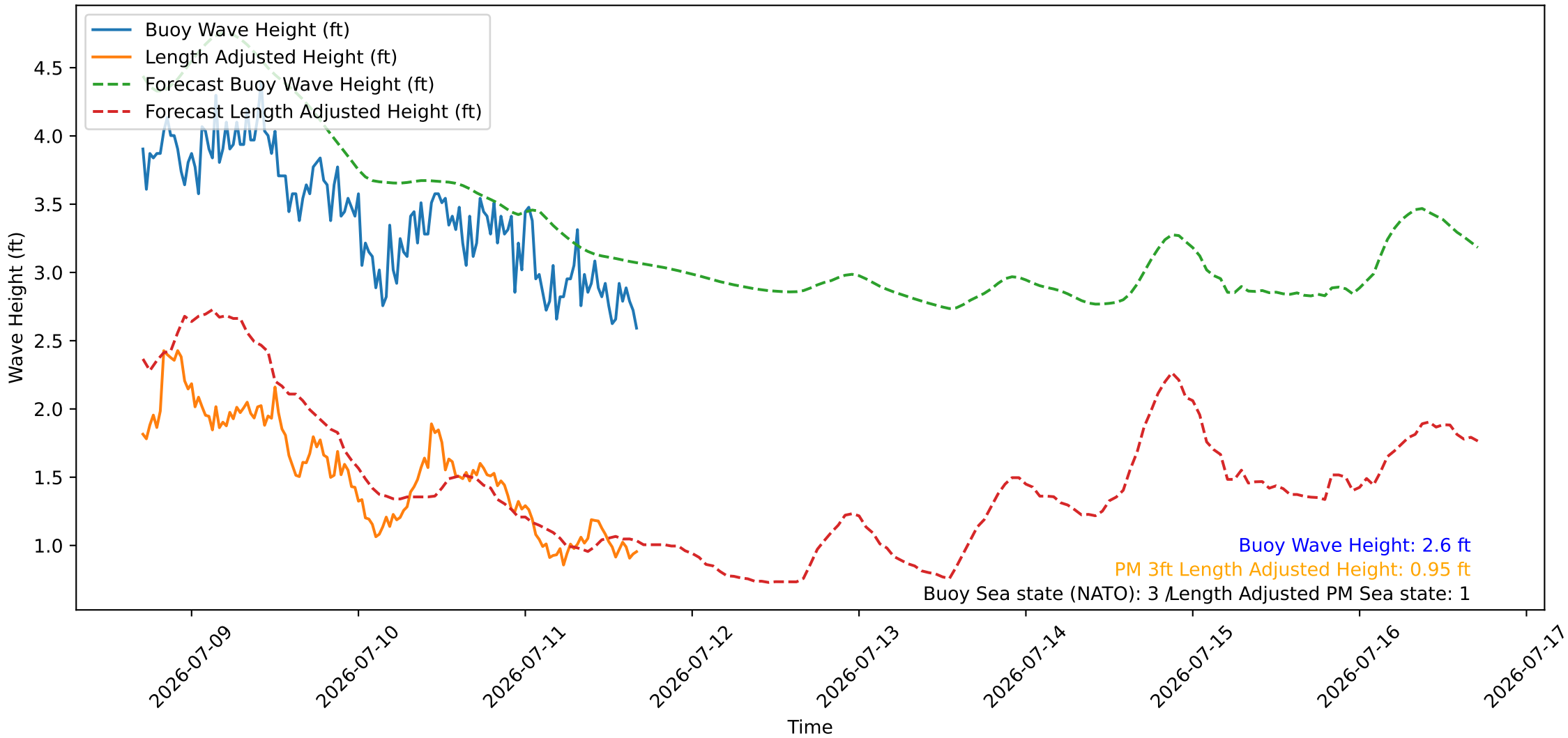
Wave Heights over Time for Green Beach at 2026-07-11 16:51:10
