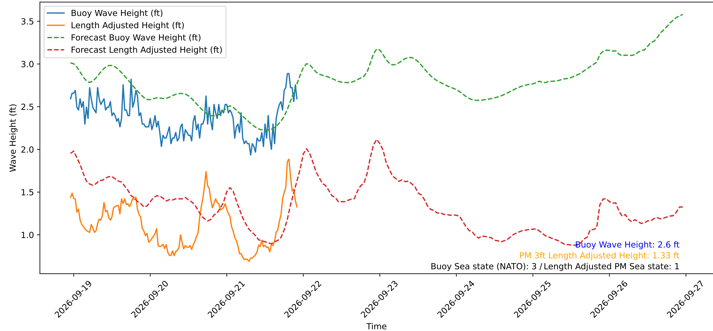
Wave Heights over Time for Red Beach at 2026-09-21 22:40:49
