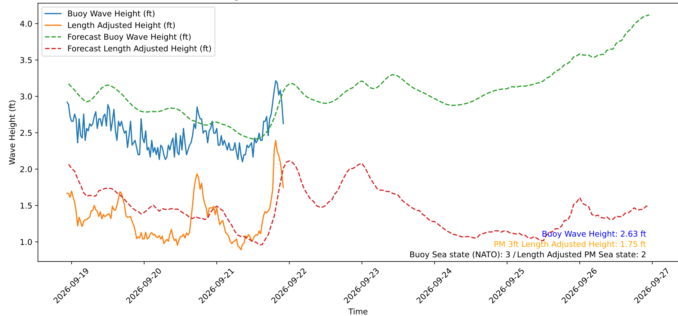
Wave Heights over Time for Oceanside Harbor at 2026-09-21 22:40:29
