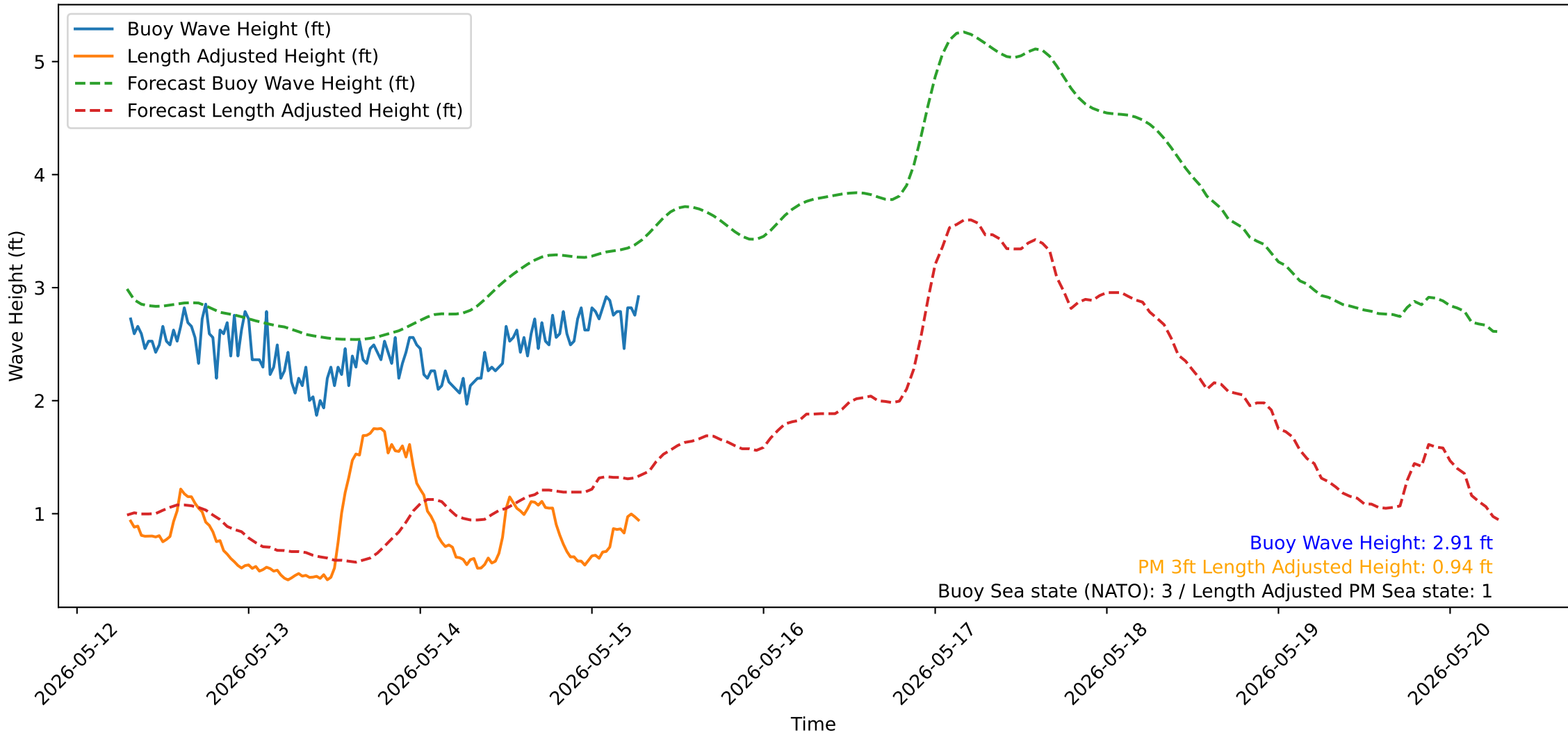
Wave Heights over Time for Red Beach at 2026-05-15 07:10:51
