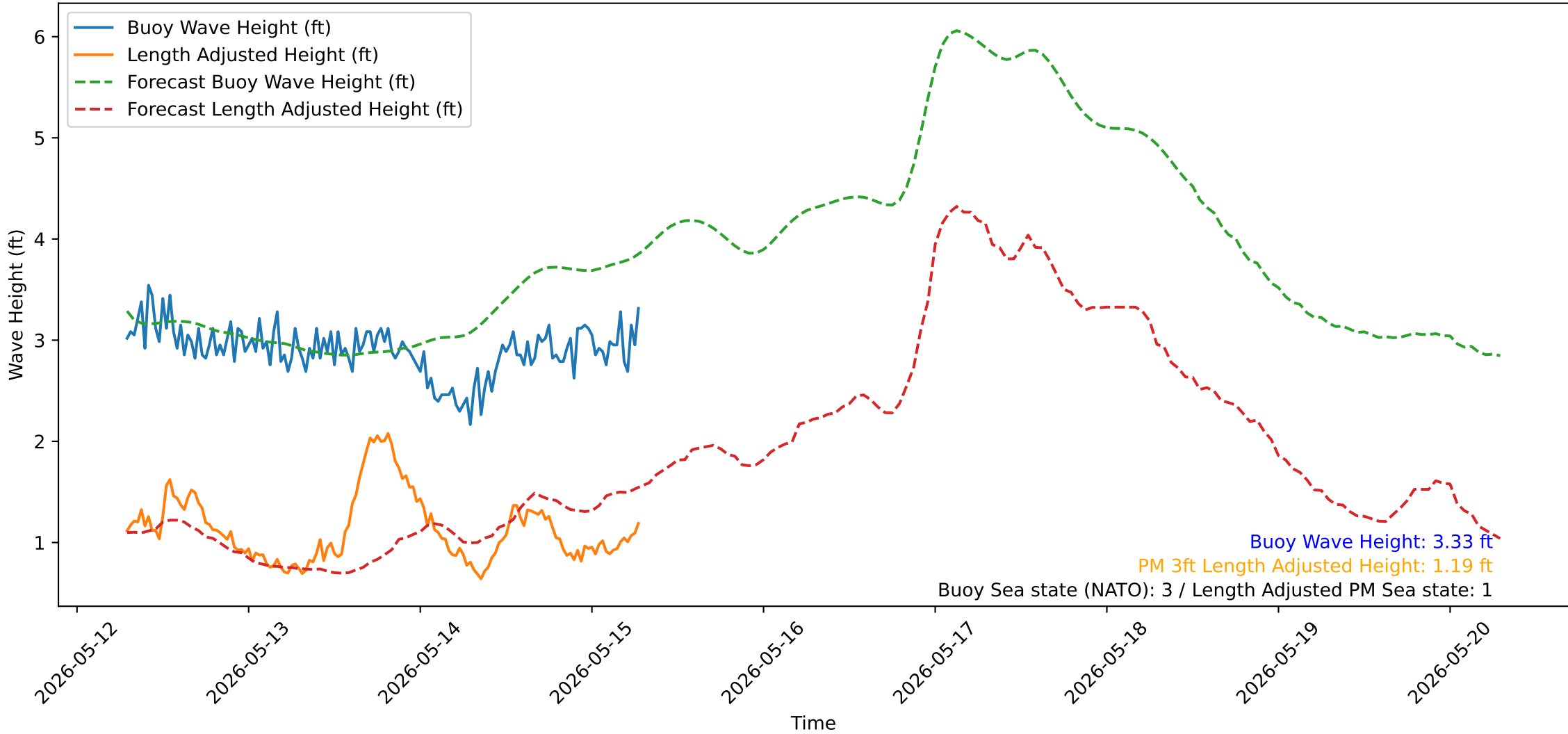
Wave Heights over Time for Oceanside Harbor at 2026-05-15 07:10:32
