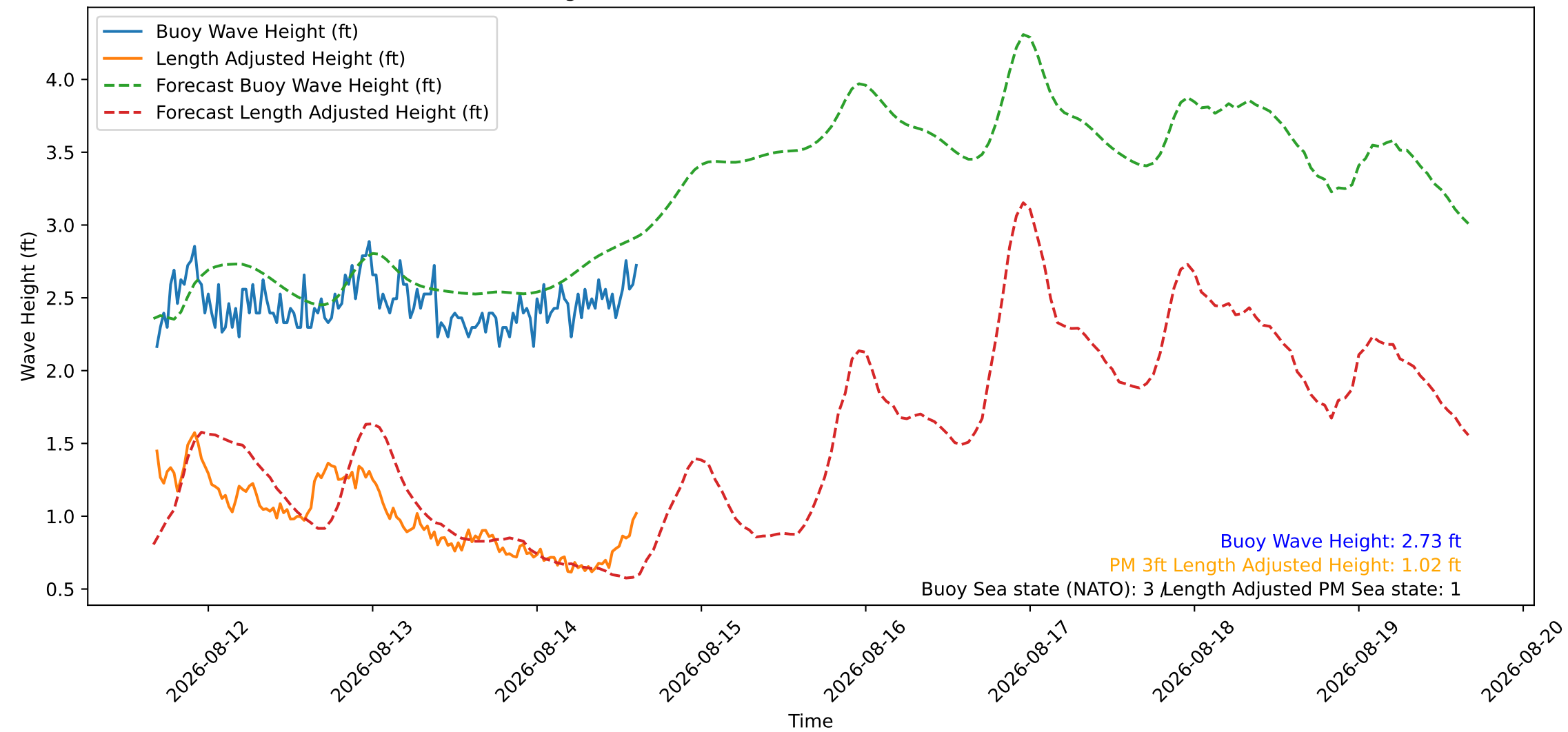
Wave Heights over Time for Red Beach at 2026-08-14 16:00:45
