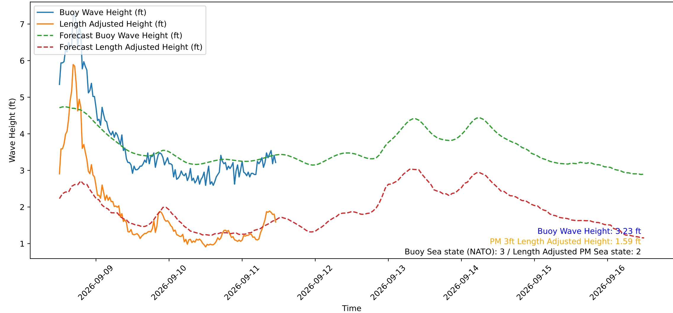
Wave Heights over Time for Green Beach at 2026-09-11 11:51:14
