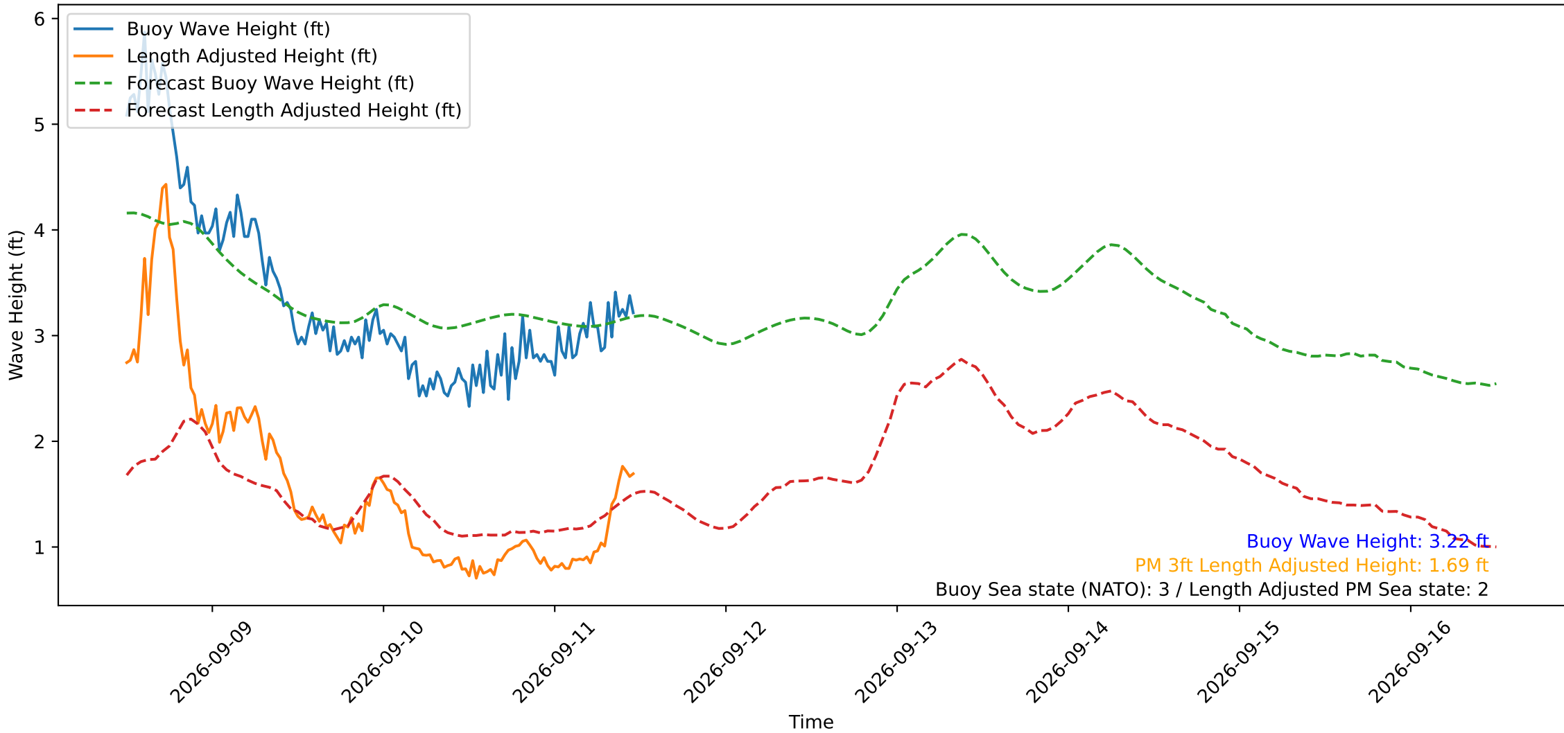
Wave Heights over Time for Red Beach at 2026-09-11 11:50:50
