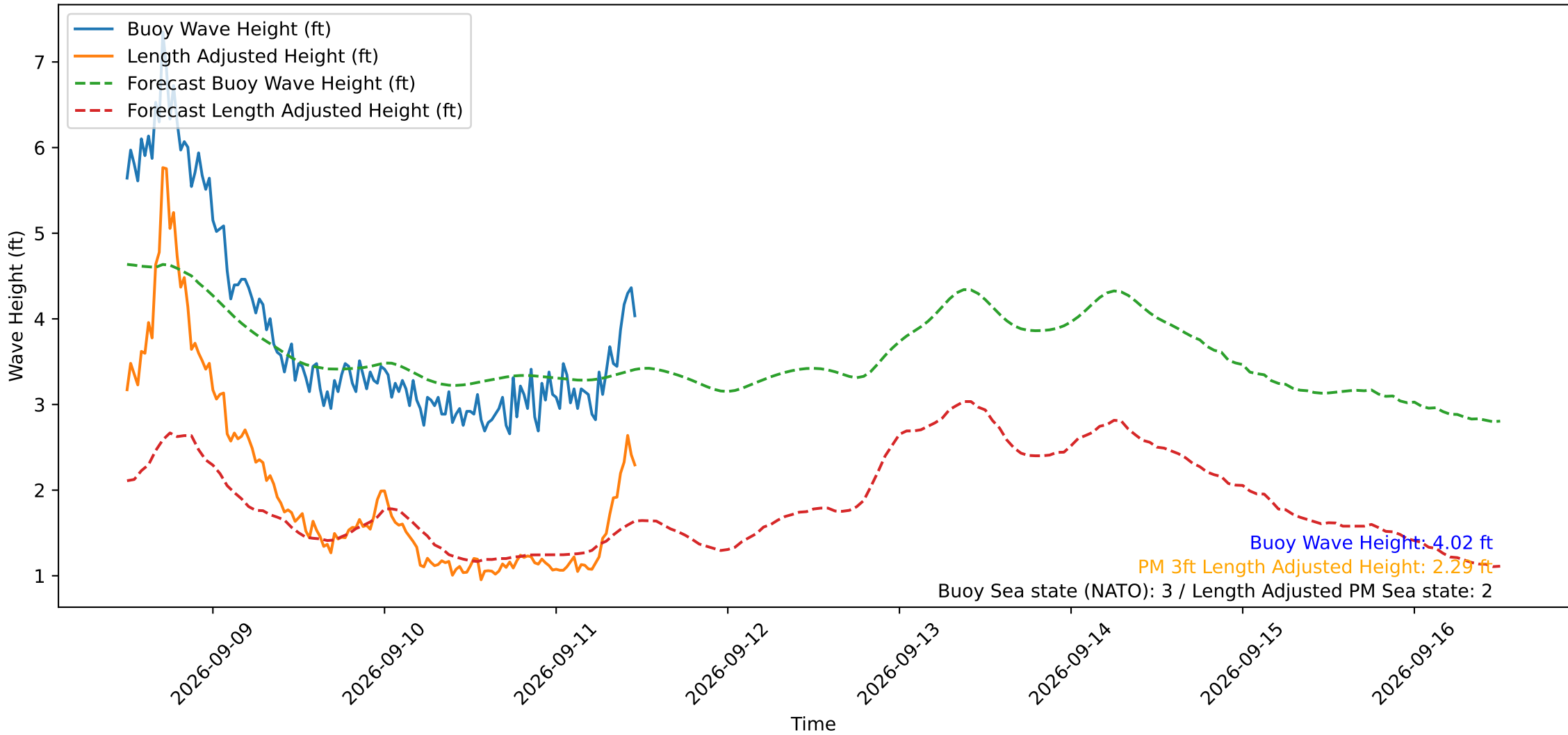
Wave Heights over Time for Oceanside Harbor at 2026-09-11 11:50:30
