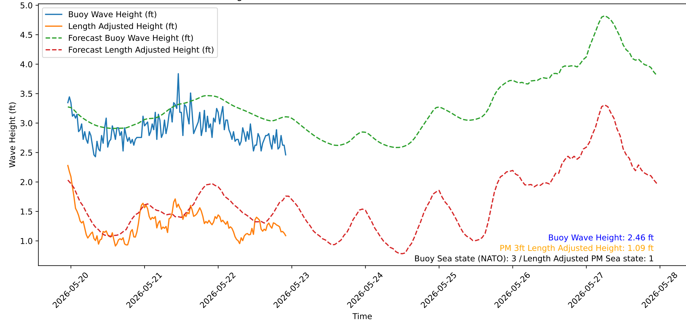
Wave Heights over Time for Oceanside Harbor at 2026-05-22 22:50:31
