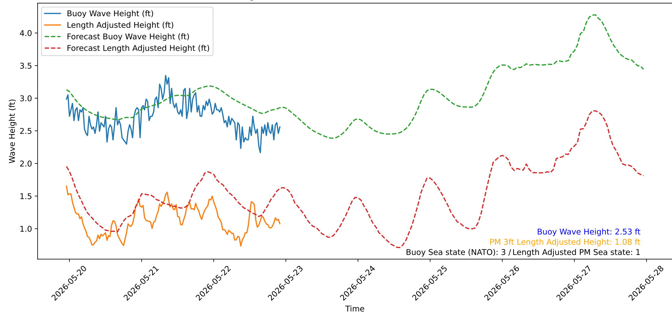
Wave Heights over Time for Red Beach at 2026-05-22 22:50:52
