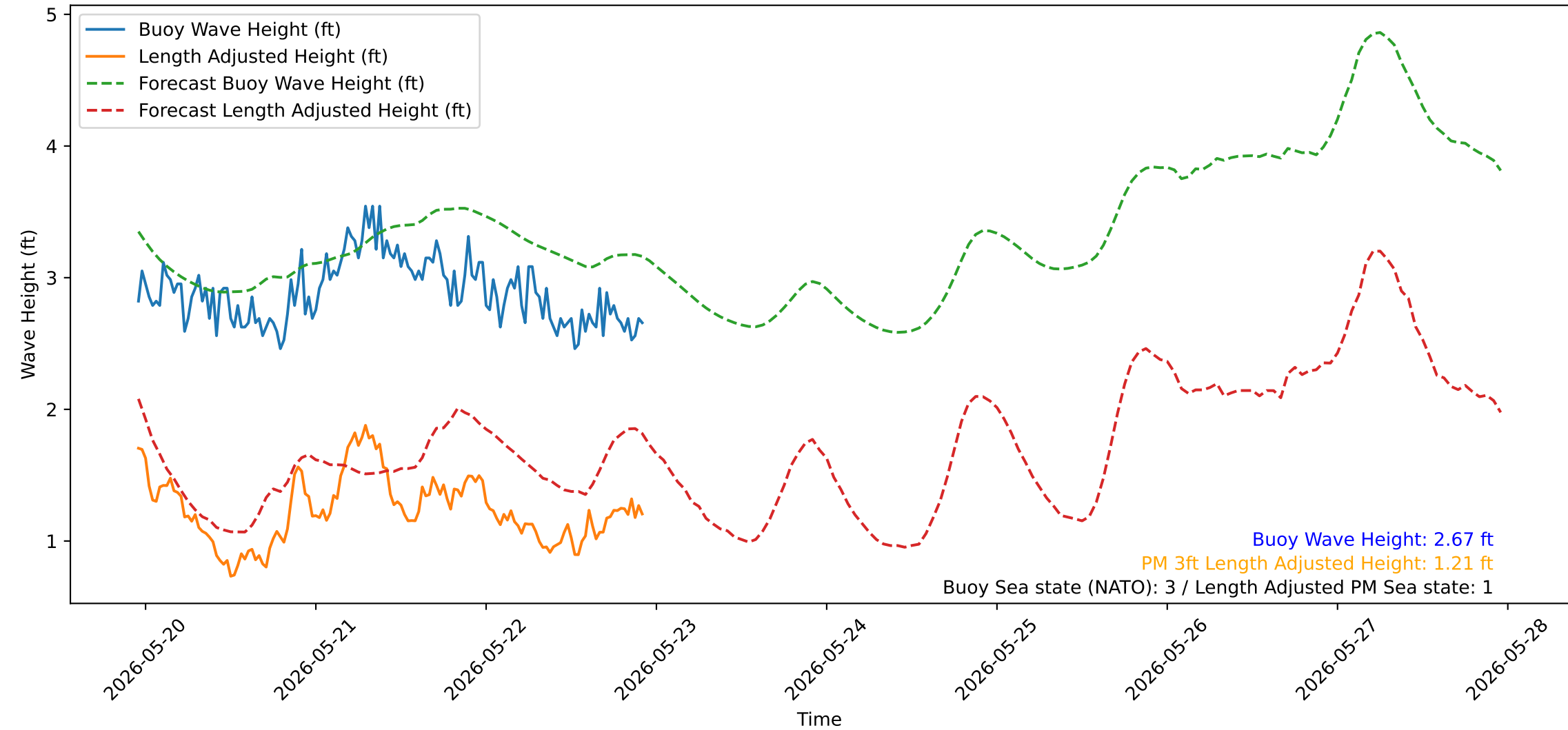
Wave Heights over Time for Green Beach at 2026-05-22 22:51:15
