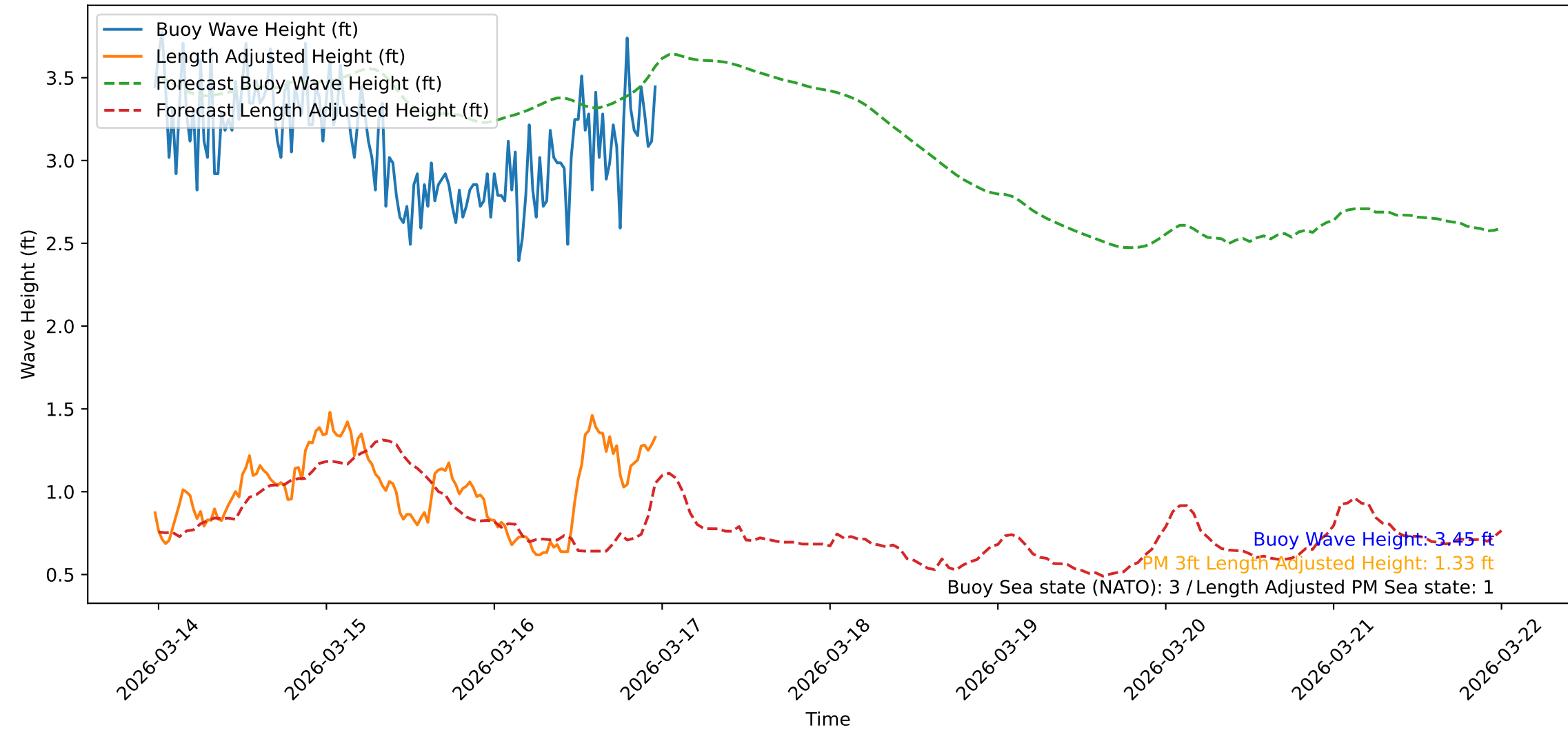
Wave Heights over Time for Oceanside Harbor at 2026-03-16 23:40:47
