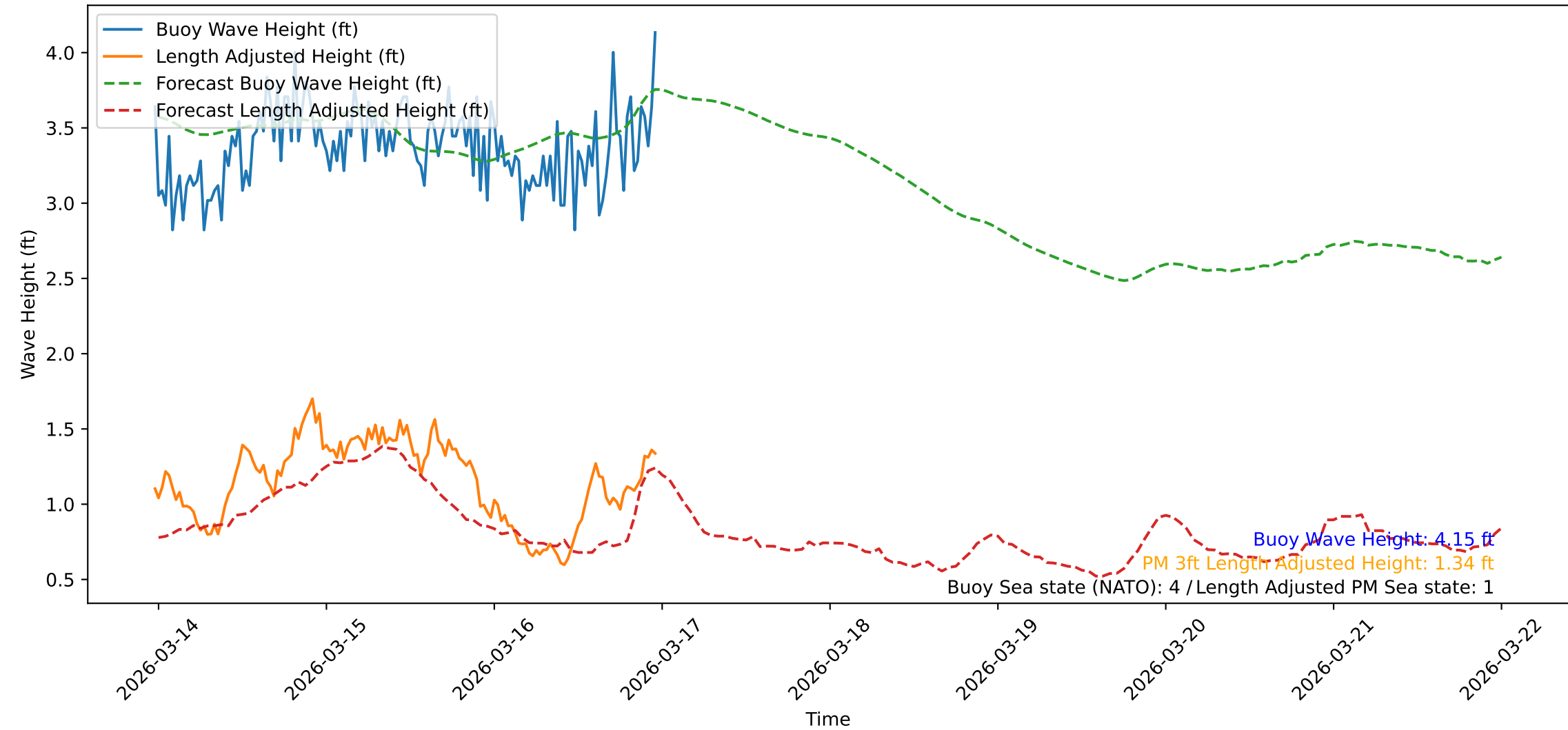
Wave Heights over Time for Green Beach at 2026-03-16 23:41:51
