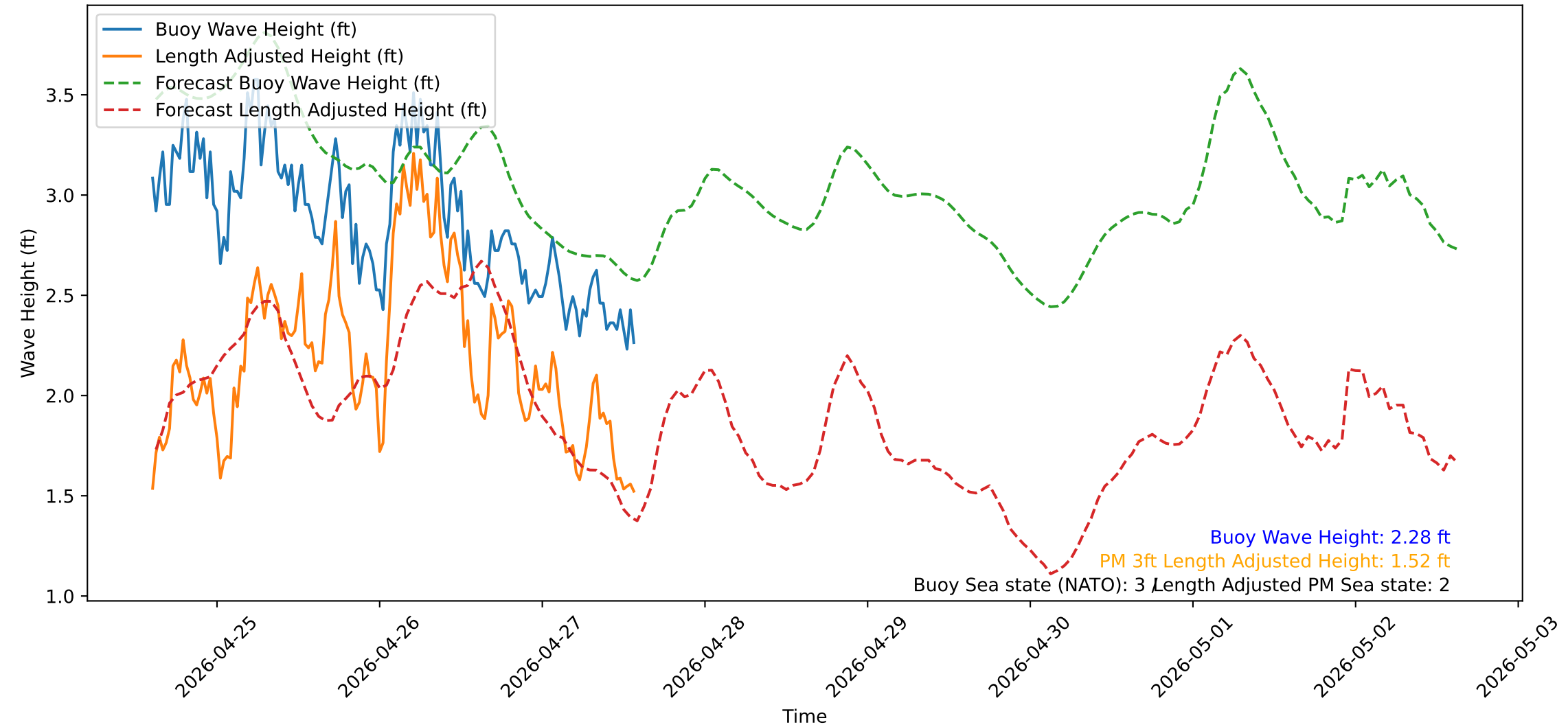
Wave Heights over Time for Green Beach at 2026-04-27 14:31:12
