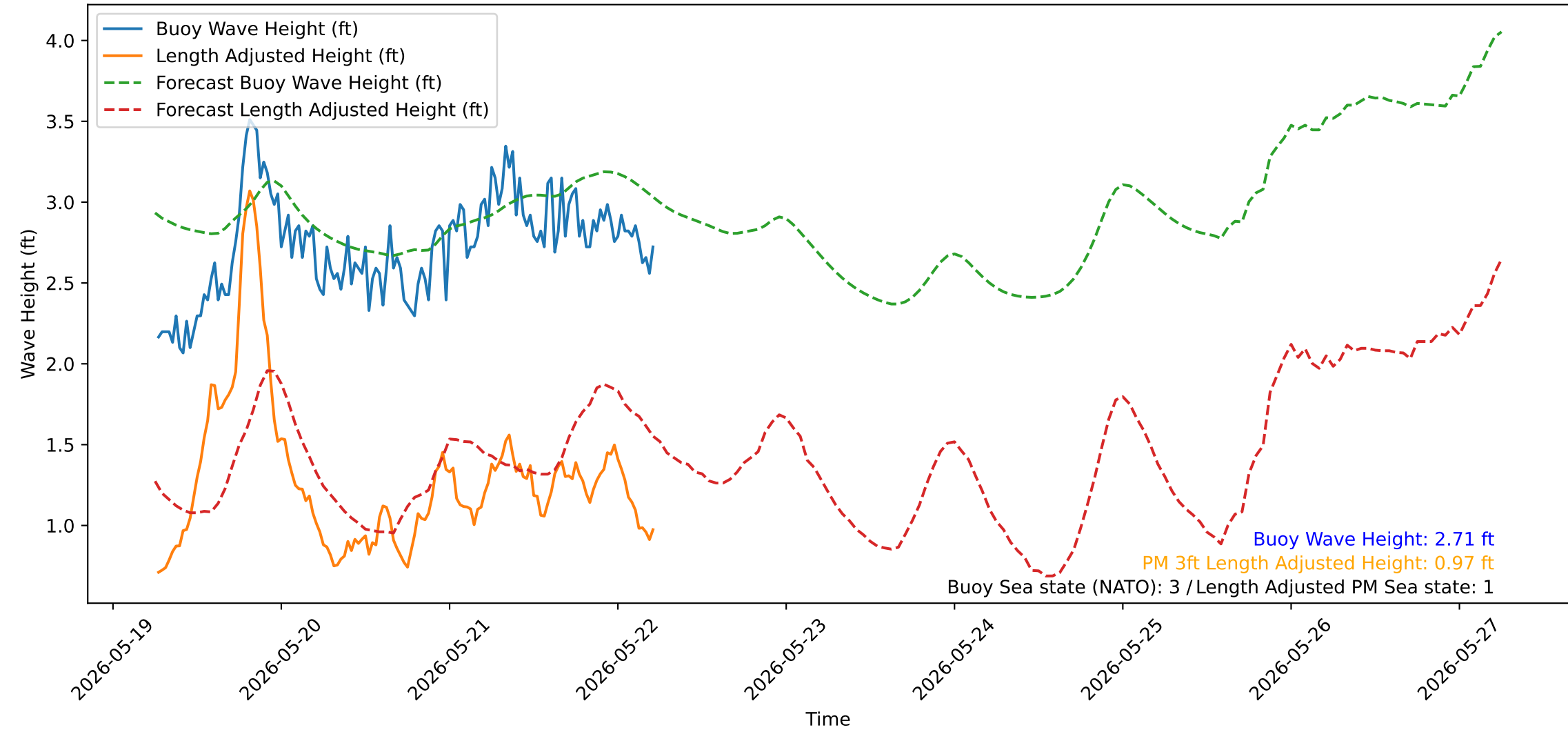
Wave Heights over Time for Red Beach at 2026-05-22 06:00:52
