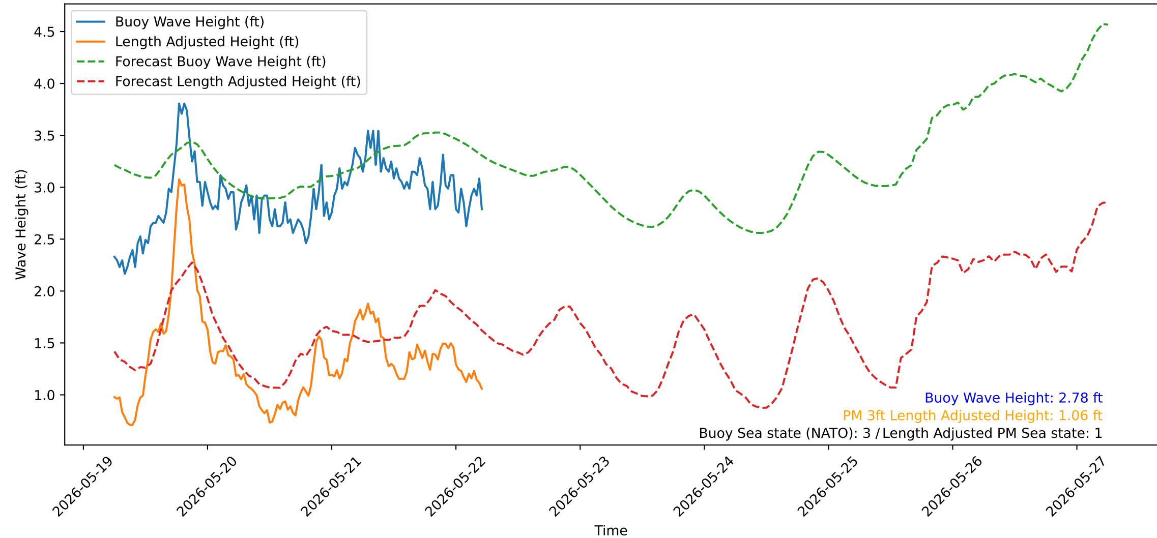
Wave Heights over Time for Green Beach at 2026-05-22 06:01:14
