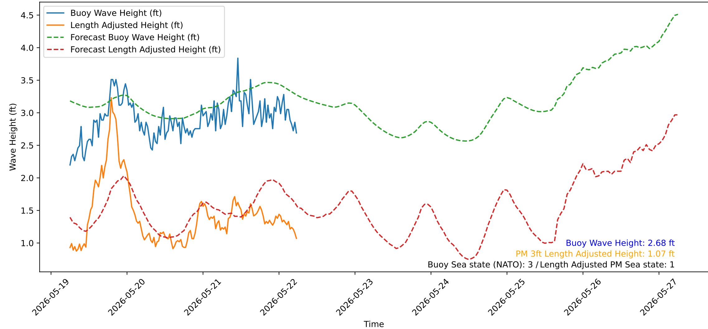
Wave Heights over Time for Oceanside Harbor at 2026-05-22 06:00:32
