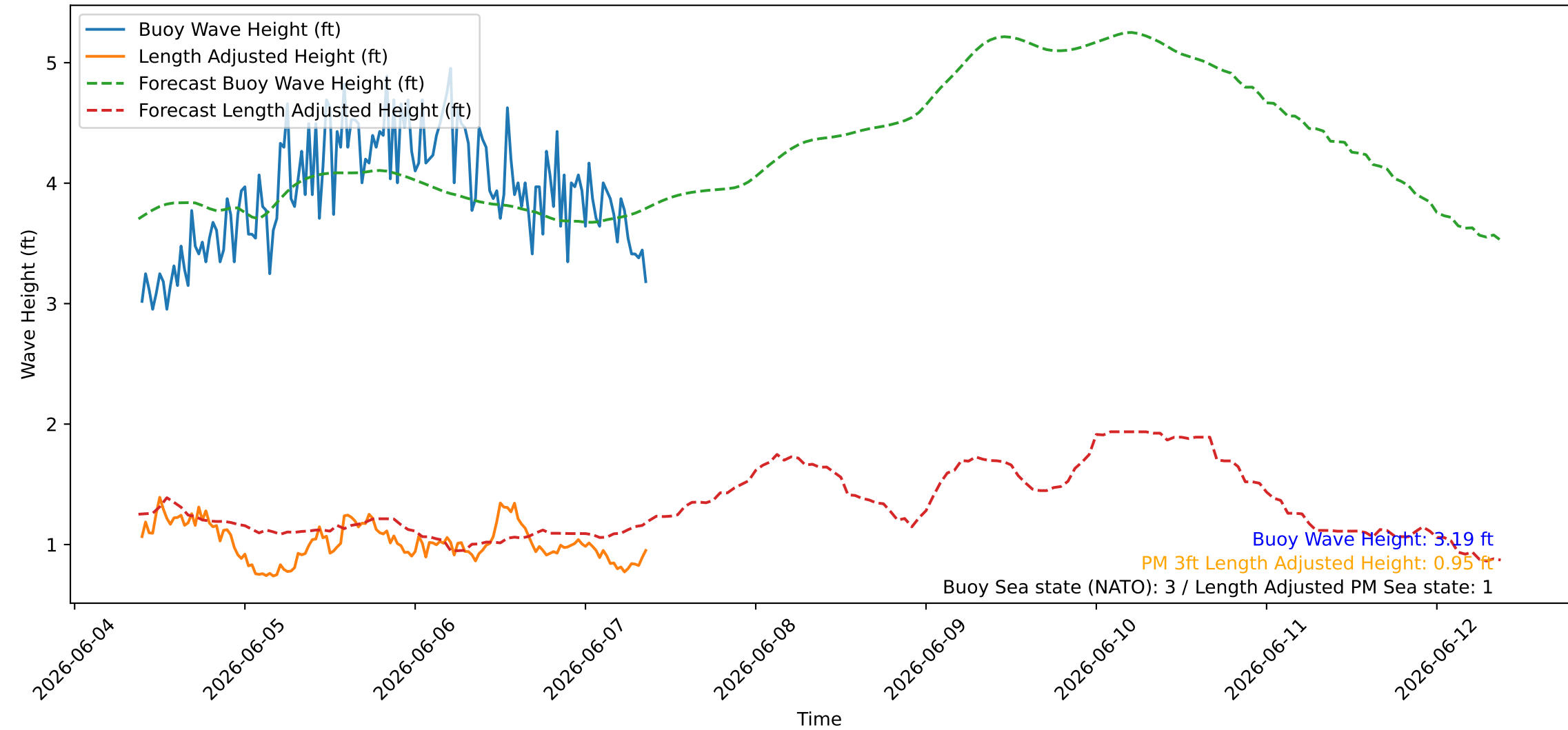
Wave Heights over Time for Red Beach at 2026-06-07 09:10:45
