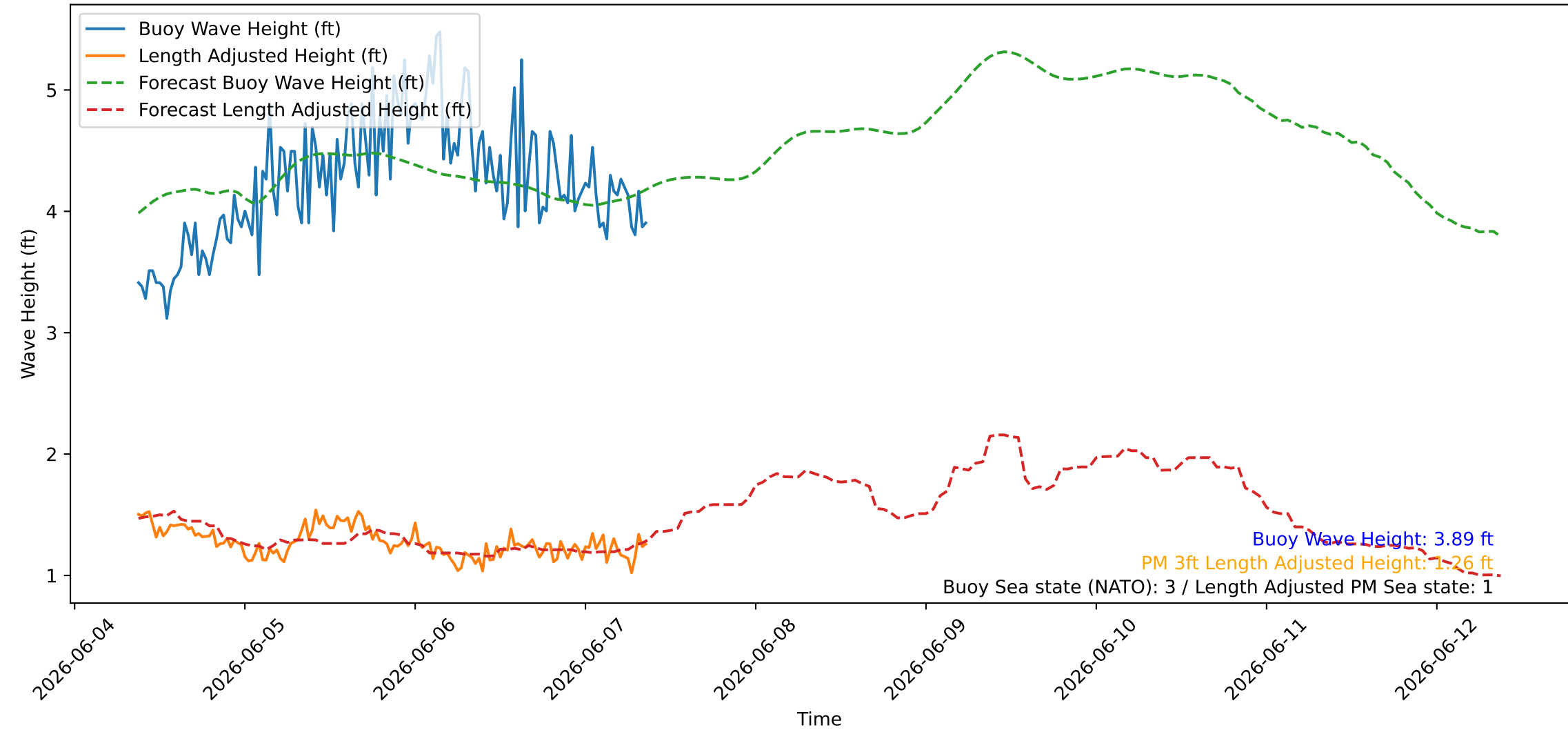
Wave Heights over Time for Oceanside Harbor at 2026-06-07 09:10:26
