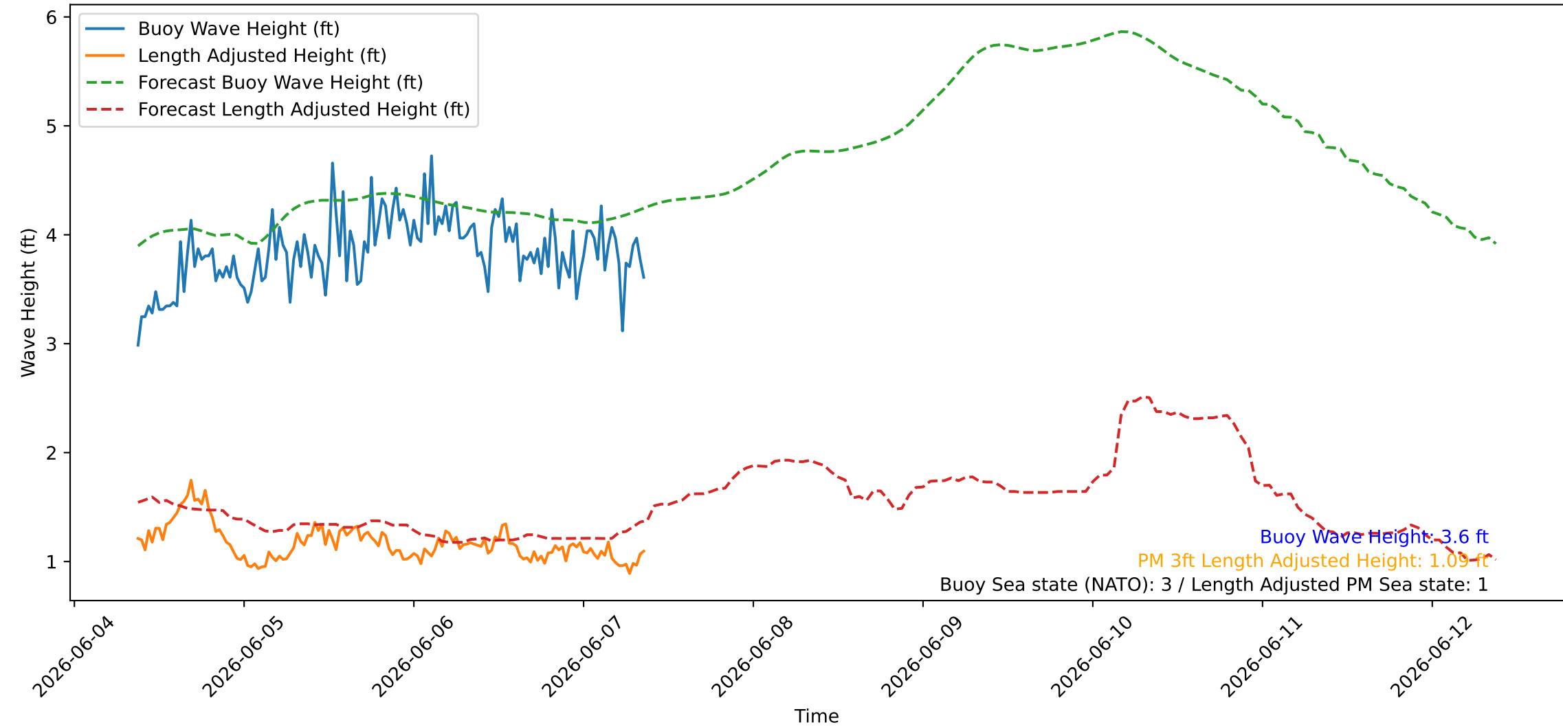
Wave Heights over Time for Green Beach at 2026-06-07 09:11:08
